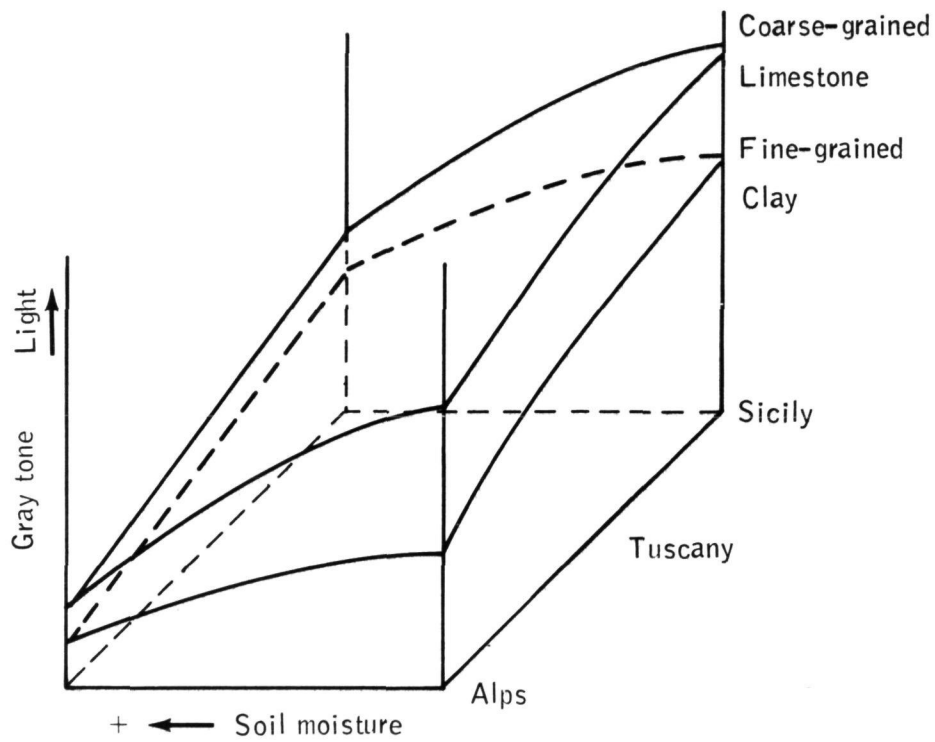
Figure 4. - Gray tone levels of grass; schematic representation for the factors of soil type, soil moisture, and climatic zone.
