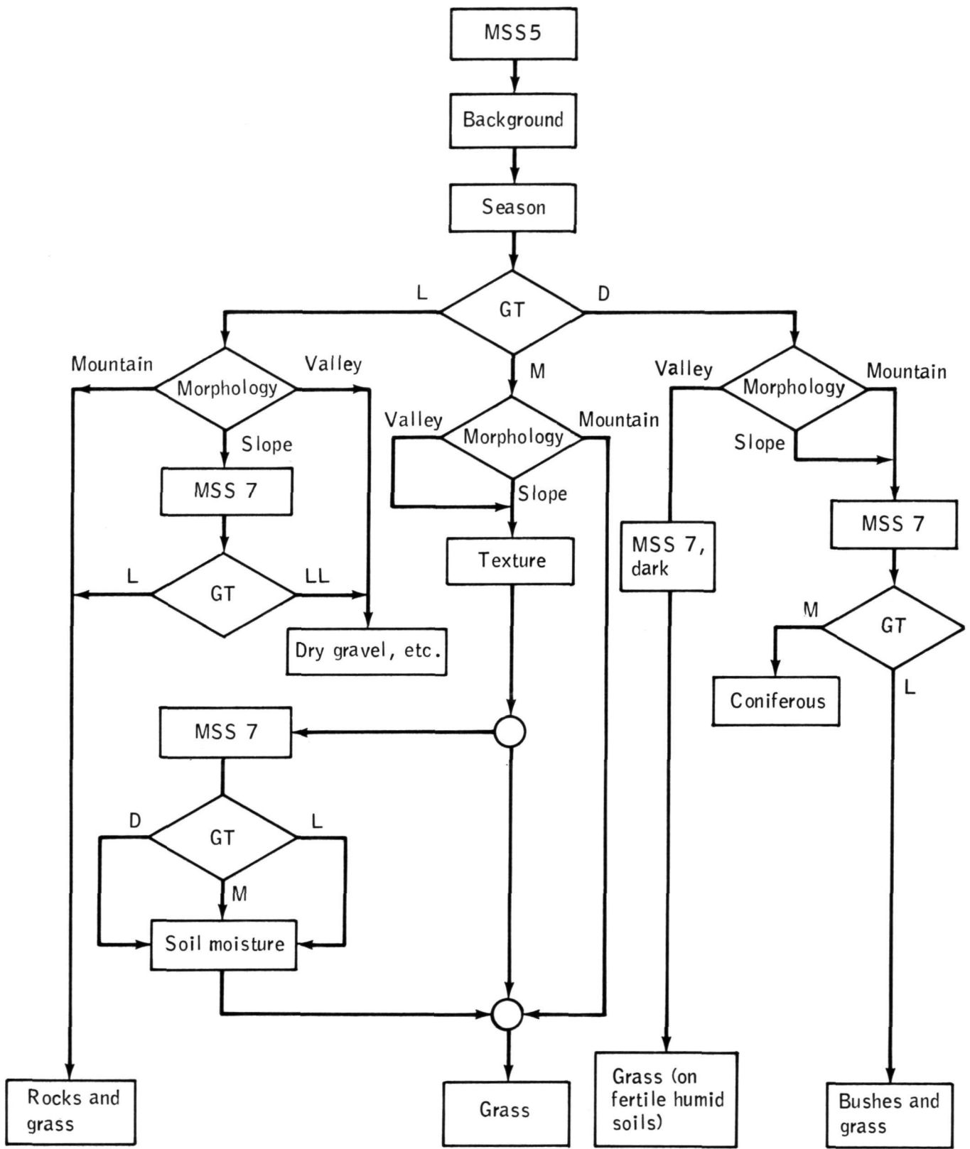
Figure 3. - Identification of grassland: schematic diagram for the interpretation of LANDSAT MSS data (GT = gray tone, L = light, LL = very light, M = medium, D = dark).
