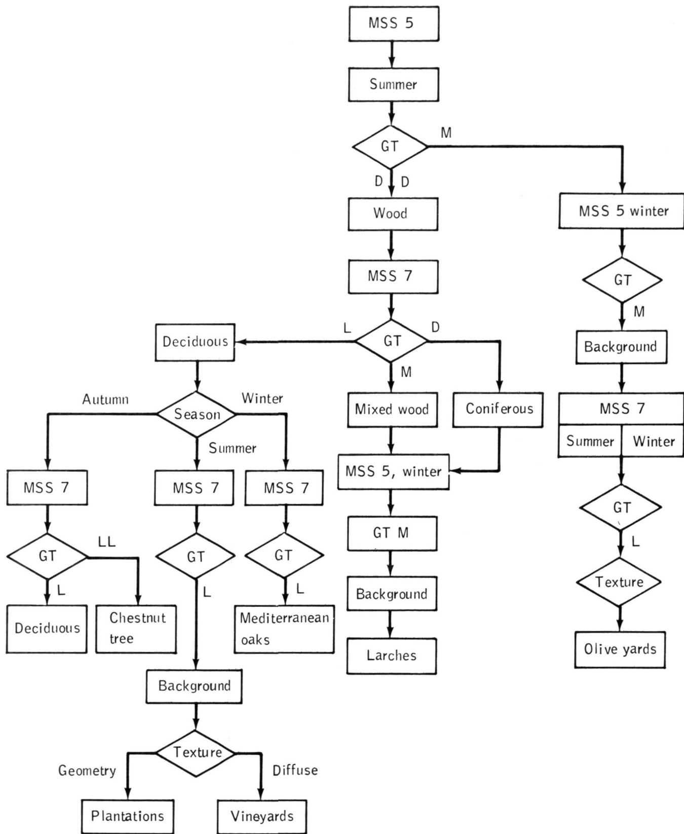
Figure 5. - Identification of wooded areas; schematic diagram for the interpretation of LANDSAT MSS data (GT = gray tone, L = light, LL = very light, M = medium, D = dark, DD = very dark).
