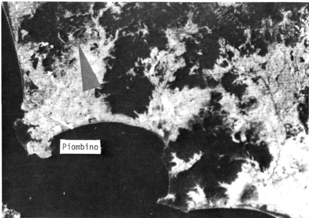
Figure 8. - Lower valley of the Cornia River, east of Piombino (detail from LANDSAT image of 12 Aug. 1972; MSS 5) (dark = woods, middle gray = olive yards (arrow)).
