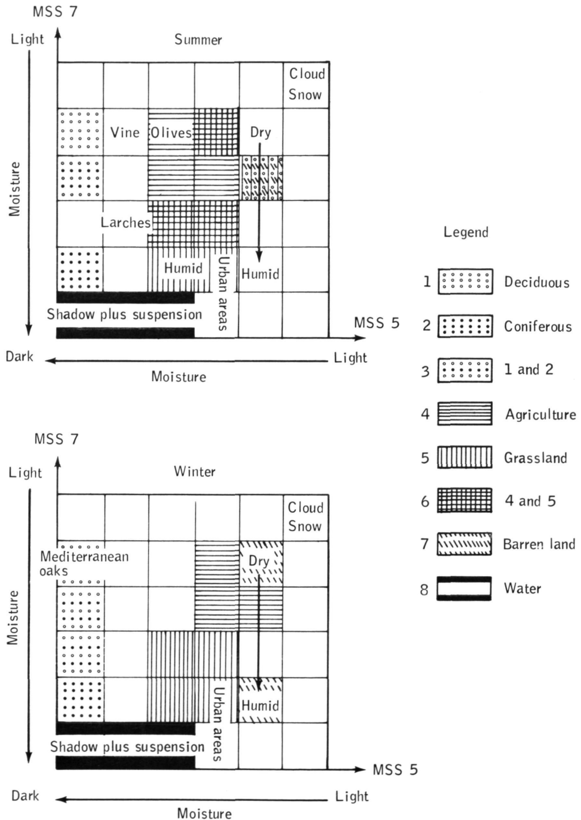
Figure 2. - Schematic position of land use categories in a coordinate system based on the gray tone in LANDSAT images of MSS 5 and 7.
