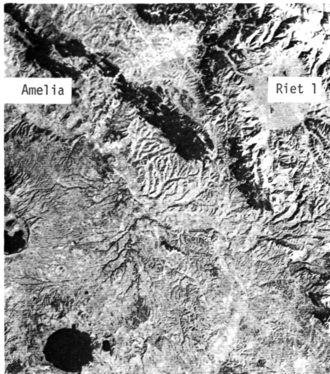
Figure 7(a). - Mountain ranges west of Rieti (detail from LANDSAT image of 6 Feb. 1973; MSS 5) (dark = evergreen, mediterranean oaks).
