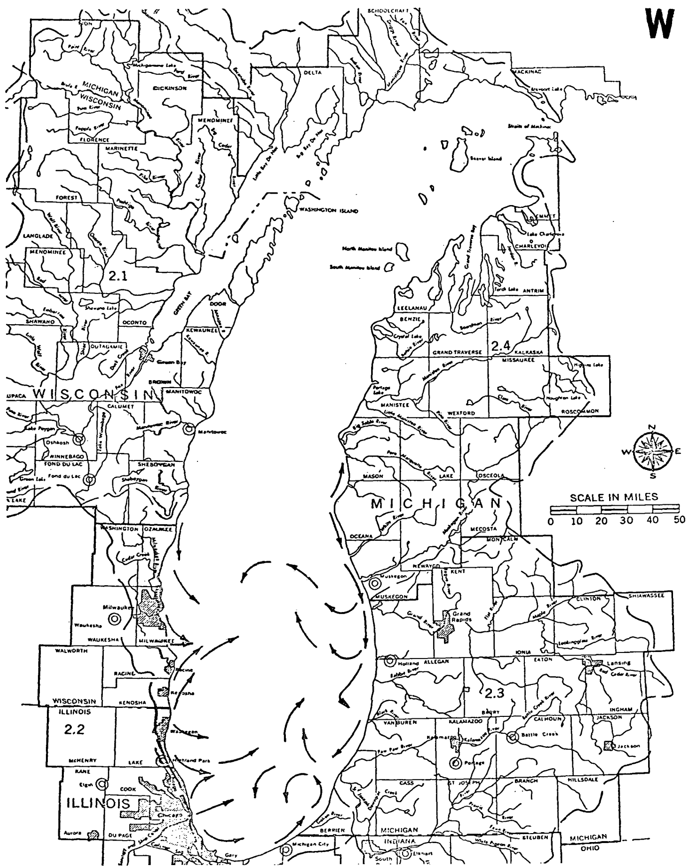
Figure 8. Surface current analysis as determined from turbidity patterns in LANDSAT-1 scenes. Weighted wind direction (Westerly) indicated in upper right-hand corner.
