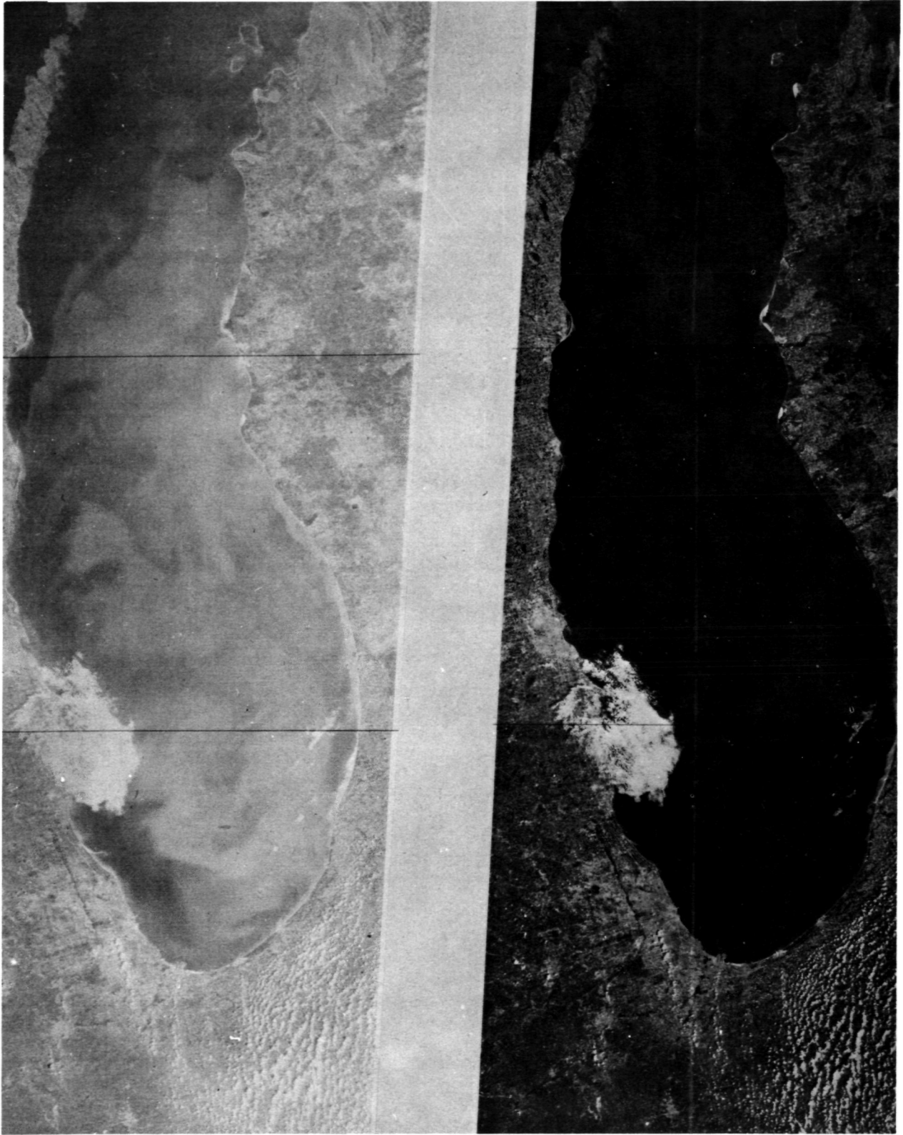
Figure 10. LANDSAT-1 images (MSS-4, left and MSS-5, right) obtained 3 August 1973, showing the extent of the calcium carbonate precipitation over southern Lake Michigan.
