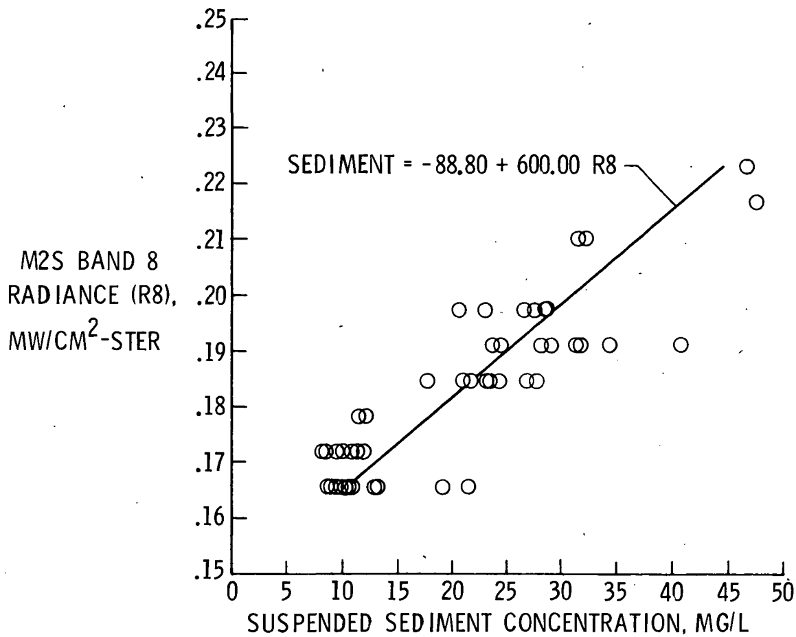
Figure 4. Suspended sediment concentrations, M2S Band 8 radiances and fitted single band regression line.
