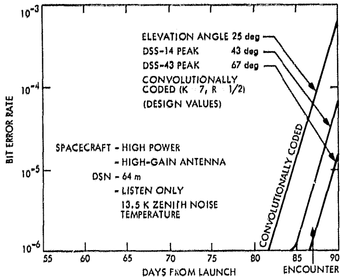
Figure 3. Mariner Encke 1980 117.6-kbps telemetry error rate vs days from launch
