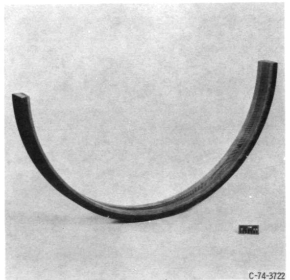
Figure 6. - Circumferential grooves.
