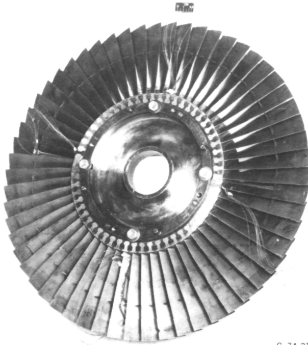
(a) Rotor.
