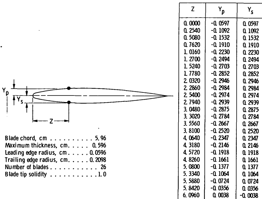
Figure 2 - Inlet guide vane.
