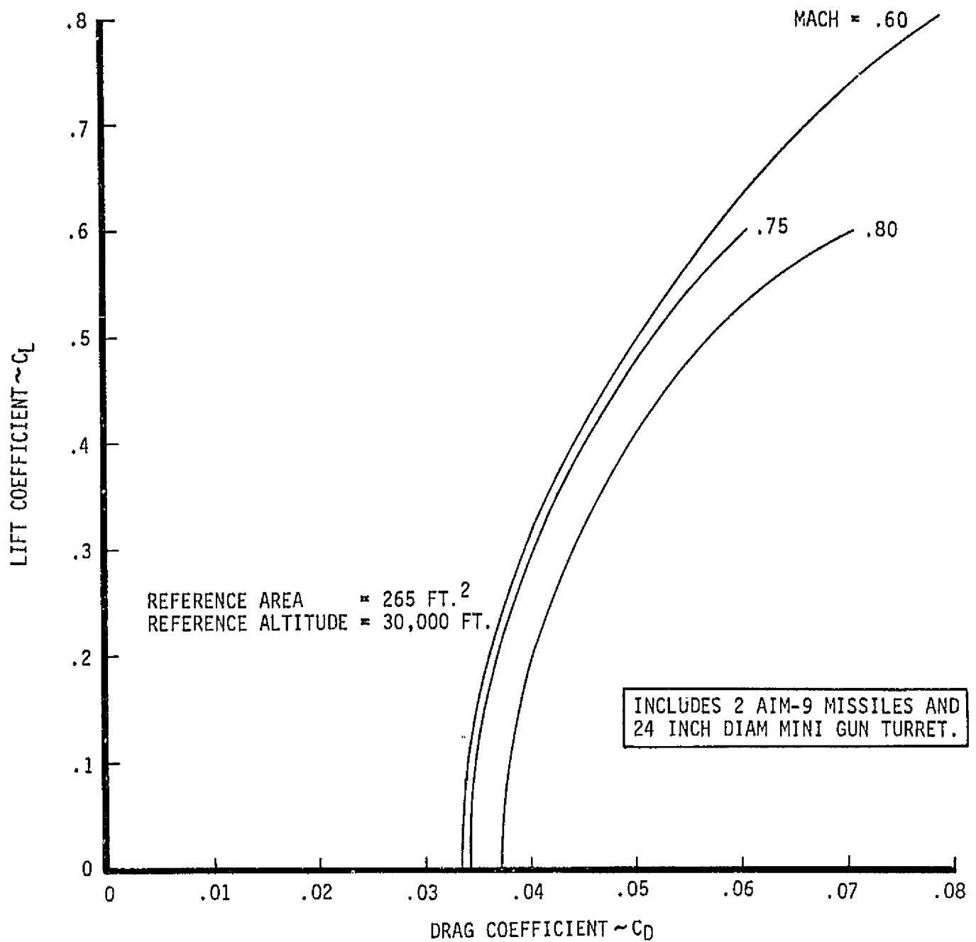
Figure 3.1-12.-Trimmed Drag Polar LCFA 1041-132 (CSAR)
