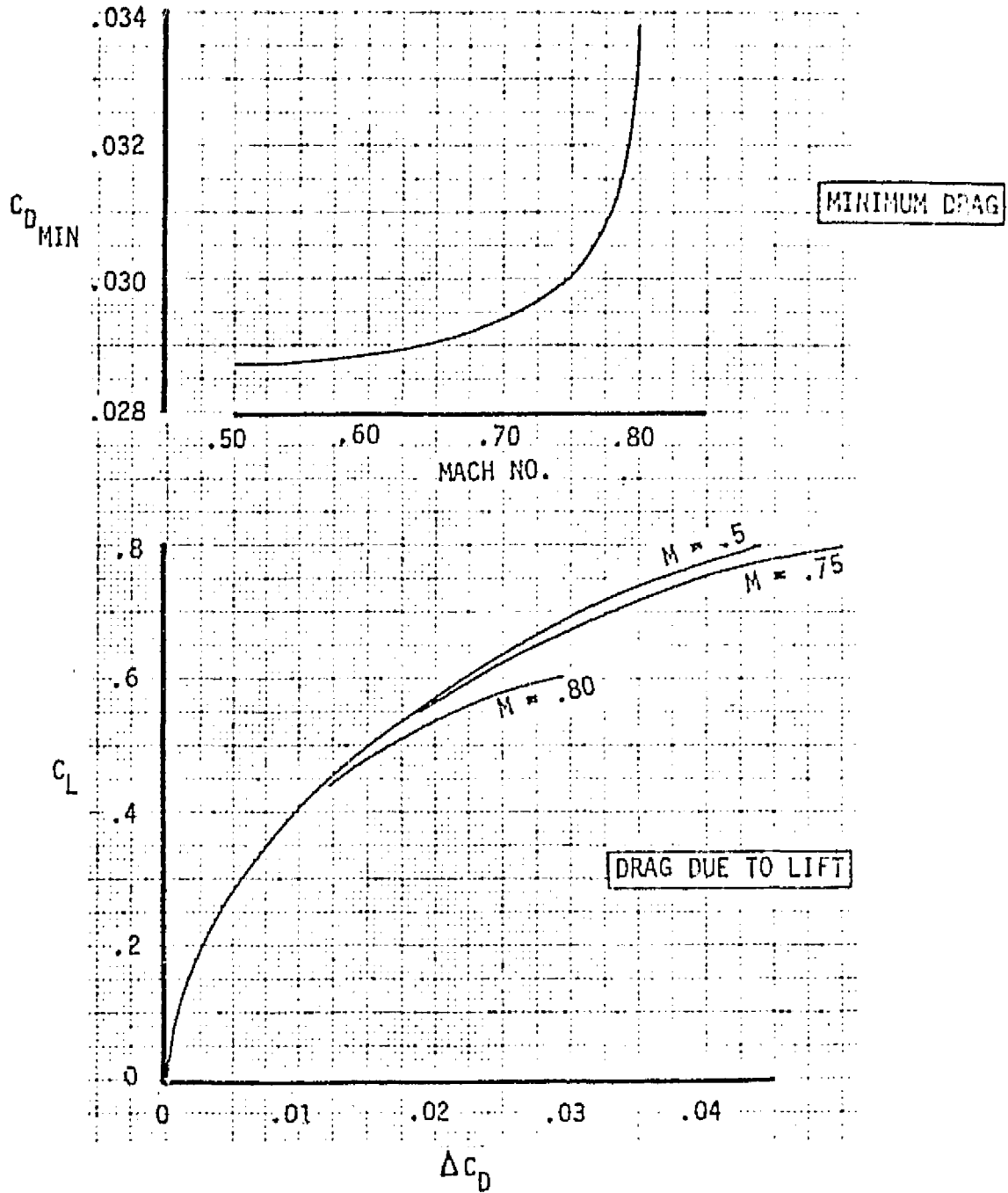
Figure 3.3.3-2.-Drag Breakdown 1041-133-1 (ASW)
