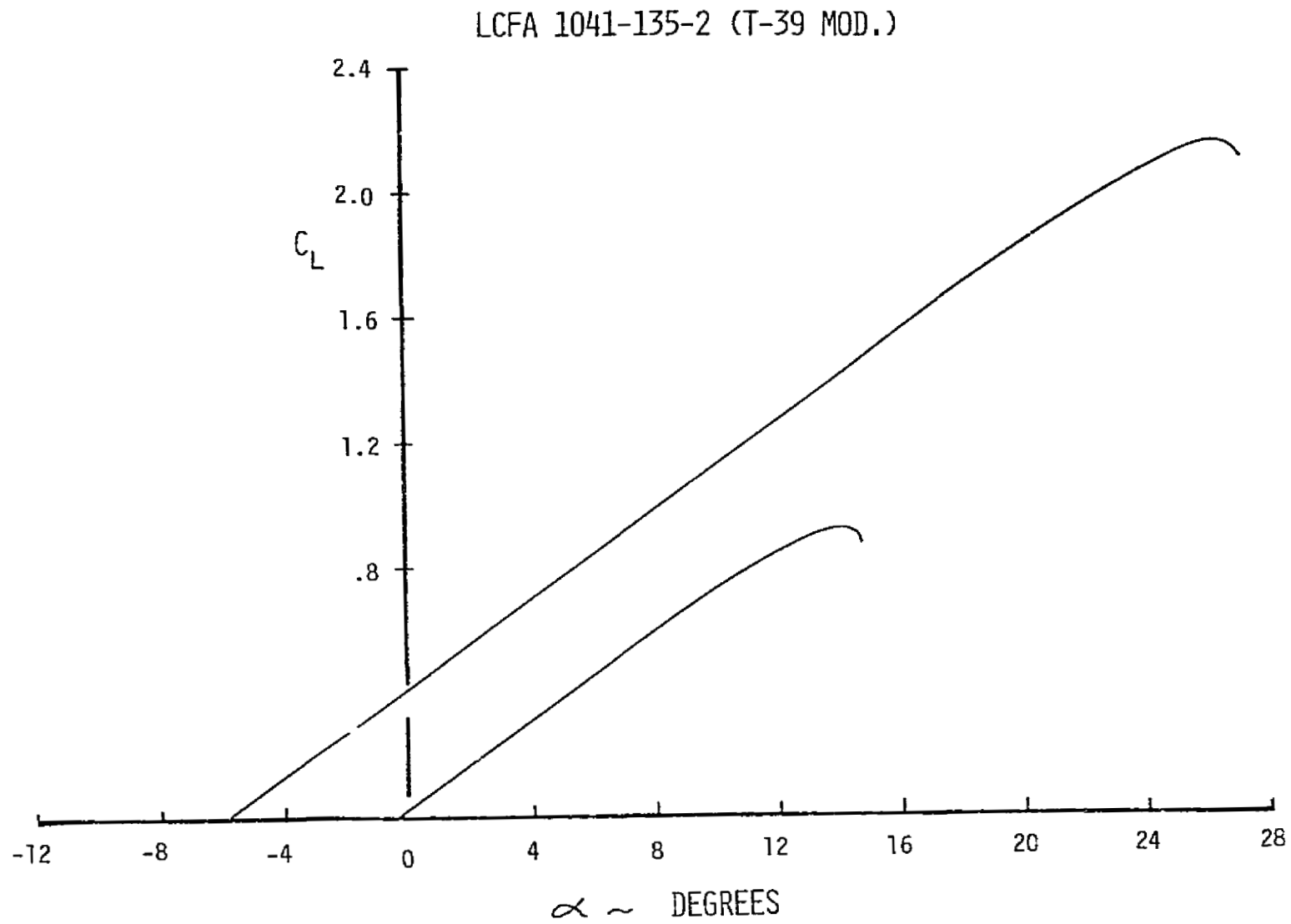
Figure 4-2-5.-Aerodynamic Lift Power Off
