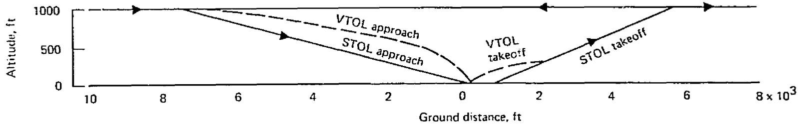
Figure 4.1.7-1.-LCFA Technology Airplanes, Typical Terminal Area Test Missions
