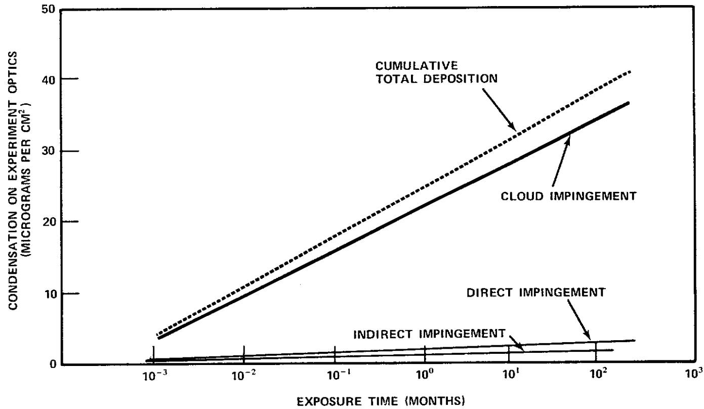
Figure C.2-1. - Condensible deposition versus time.
