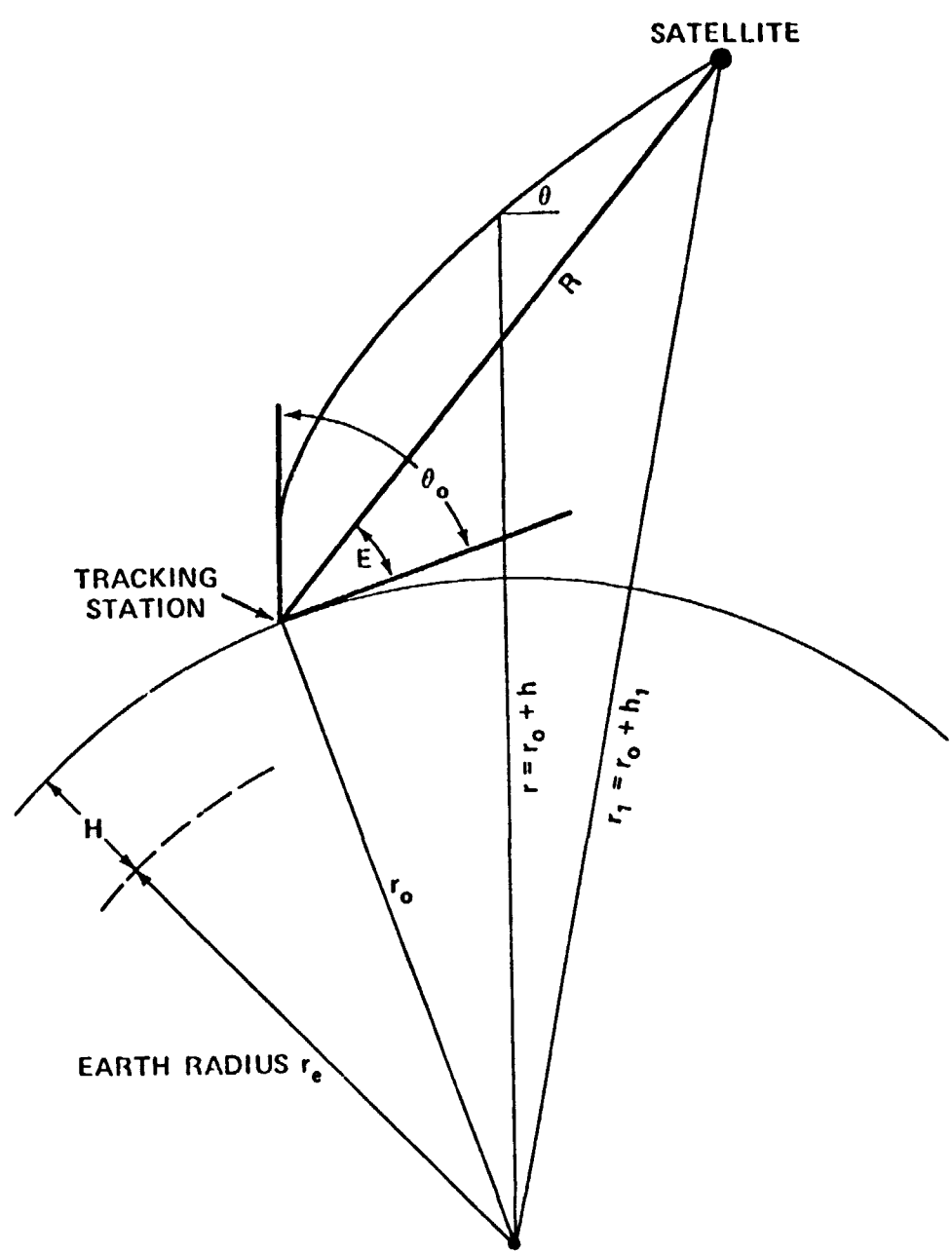
Figure 1. Geometry of laser ranging site and satellite target [3].
