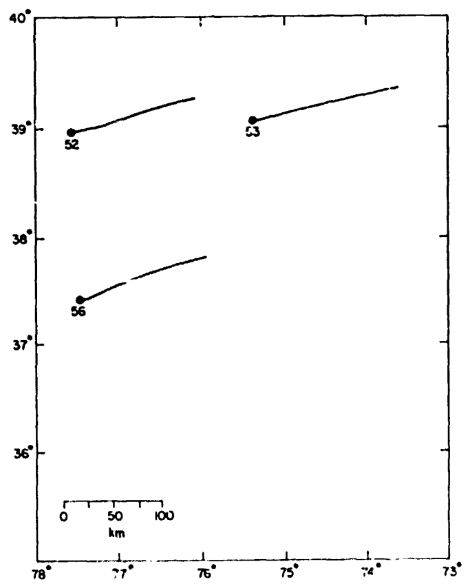
Figure 3. Balloon trajectories for sites 52, 53, and 56. Release time = 17.30. Release date = 2/13/70.
