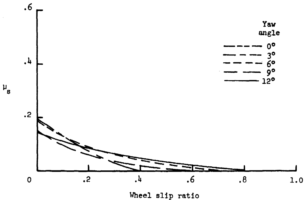
(a) Ground speed \approx 50 knots.
