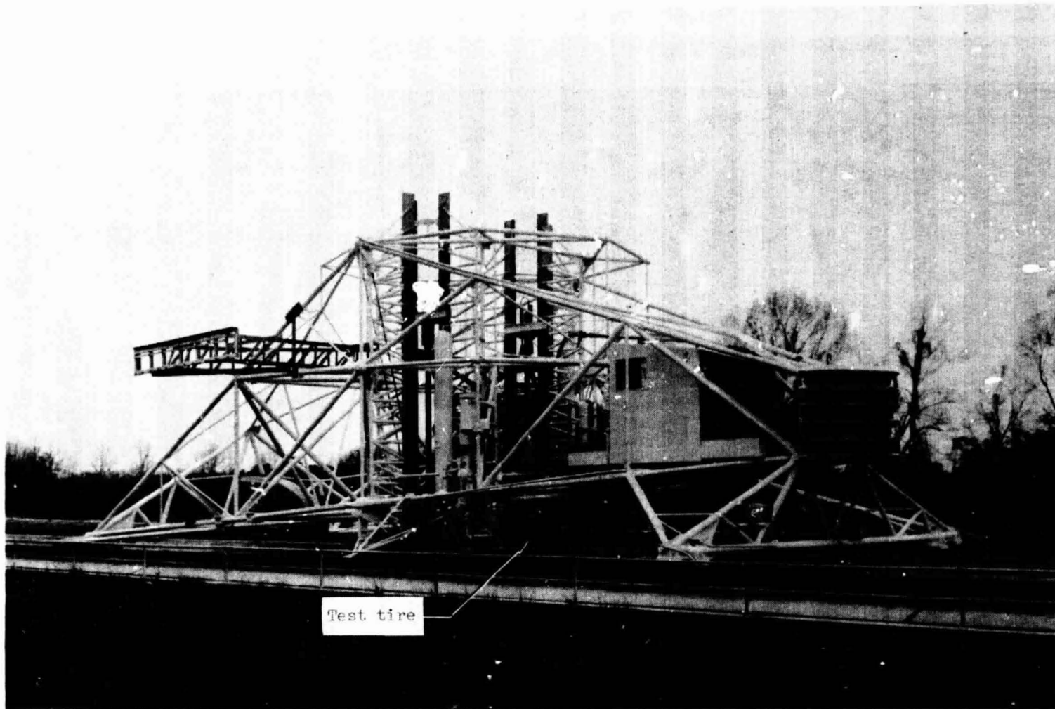
Figure 4.- Main test carriage at the Langley aircraft landing loads and traction facility.
