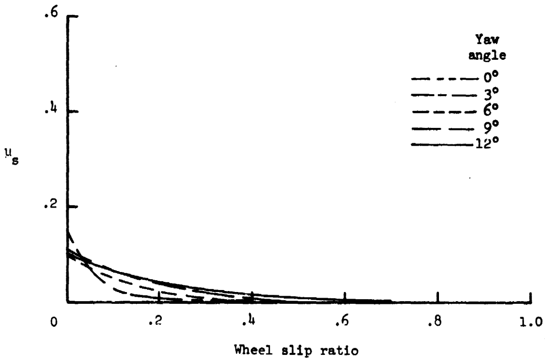
(b) Ground speed \approx 75 knots.
