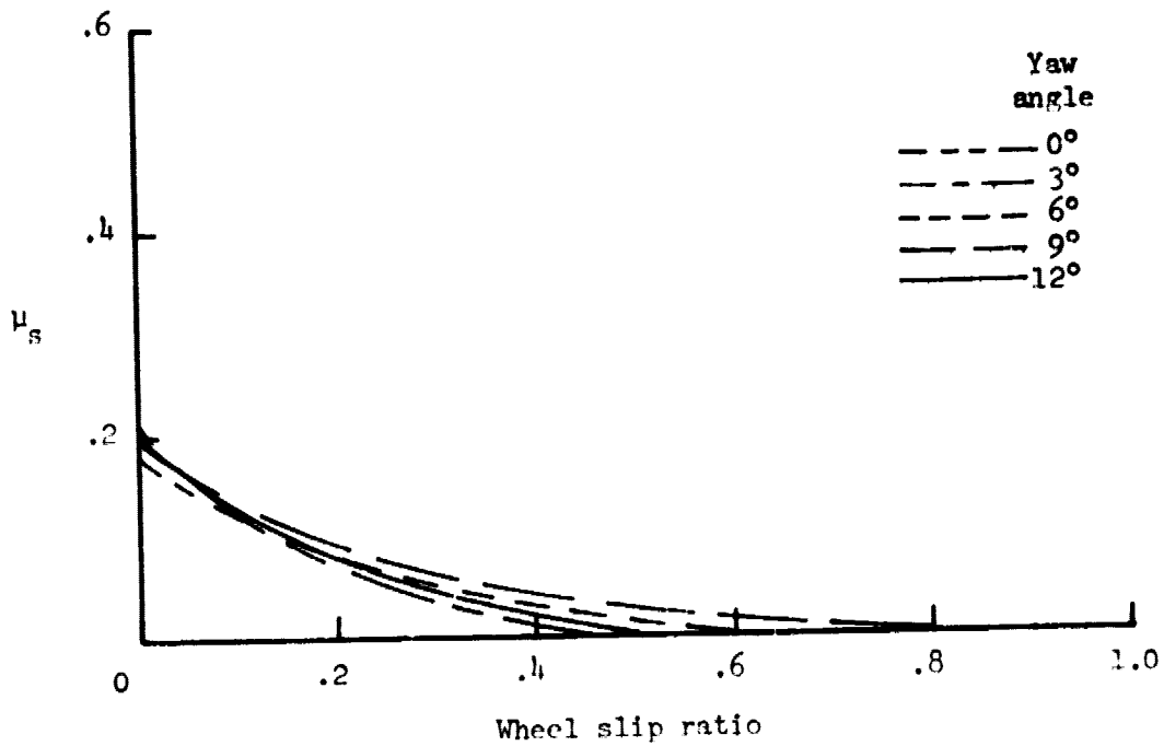
(a) Ground speed \approx 50 knots.
