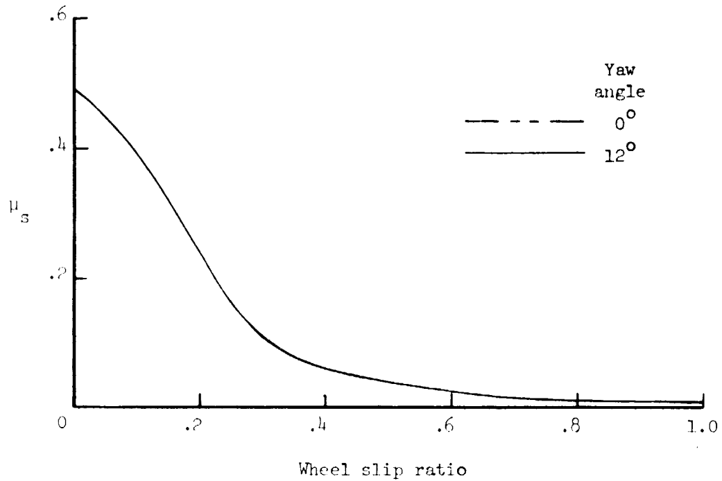
(c) Ground speed \approx 100 knots.
