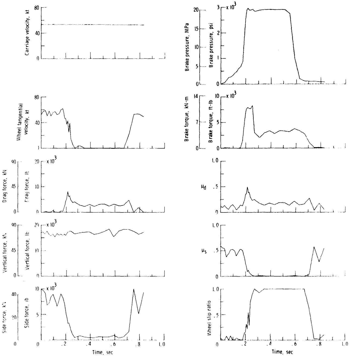
Figure 6. - Typical time histories of various parameters recorded and computed for test run brake cycles. Yaw angle = 12^\circ ; ground speed = 51 knots; dry concrete surface.
