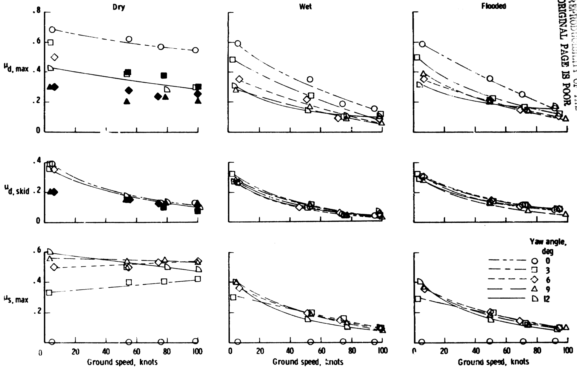
Figure II. - Variation of maximum drag-force friction coefficient \mu_{d, max} , skidding drag-force friction coefficient \mu_{d, skid} , and maximum cornering-force friction coefficient \mu_{s, max} with ground speed at various yaw angles on dry, wet, and flooded surfaces. (Closed symbols denote rubber contaminated surface)
