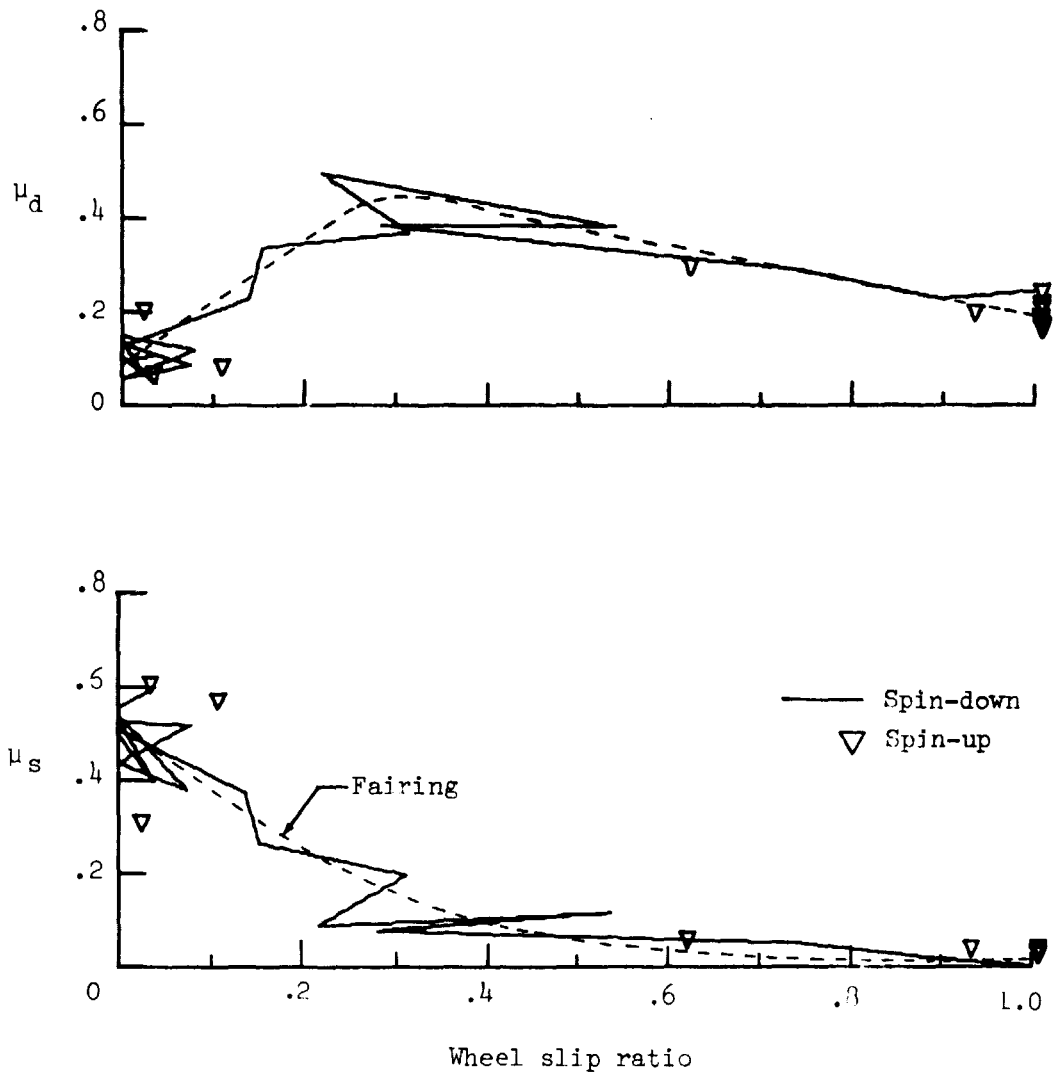
Figure 7.- Variation of computed friction coefficients with wheel slip ratio during a brake cycle on dry concrete surface.
