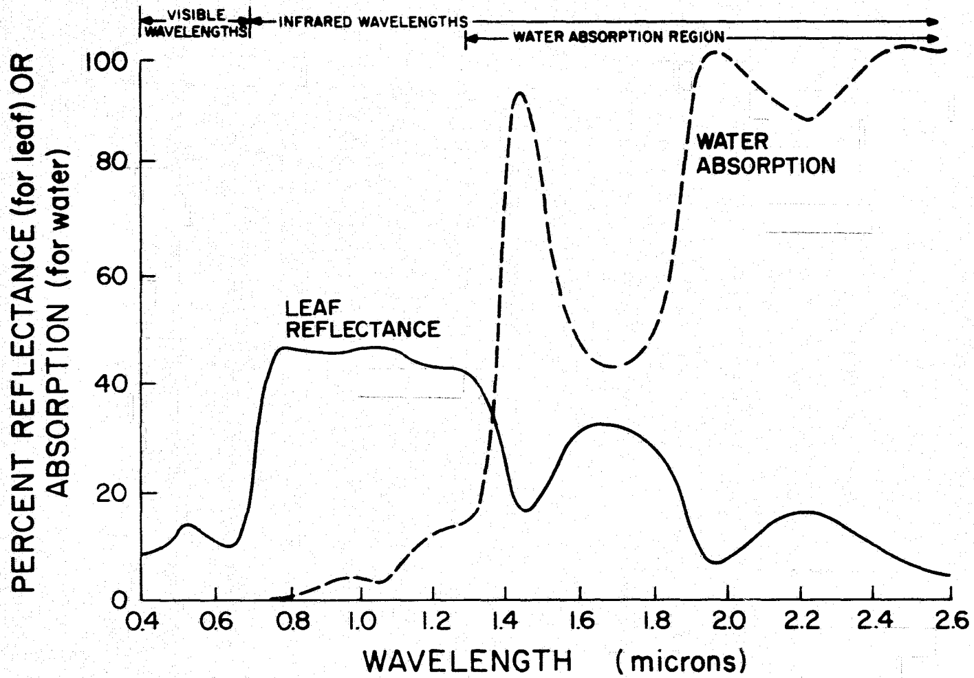
Fig. 3. Relationship between leaf reflectance and water absorption between 0.4 and 2.60 micron wavelengths (LARS, 1968)
