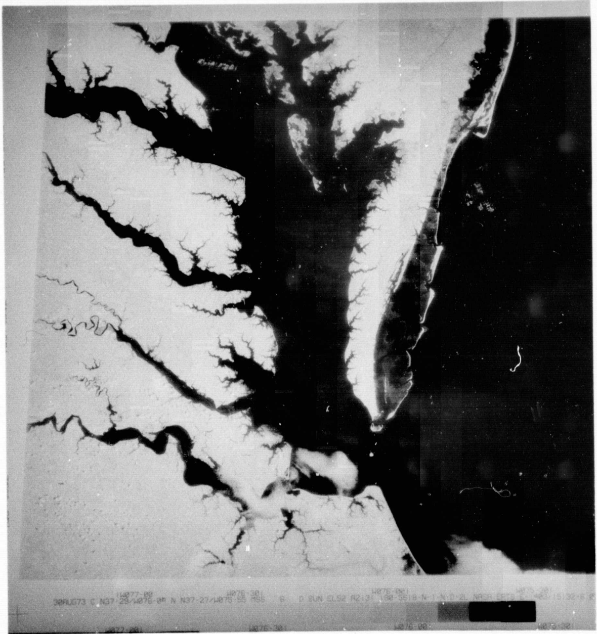
Fig. 6 c. Band 6 of LANDSAT-1 MSS image of August 30, 1973
