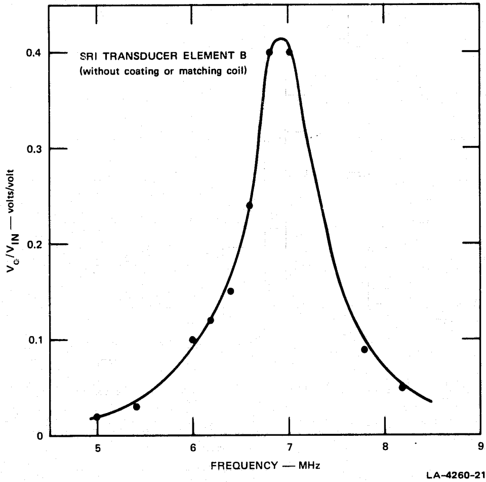
FIGURE C-2 ELEMENT-B TEST RESPONSE, SRI TRANSDUCER
