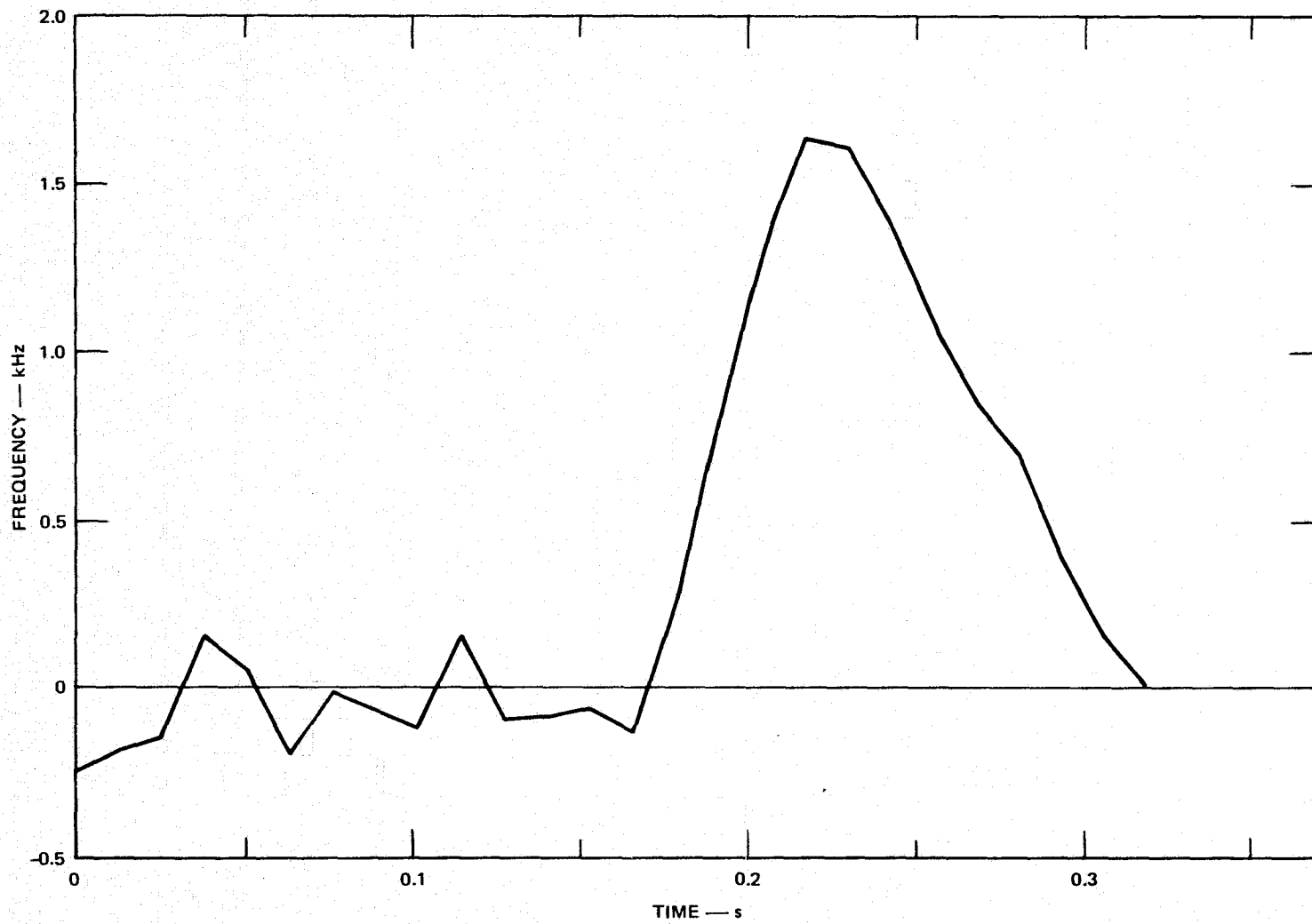
FIGURE 8 DIGITAL FIRST-MOMENT ESTIMATE OF PULSATILE WAVEFORM
