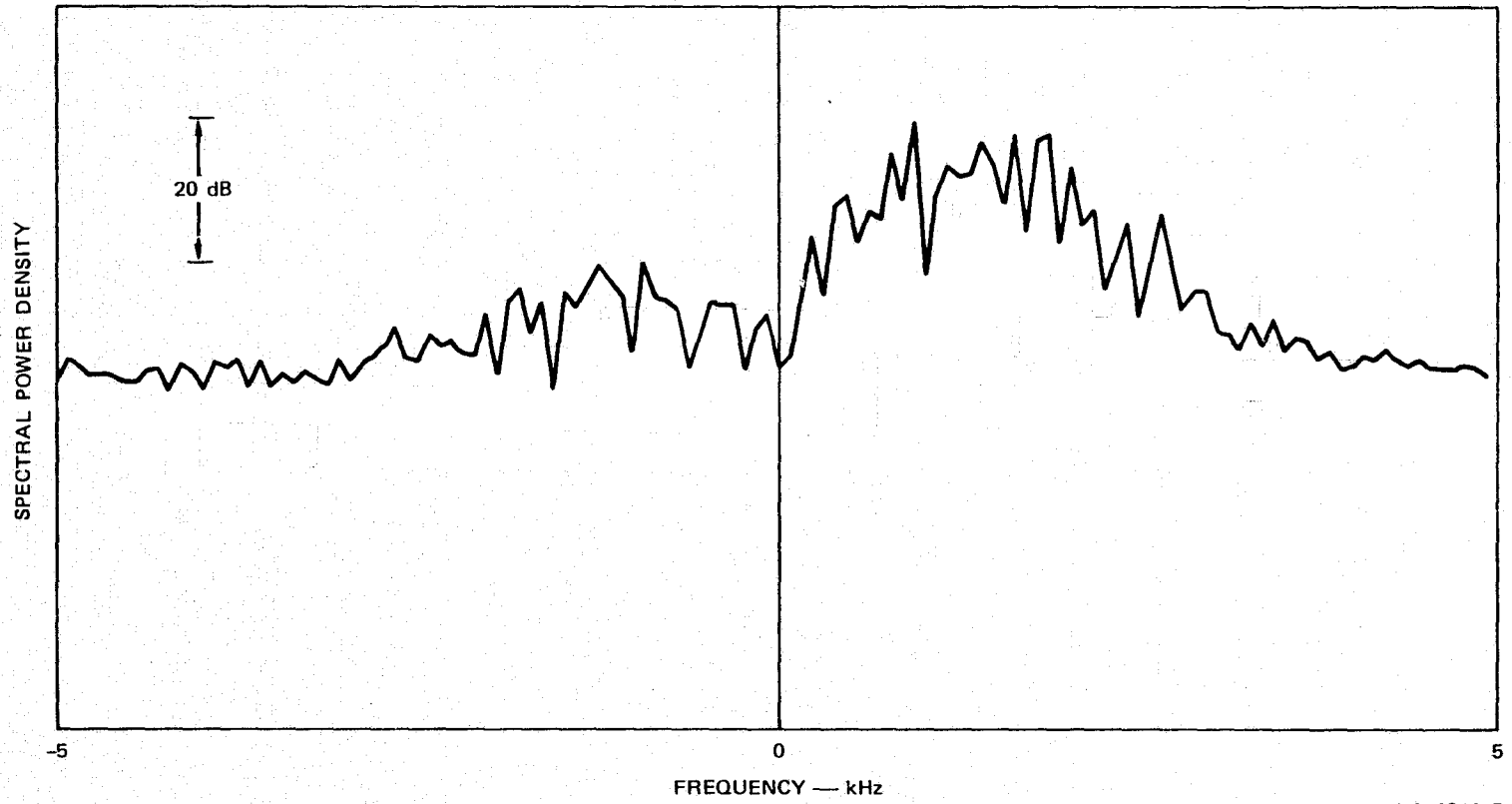
FIGURE 6 REPRESENTATIVE DOPPLER FLOW SPECTROGRAM
