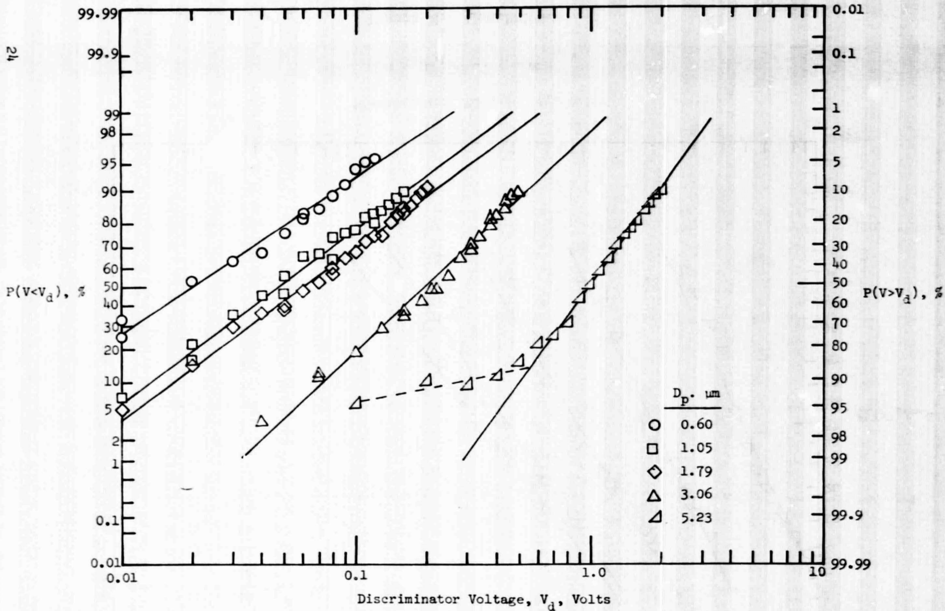
Figure 9. - Cumulative pulse height distributions for methylene blue aerosol. (Isokinetic sampling, D_d = 21.7 \mu\text{m}. )
