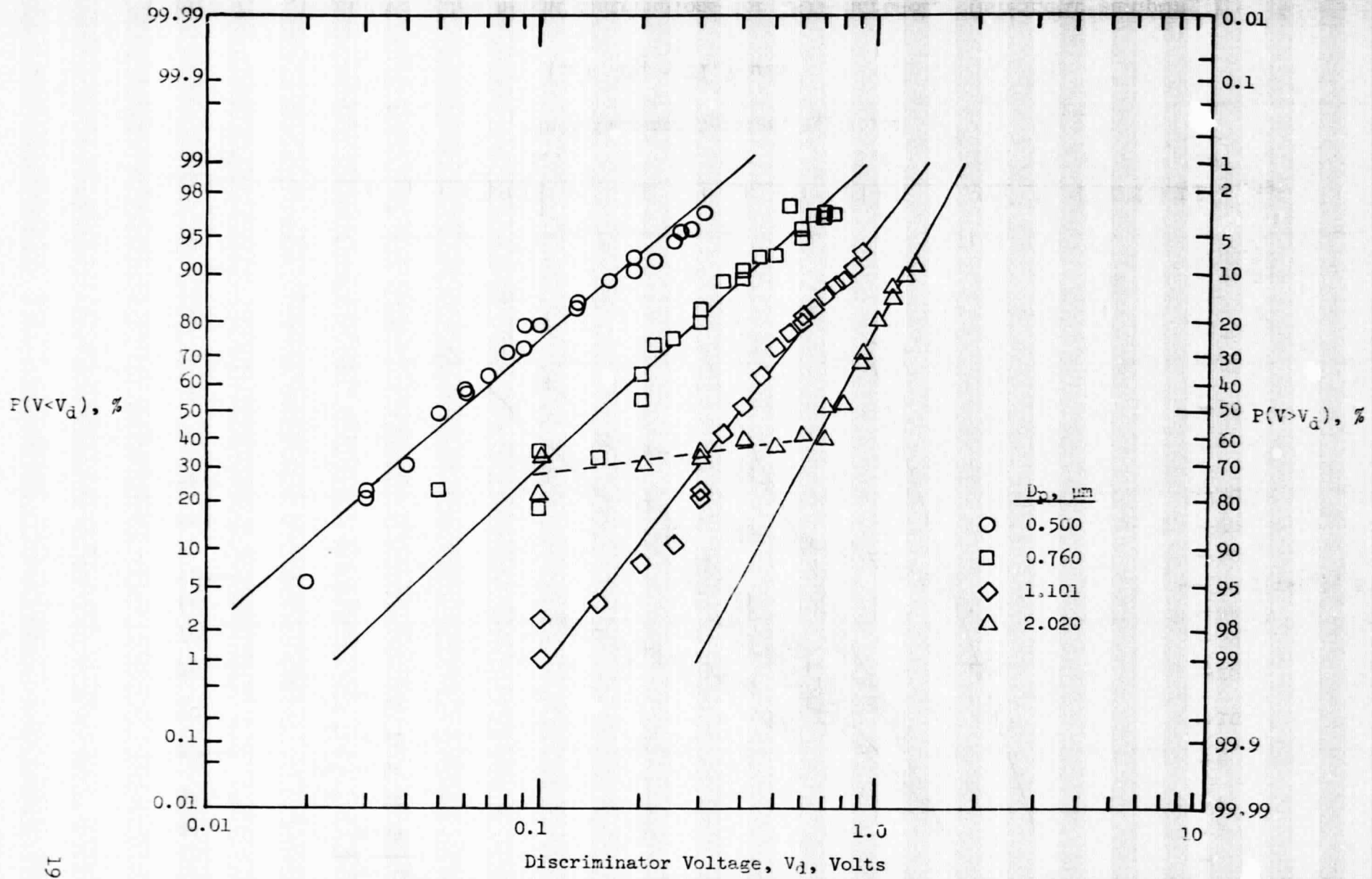
Figure 6. - Cumulative pulse height distributions for PSL spheres.
