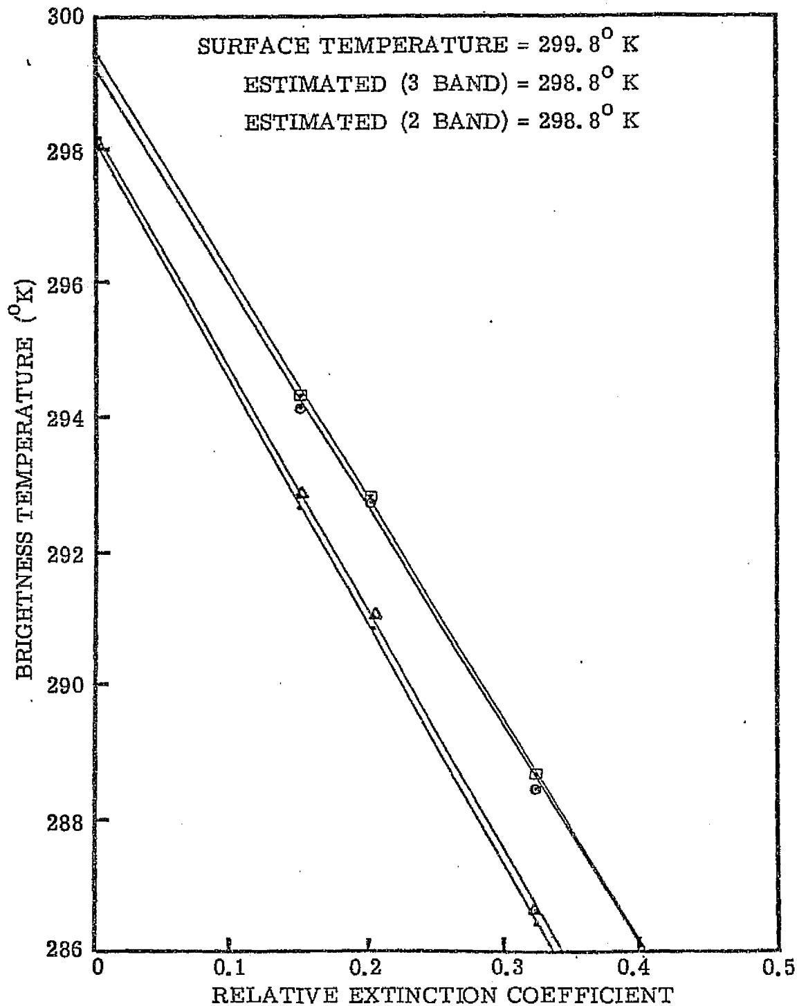
Figure 5e. Brightness Temperature Versus Extinction Coefficient. Key: □ Low Humidity, Continental-Maritime Haze; ○ Low Humidity, Maritime Haze; ▲ High Humidity, Continental-Maritime Haze; • High Humidity, Maritime Haze.
