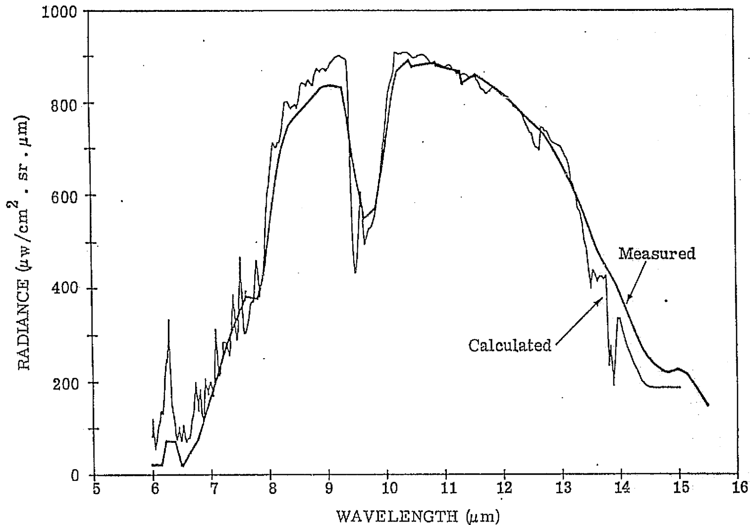
Figure 16. Comparison of Measured and Calculated Spectral Radiance for Monroe Reservoir, Salem, Illinois, on 10 June 1973. SST = 298^{\circ} K, \epsilon = 0.99 .
