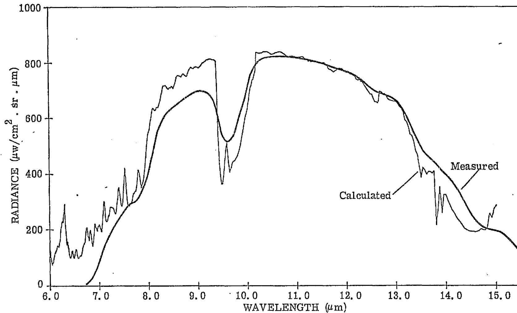
Figure 14. Comparison of Measured and Calculated Spectral Radiance for Key West on 8 January 1974. SST = 296^{\circ} K, \epsilon = 0.99 .
