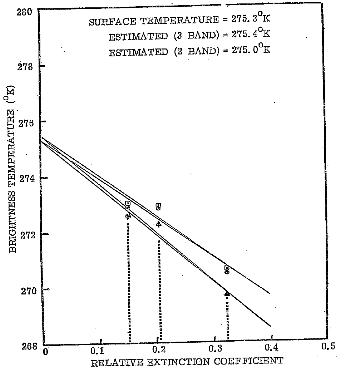
Figure 5a. Brightness Temperature Versus Extinction Coefficient. Key: □ Low Humidity, Continental-Maritime Haze; ○ Low Humidity, Maritime Haze; △ High Humidity, Continental-Maritime Haze; • High Humidity, Maritime Haze.
