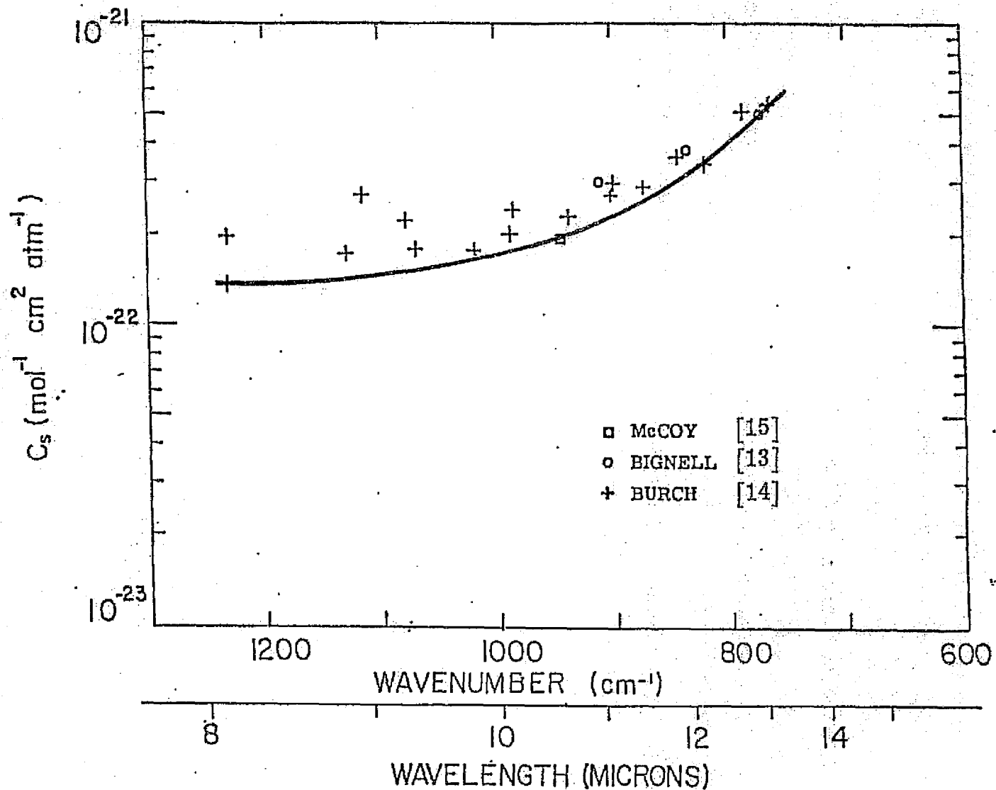
Figure 3. \text{H}_2\text{O} Self-Broadening Continuum Absorption Coefficient for Infrared Window Region at 296^\circ \text{K} .
