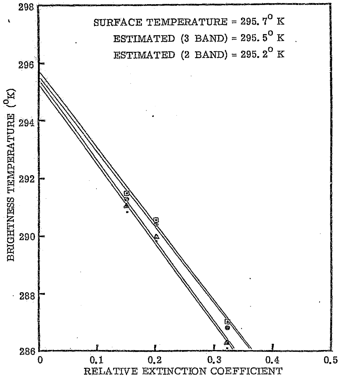
Figure 5d. Brightness Temperature Versus Extinction Coefficient. Key: □ Low Humidity, Continental-Maritime Haze; ○ Low Humidity, Maritime Haze; △ High Humidity, Continental-Maritime Haze; · High Humidity, Maritime Haze.
