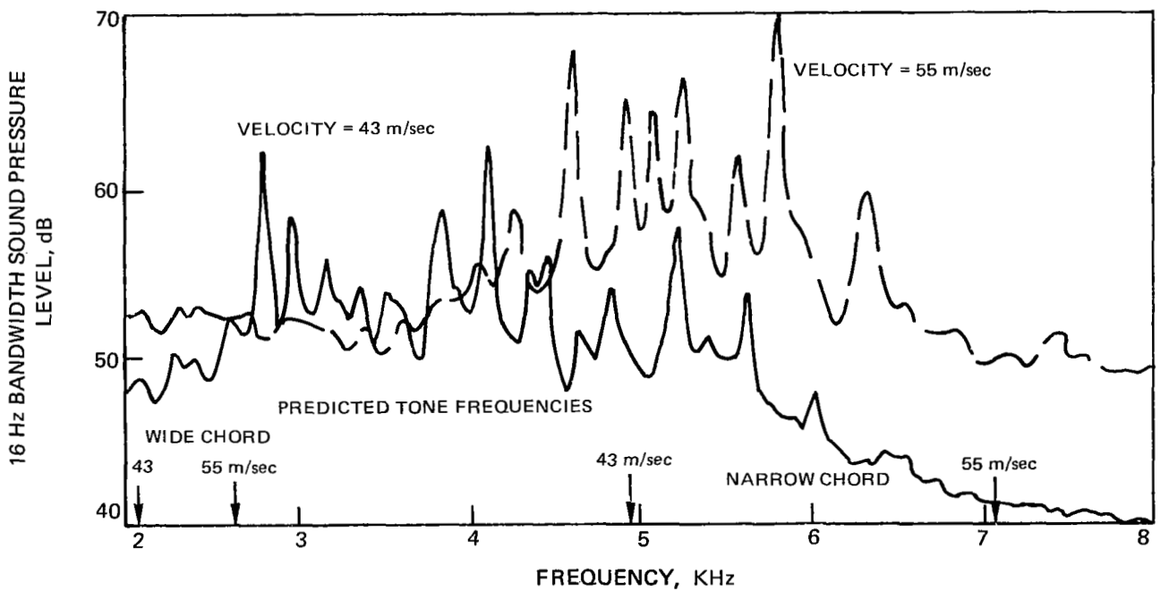
FIGURE 35 - NARROW BAND SPECTRA DIRECTLY ABOVE 4:1 TAPERED CHORD AIRFOIL AT 0° ANGLE OF ATTACK AND 30, 43, AND 55 m/sec VELOCITIES.
