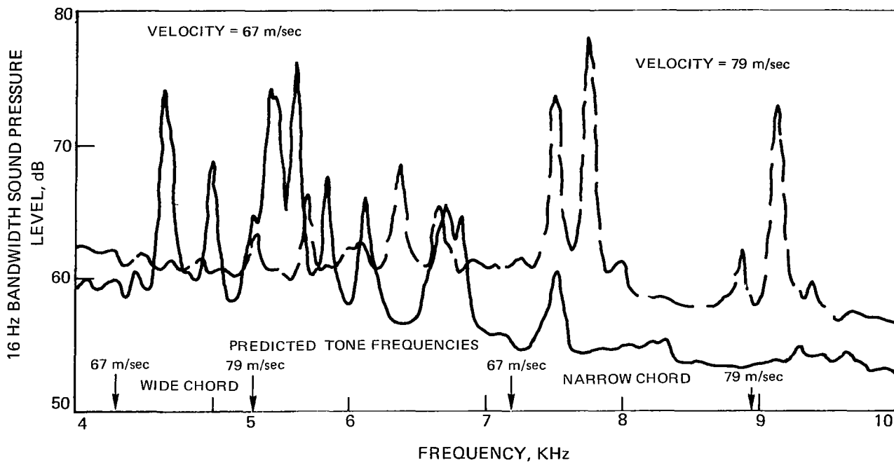
FIGURE 29 – NARROWBAND SPECTRA DIRECTLY ABOVE 2:1 TAPERED CHORD AIRFOIL AT -4^\circ ANGLE OF ATTACK AND 40, 52, 67, AND 79 m/sec VELOCITIES.
