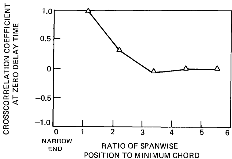
(b) VARIATION OF CROSSCORRELATION COEFFICIENT WITH SPANWISE POSITION
