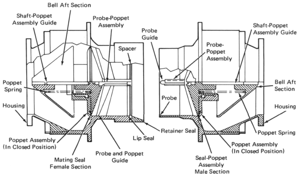
Quick-Disconnect Valve
