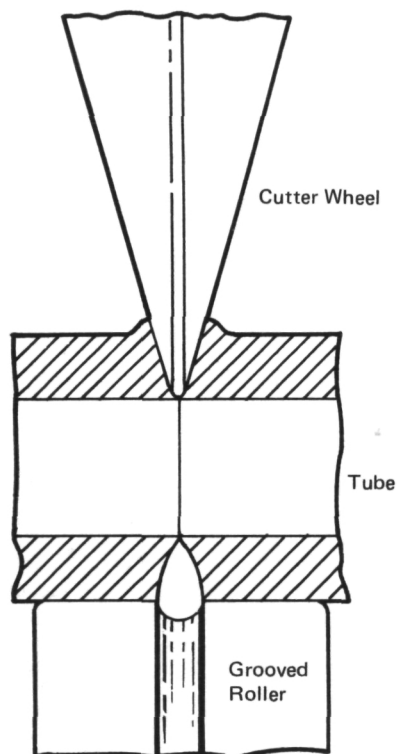
Tube Cutter
