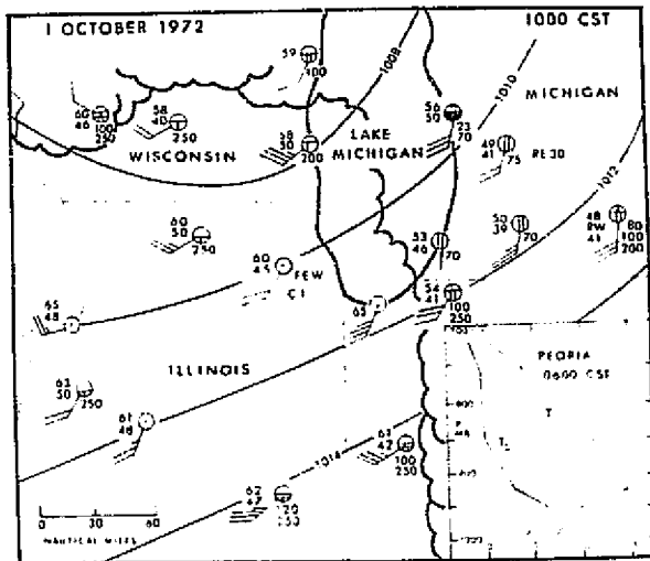
FIG. 4. Synoptic conditions, 1000 CST, 1 October 1972. An overcast area of altostratus is present to the north and east of the study area. Isobars every 2 mb, one wind bar equals 5 kt. Inset shows 0600 CST Peoria, Ill., radiosonde.
