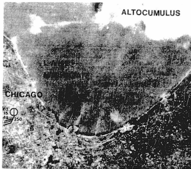
Figure 2. - Landsat-1 image, band 5 (0.6-0.7 micrometers), 1 October 1972, showing smoke plumes from steel mills drifting over Lake Michigan.
