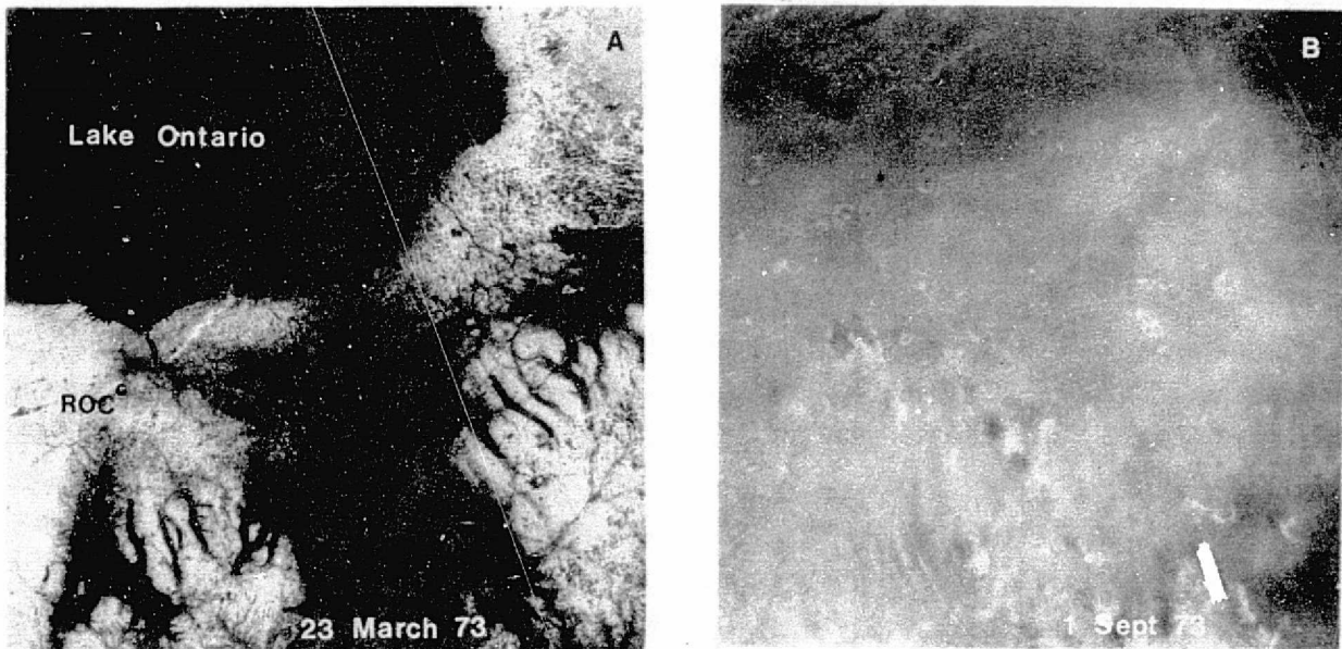
Figure 9(a) - Landsat-1 image, band 4, 0945 LST, 23 March 1973, of eastern Lake Ontario and the Finger Lakes, on a cloud-free day with low atmospheric turbidity. Snow cover is spotty through the region. Rochester, New York indicated by ROC.
