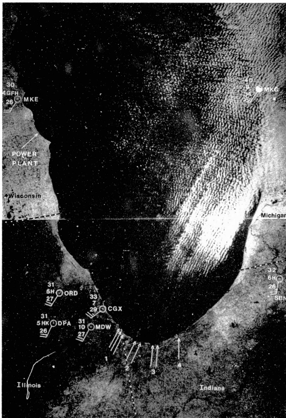
FIG. 2. ERTS-1 MSS Band 6 (0.6-0.7 \mu m) image over southern basin of Lake Michigan, 1003 CST 24 November 1972 (ERTS image ID No. 1124-16050). Hourly aviation weather plotted (one wind barb equals 2.5 m sec -1 ). Four major clusters of industry (arrows) form large combined plumes of suspended particulates. The width of the image shown is 165 km.
