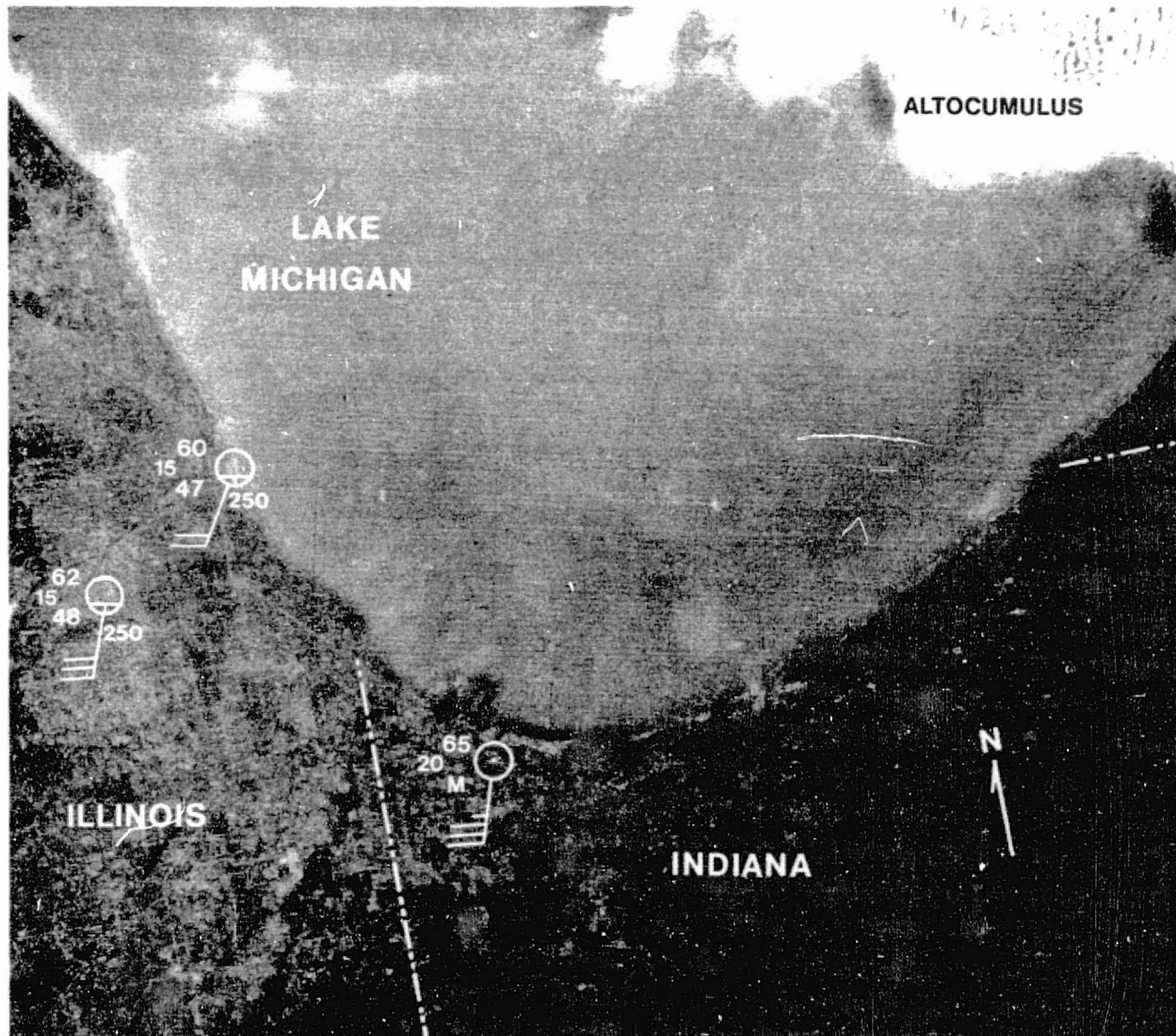
FIG. 5. ERTS-1 image, MSS-4 ( 0.5\text{--}0.6\ \mu\text{m} ) taken at 1003 CST, 1 October 1972. Aviation weather observations superimposed.
