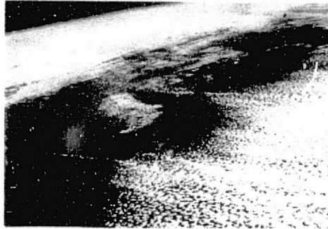
Figure 11. - Apollo manned orbital flight photograph of east coast, from Virginia to New York, during period of cold westerly flow over relatively warm ocean. The expected cumulus clouds form, but the two bands of clouds forming closer to land downwind of major industrial centers.
