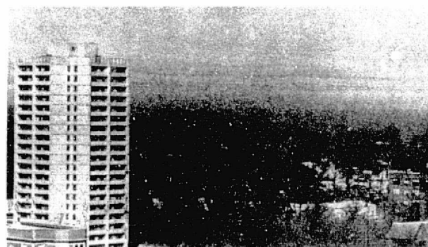
FIG. 1. Photograph, looking east, from University of Milwaukee-Wisconsin campus, showing layers of iron oxide red smoke over Lake Michigan, during brisk south-southeast winds and very stable conditions in March 1973. The source of the smoke is presumably the Chicago-Gary area.
