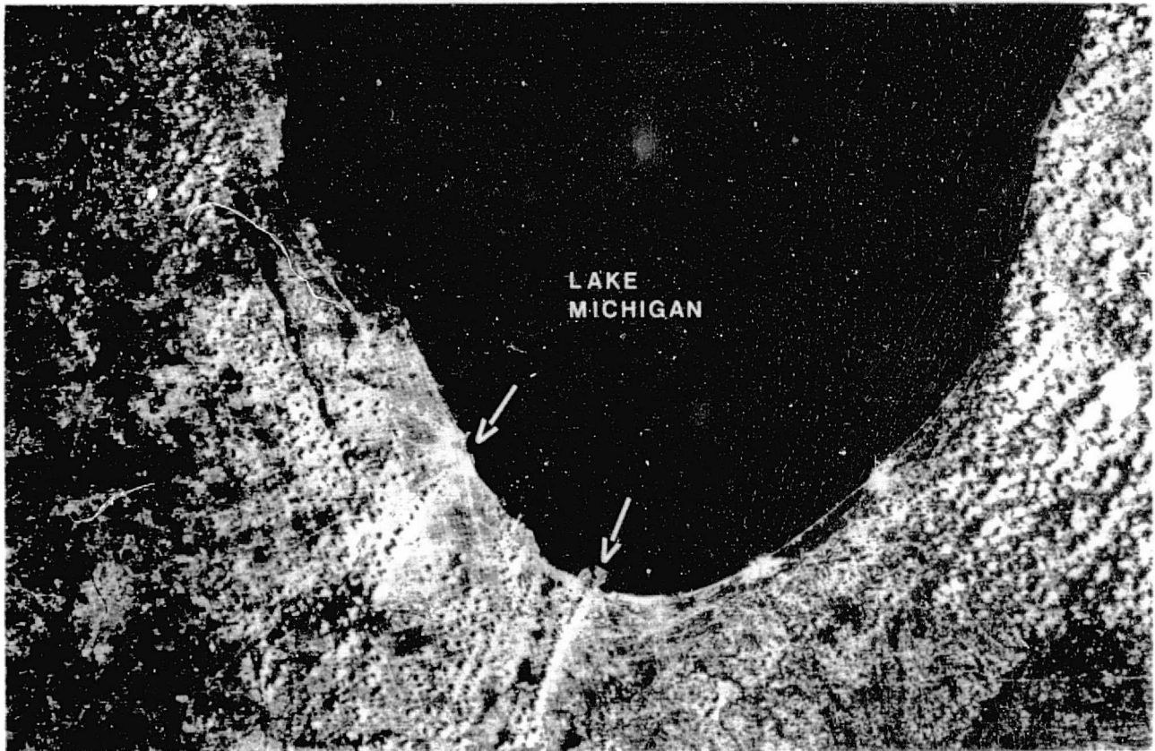
Figure 14. - Landsat-1 image, band 6, Chicago and southern Lake Michigan, 1003 LST, 16 July 1963. There was a general northeasterly flow throughout area, although a weak lake breeze was just pushing onshore along eastern shore. This caused the abrupt edge of cumulus there. Cumulus gradually reformed along the southern and western shore, with noticeable lines of clouds forming out of the plumes of major steel mills and industrial complexes (arrows).
