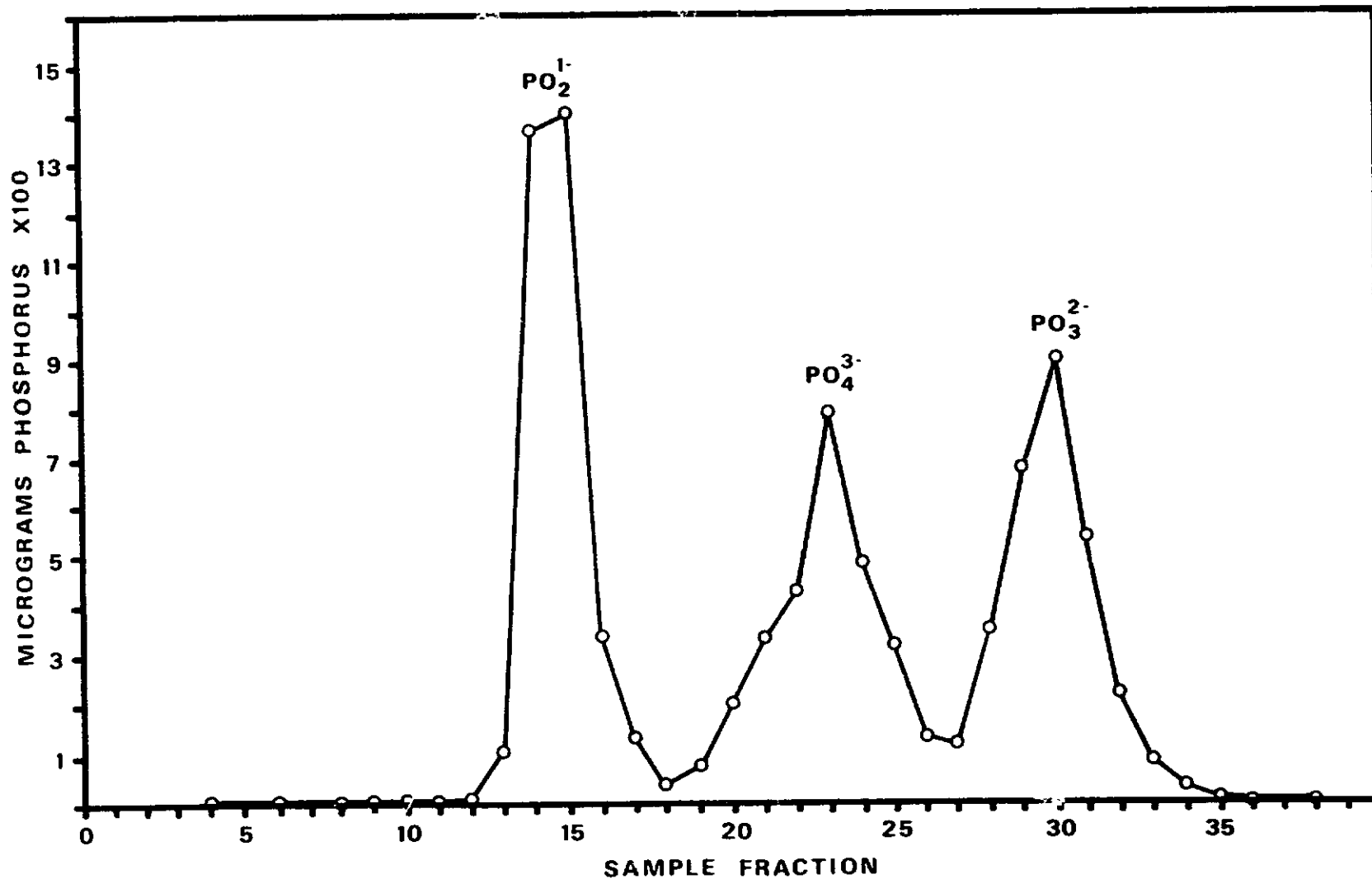
FIGURE 1: SEPARATION OF KNOWN HYPOPHOSPHITE ( PO_2^{1-} ), PHOSPHATE ( PO_4^{3-} ), AND PHOSPHITE ( PO_3^{2-} ) SAMPLES THROUGH A CHROMATOGRAPHIC COLUMN FOR QUANTITATIVE AND QUALITATIVE PROCEDURES.
