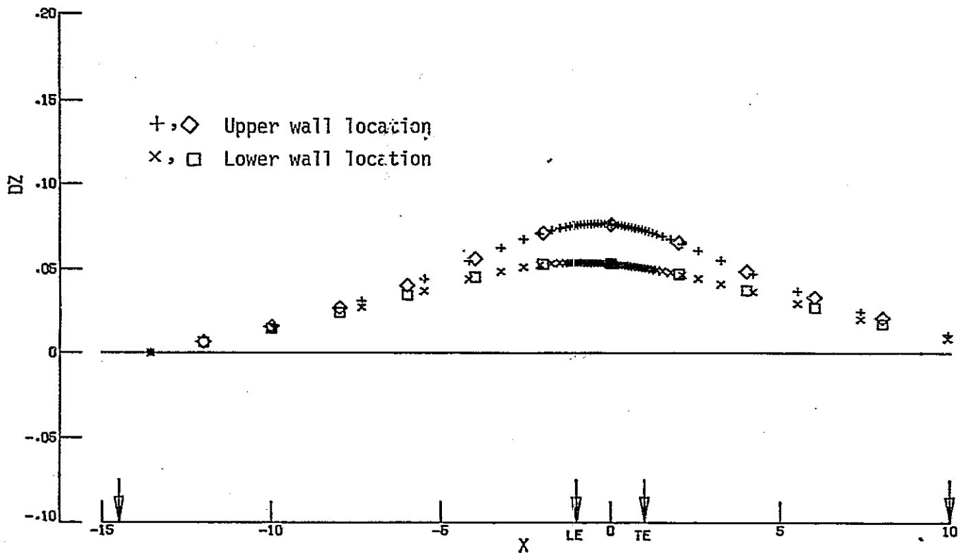
10 PERCENT PARABOLIC ARC - 2D MODEL APPROX. STREAM DEFLECTION DZ AT 6X19 UPPER AND LOWER TUNNEL WALL LOCATIONS OPEN SYMBOLS - DEFLECTION AT TUNNEL WALL JACK POSITIONS LINE SYMBOLS - DEFLECTION AT COMPUTATIONAL GRID POINTS (MULTIPLY BOTH DZ AND X BY HCHORD= 2.0000 TO GET INCHES)
