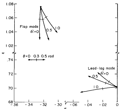
(a) Soft inplane, \omega_V = 0.7 .
