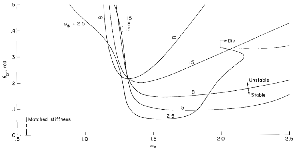
Figure 24.- The effect of torsion frequency on stability boundaries, \theta_{cr} versus lead-lag frequency: \beta_{pc} = 0.0 rad, R = 0.2 .
