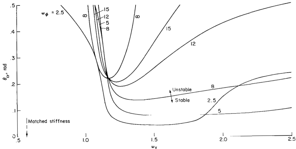
Figure 23.- The effect of torsion frequency on stability boundaries, \theta_{cr} versus lead-lag frequency: \beta_{pc} = 0.0 rad, R = 0.0 .
