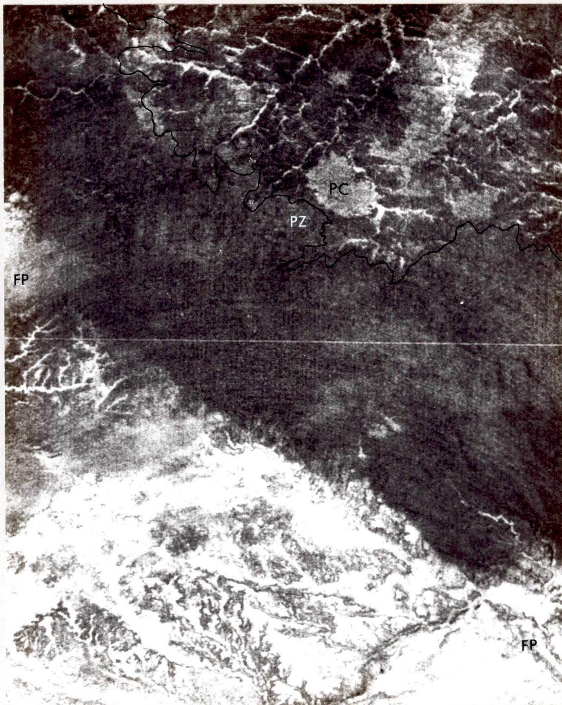
Figure 26. West-central Black Hills. Fanny Peak Lineament (FP), Precambrian (PC). Paleozoic (PZ).
