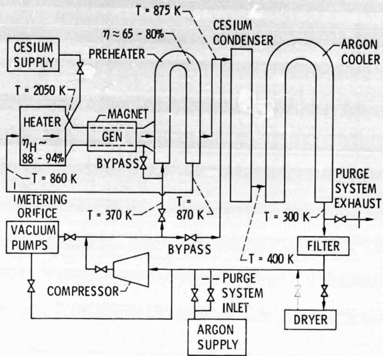
Figure 1. - Loop schematic.
