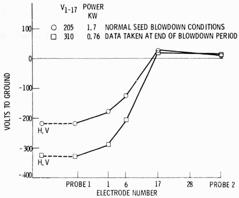
Figure 8. - Variation of Hall voltage along the channel for B = 1.68 \text{ T} , R_L = 40 \Omega
