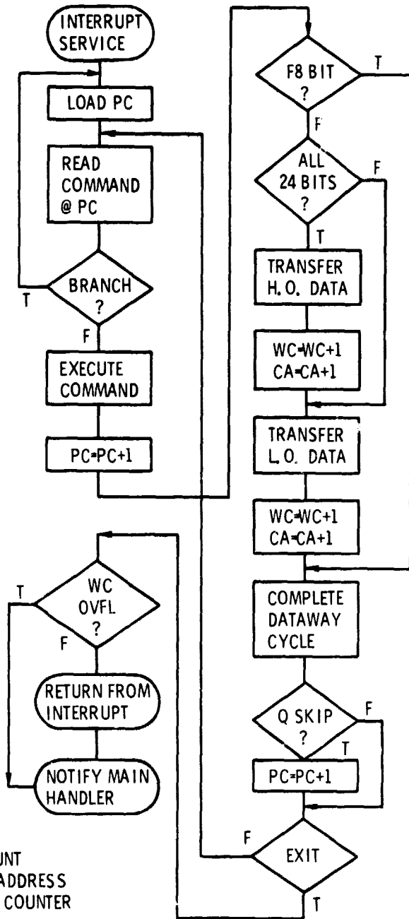
Figure 4. - Data transfer primitive.
