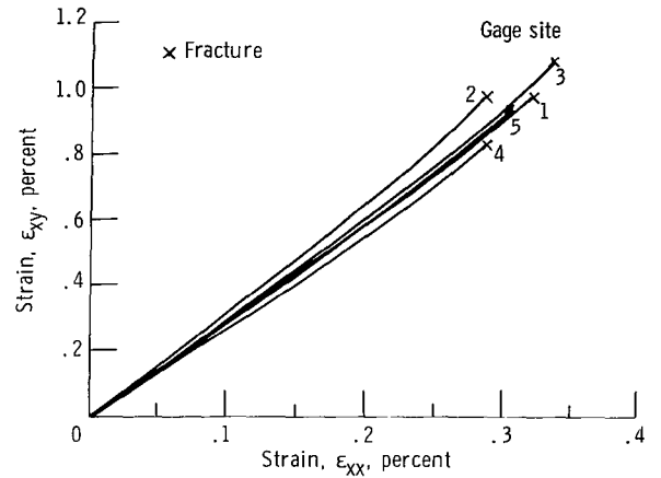
Figure 12. - Shear strain curves at various gage sites (fig. 8) for 10^0 off-axis tensile specimen (Mod-I/epoxy fiber composite).
