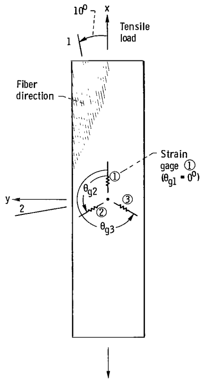
Figure 5. - Schematic depicting 10° off-axis tensile test specimen with strain gage positions ( \alpha, y - structural axes; 1, 2 - material axes).
