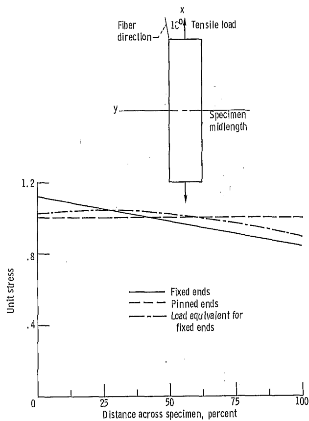
Figure 7. - Finite element analysis results of axial stress variation at midlength for three different boundary conditions; Mod-I/epoxy 10^\circ off-axis tensile specimen. (See fig. 6 for finite element representation.)
