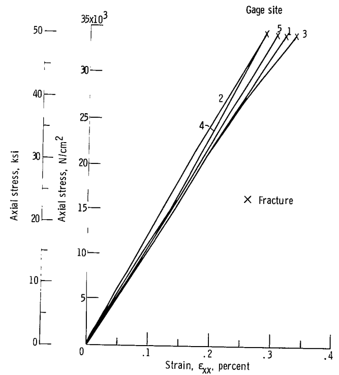
Figure 10. - Stress strain curves at various gage sites (fig. 8) for the 10^0 off-axis tensile specimen (Mod-I/epoxy fiber composite).
