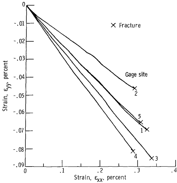
Figure 11. - Transverse (Poisson) strain curves at various gage sites (fig. 8) for 10^0 off-axis tensile specimen (Mod-I/ epoxy fiber composite).
