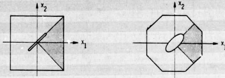
b) Plates with two planes (or lines) of reflection symmetry x_1 = \pm x_2 . Symmetry type II.
