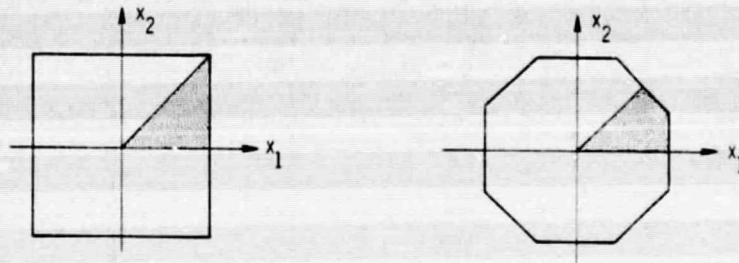
c) Plates with four planes (or lines) of reflection symmetry x_1 = 0, x_2 = 0 and x_1 = \pm x_2 . Symmetry types IV and IVa.
