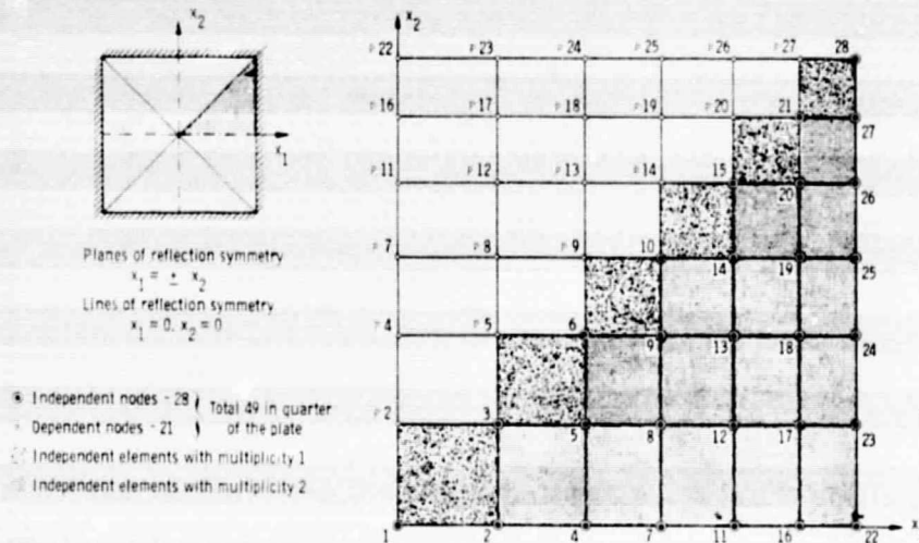
Figure 9 Independent nodes and elements for composite plates with two planes of reflection symmetry and two lines of reflection symmetry.
