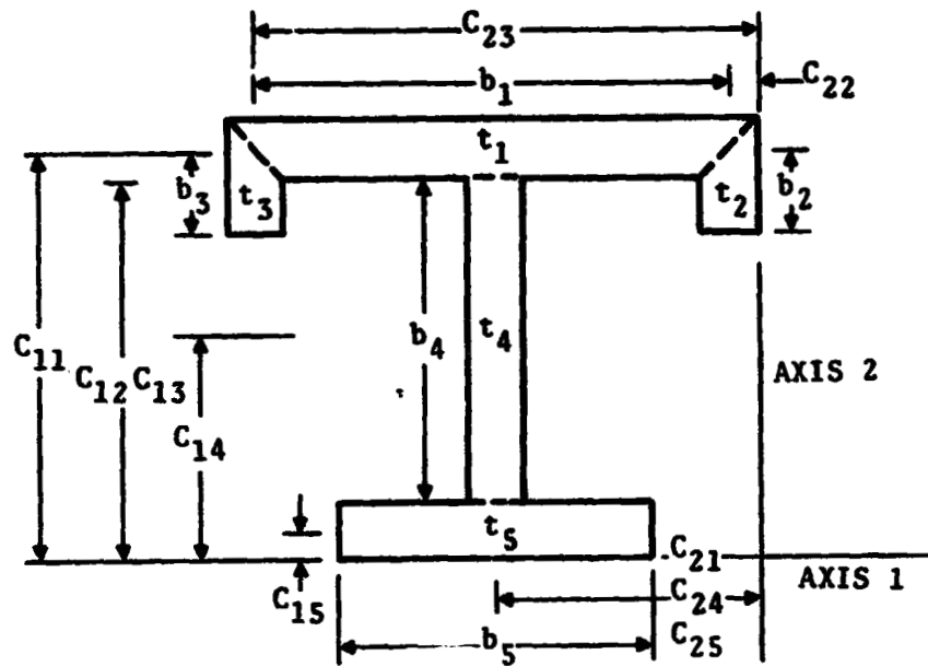
T-SECTION
