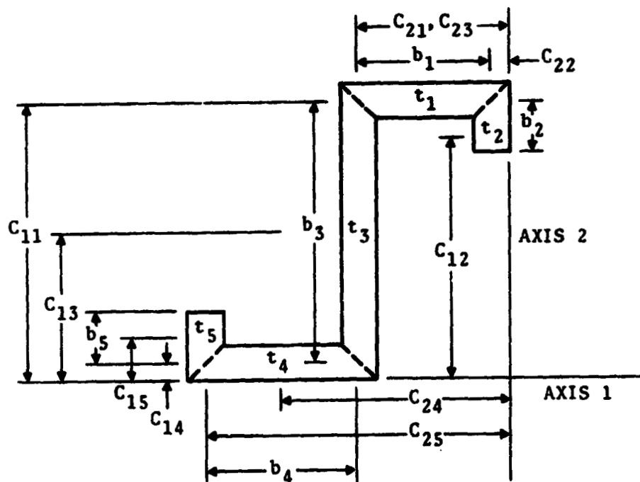
BULBED Z-SECTION
