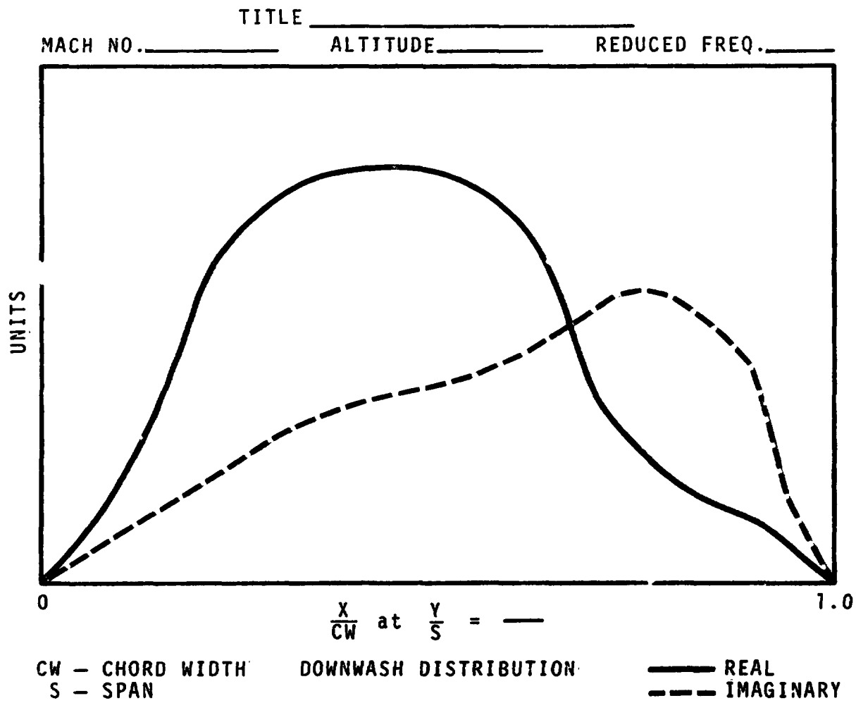
Figure 4.17-7. - Example of chordwise plot.
