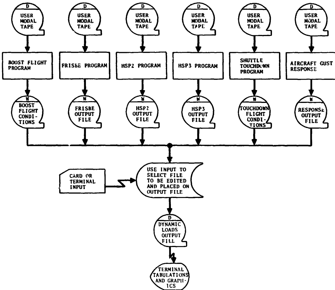
Figure 4.10-1. - Data flow diagram for Dynamic Loads.
