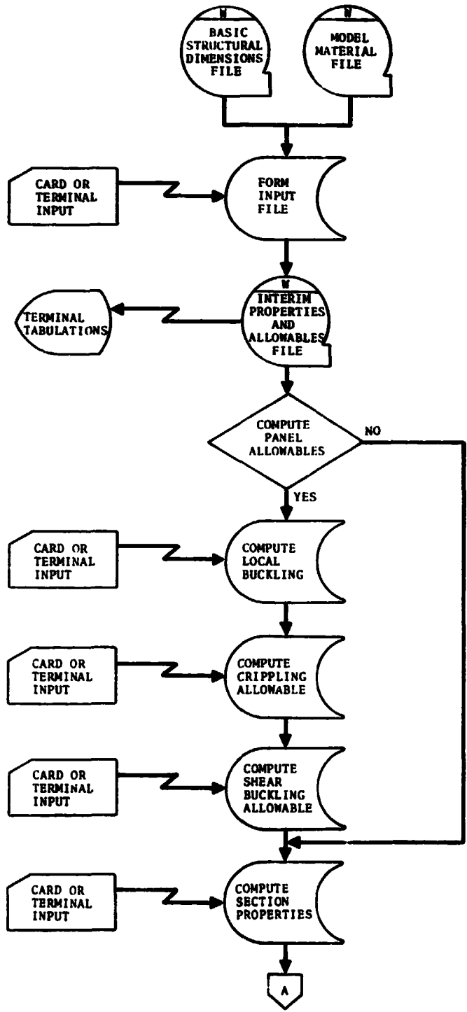
Figure 4.26-1. - Data flow diagram for Properties and Allowables.
