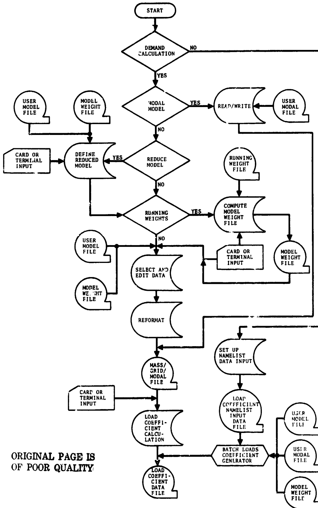
Figure 4.18-1. -- Data flow diagram for Load Coefficient Generator.
