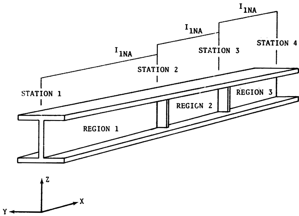
Figure 4.26-12. - Beam concept.
