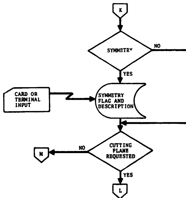
Figure 4.31-1. - Data flow diagram for User Model File Generator (continued).
