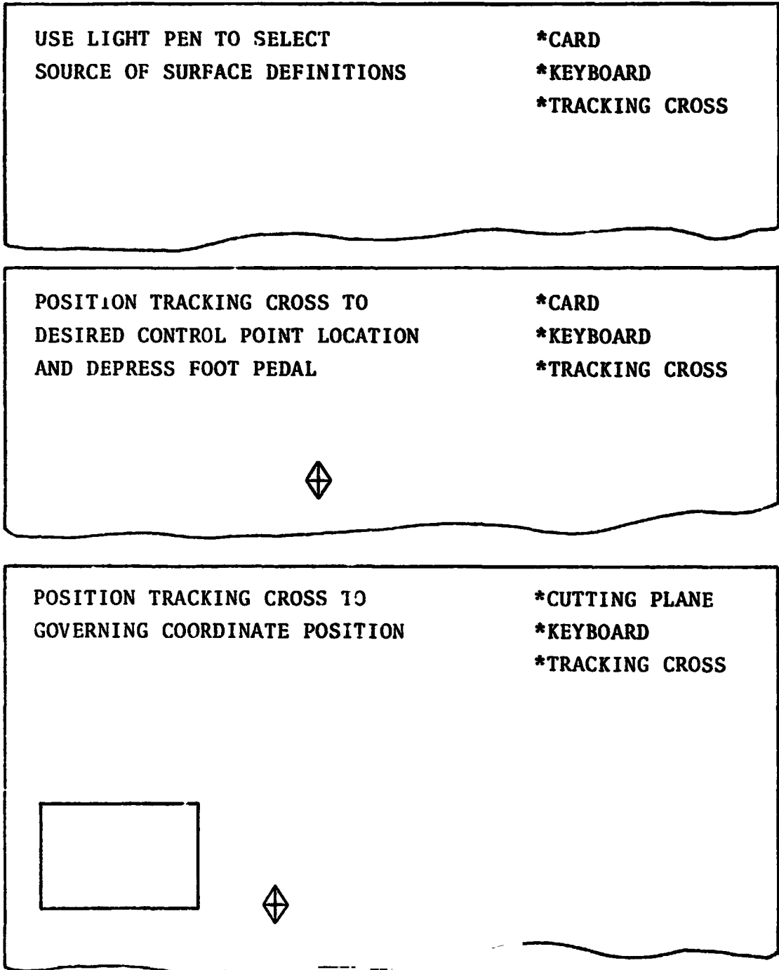
Figure 4.7-2. - Examples of display selectable input.
