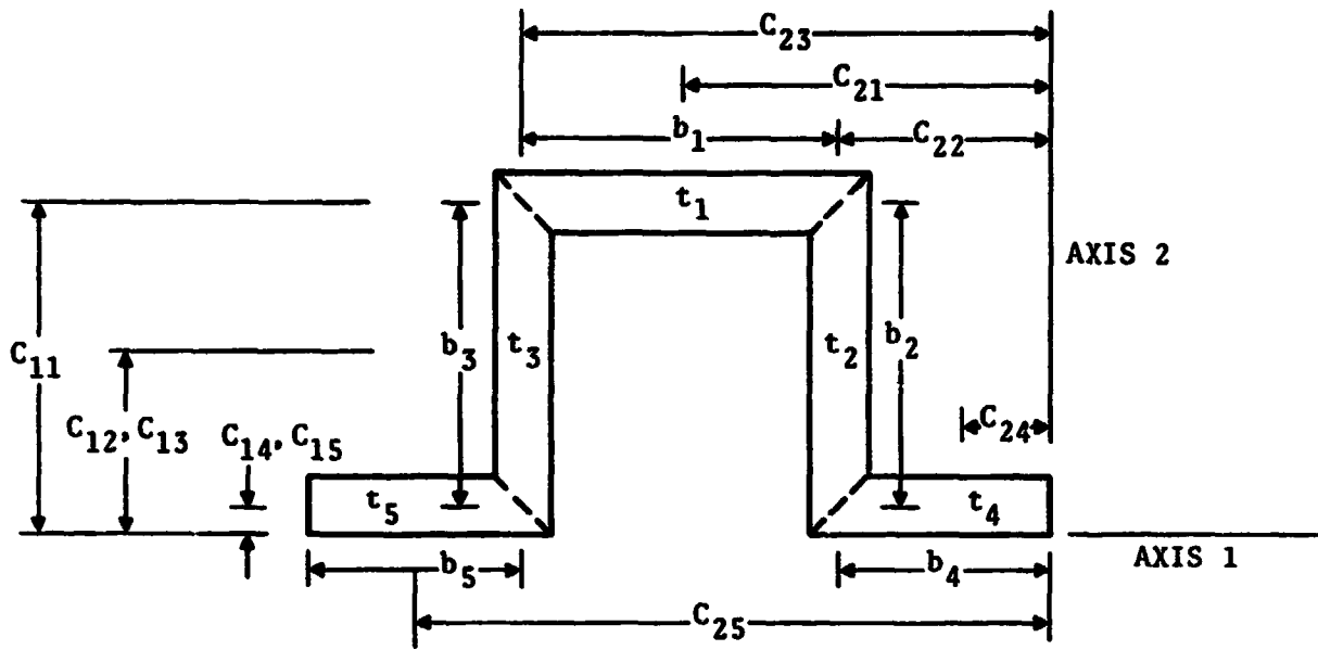
HAT-SECTION
