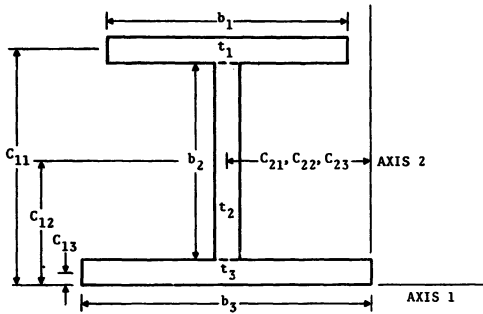
I-SECTION
