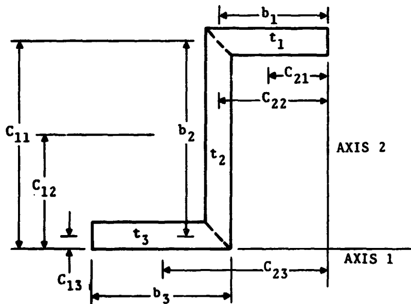
Z-SECTION
