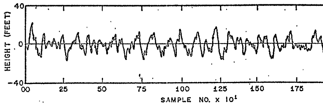
FIGURE 4. LASER MEASUREMENTS OF SURFACE WAVE CONDITIONS NEAR THE CENTER OF HURRICANE AVA. Flight level winds averaged for 1 minute were 6
