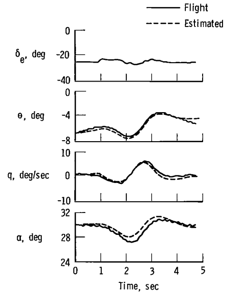
(a) Lateral-directional coupling terms ignored.
