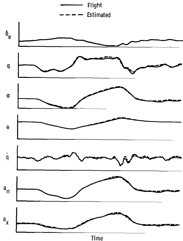
Figure 11. Comparison of flight data and data estimated by using a nonlinear model.
