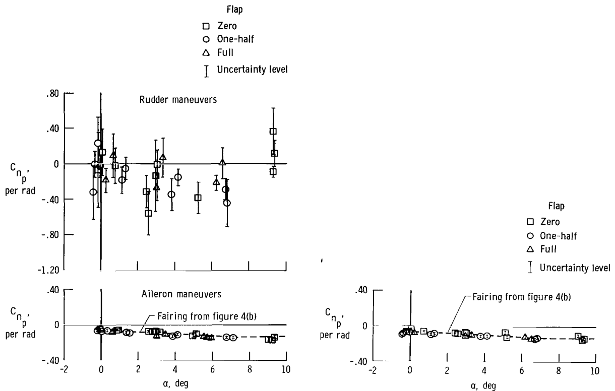
(a) Single maneuver analysis.
