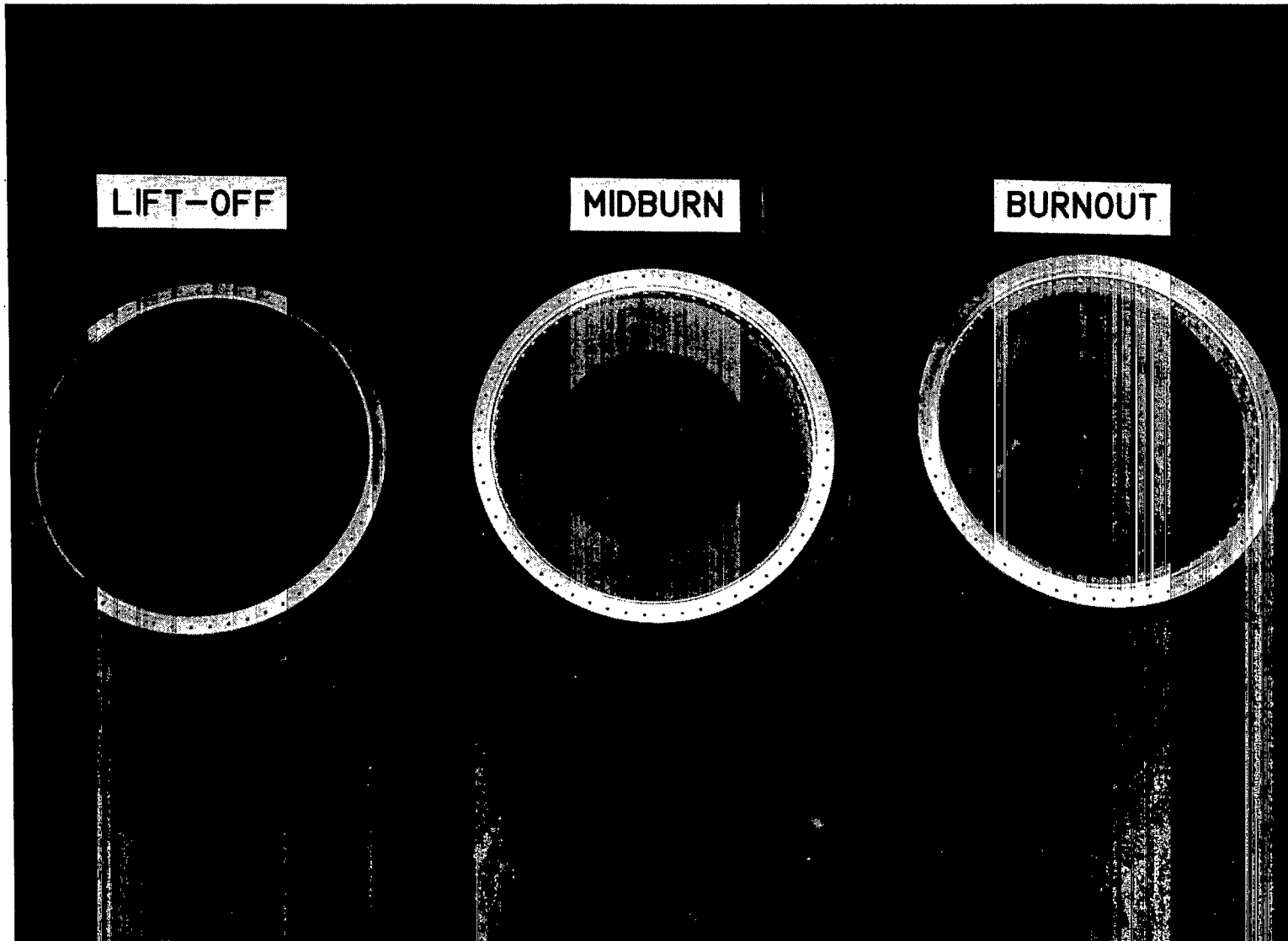
Figure 3.- Propellant cylinders of the 1/8-scale SRB model for different flight conditions.
