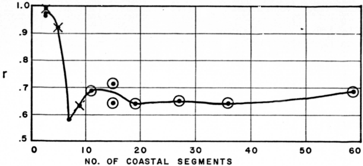
FIGURE 6-A: r vs. Number of Coastal Segments for Assateague Is. Before Removal of Anomalous Segments
