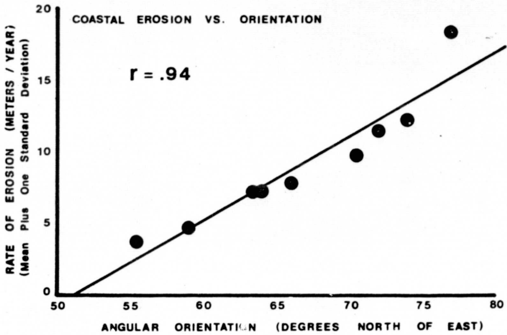
Figure 5: Analysis of Coastal Orientation vs. Coastal Erosion.
