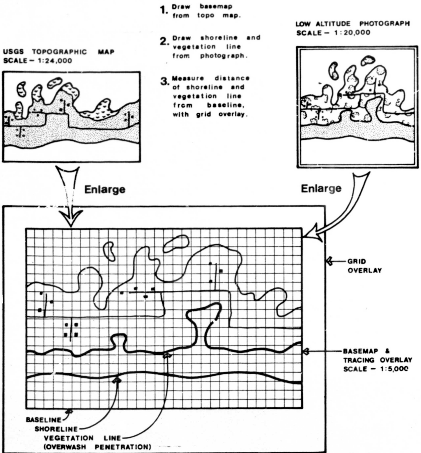
Figure 3: Method of Data Collection Using Historical Photography, Base Maps, and a Grid-Address System.
