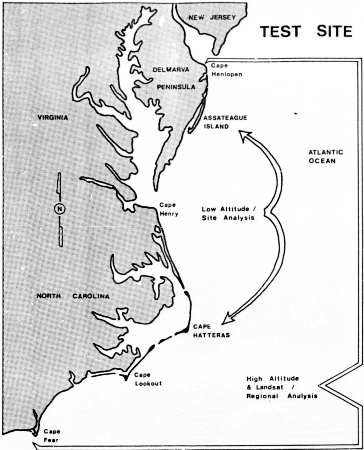
Figure 1: Barrier Islands of the Mid-Atlantic Coast.
