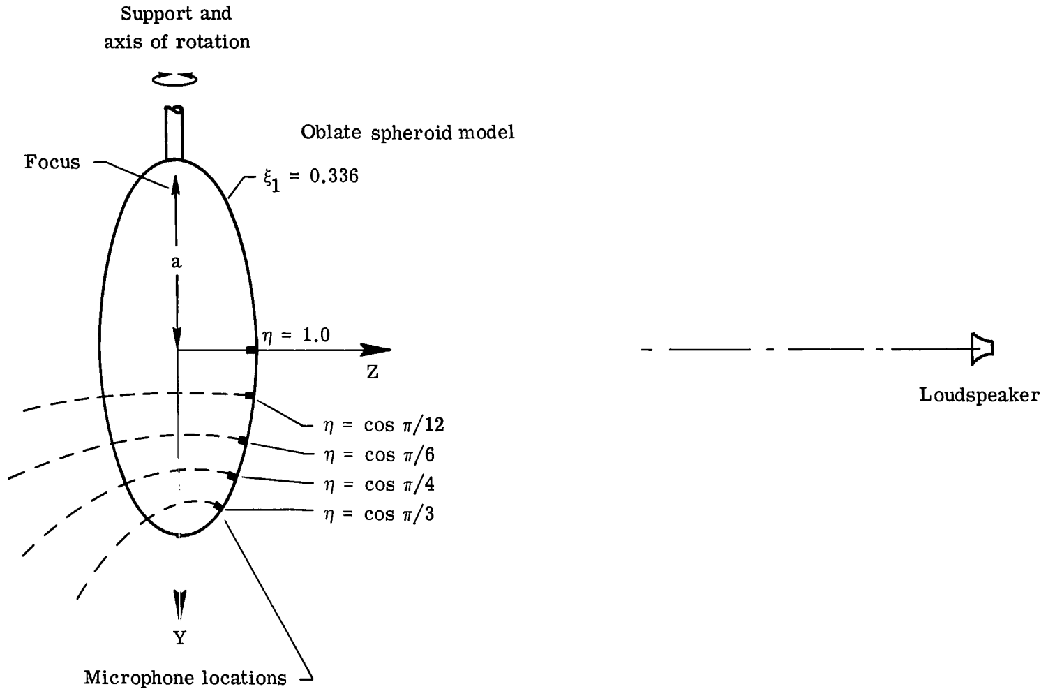
Figure 7.- Side view of experimental setup in terms of oblate spheroidal coordinate system for 180^\circ incidence.
