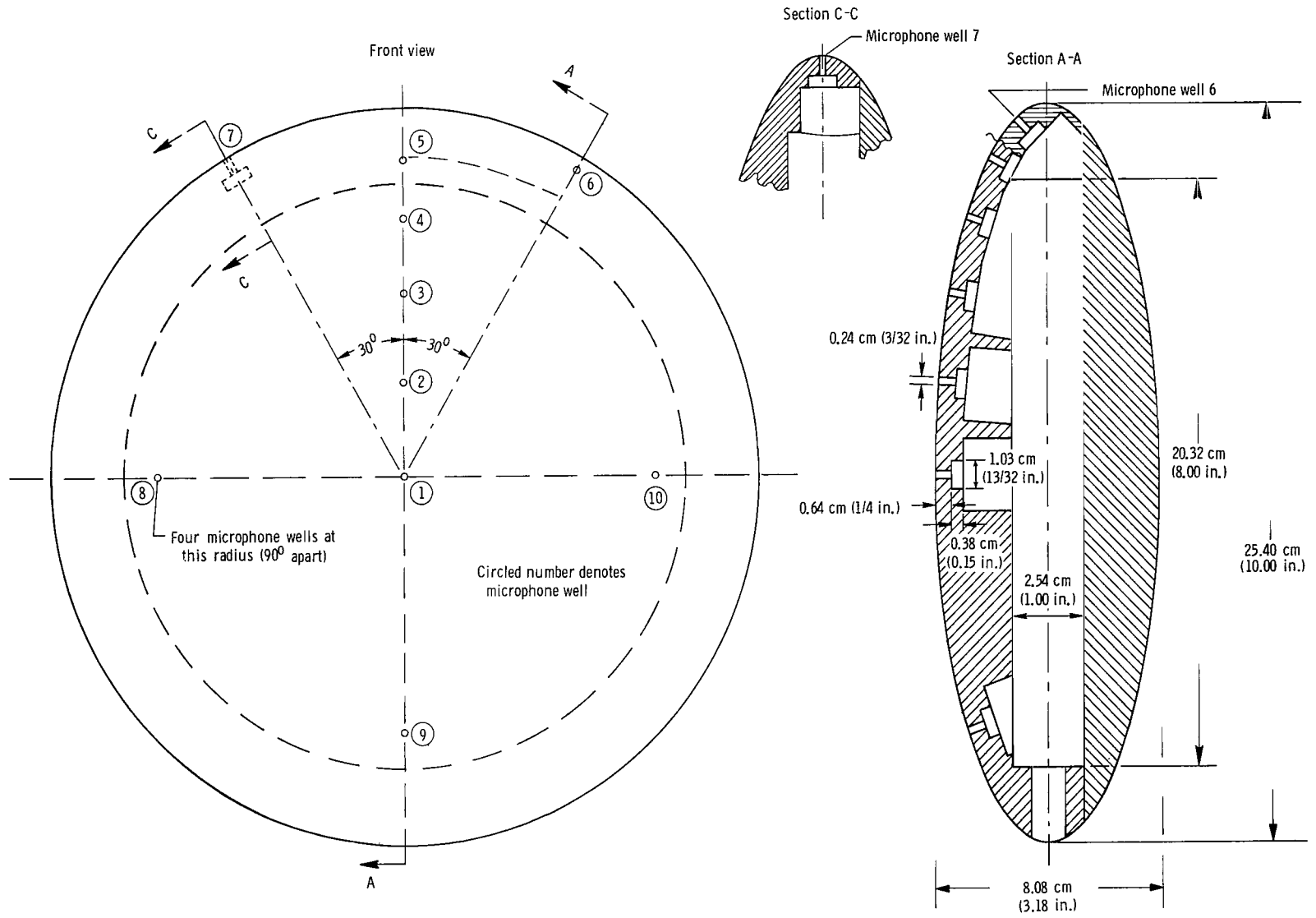
Figure 2.- Experimental model.
