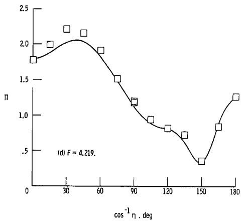
Figure 11.- Comparison of measured and calculated surface pressure augmentation due to scattering for 180^\circ incidence to the oblate spheroid \xi_1 = 0.336 .
