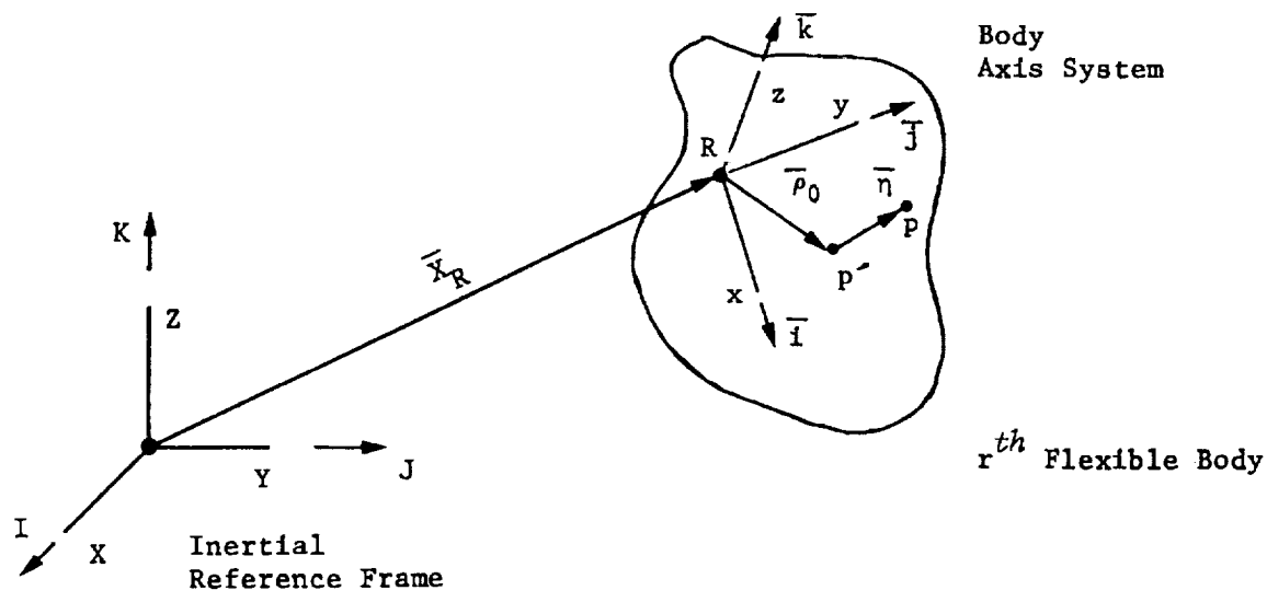
Figure II-1 The r^{th} Flexible Body
