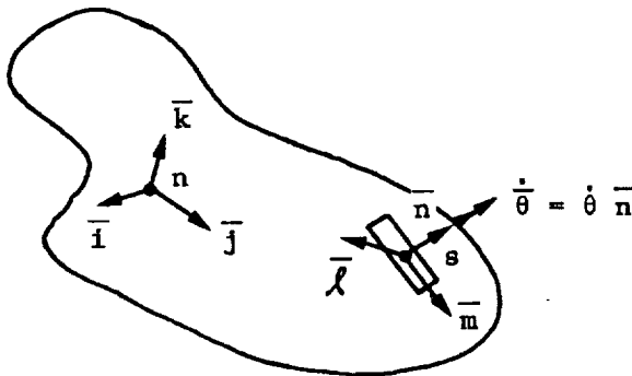
Figure II-4 Typical Body-Momentum Wheel Relationship
