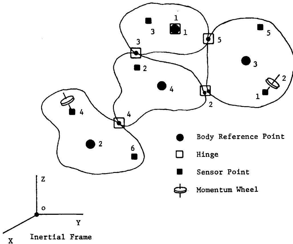
Figure I-1 Labeling Scheme for Example System
