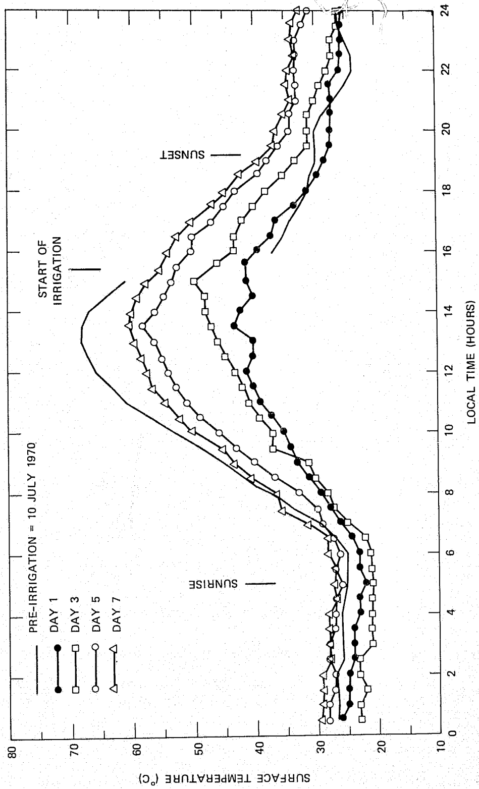
Figure 1. Diurnal surface temperature variation
