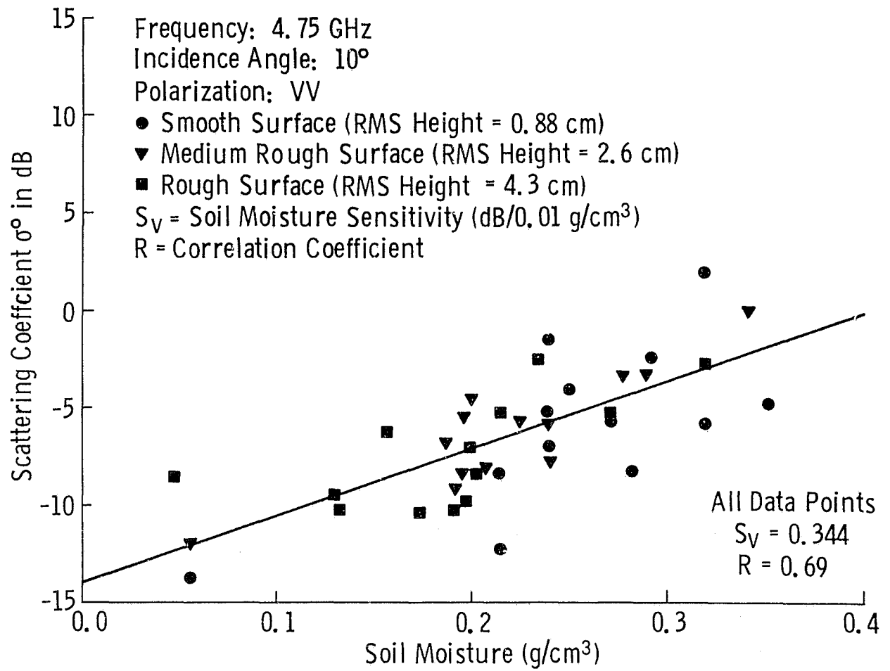
Figure 11. Soil moisture response of \sigma^o for the three surface roughnesses
