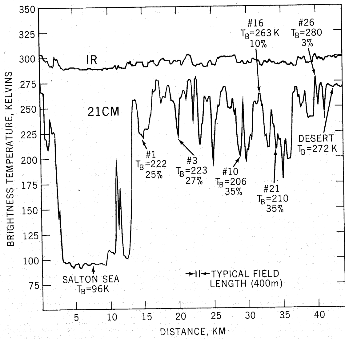
Figure 5. Infrared (10-12 \mu m) and 21 cm brightness temperature over Imperial Valley, California
