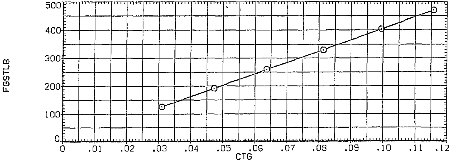
FIG. 11 STATIC THRUST CALIBRATION- CONFIGURATIONS 2 AND 3
