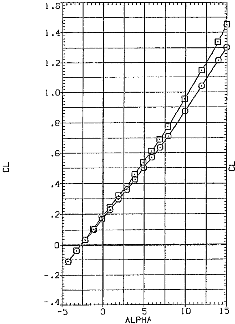
FIG. 12 REYNOLDS NUMBER SENSITIVITY WITH JET ON (A) MACH = .70
