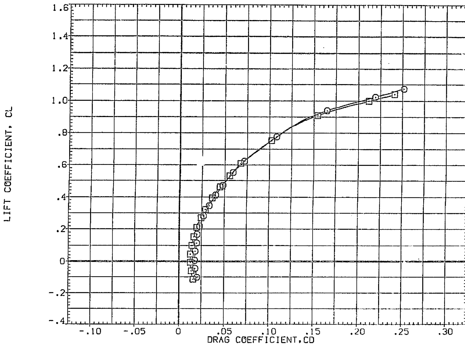
FIG. 9 REPEATABILITY EVALUATION- CONFIGURATION 2 CAJMACH = .70
