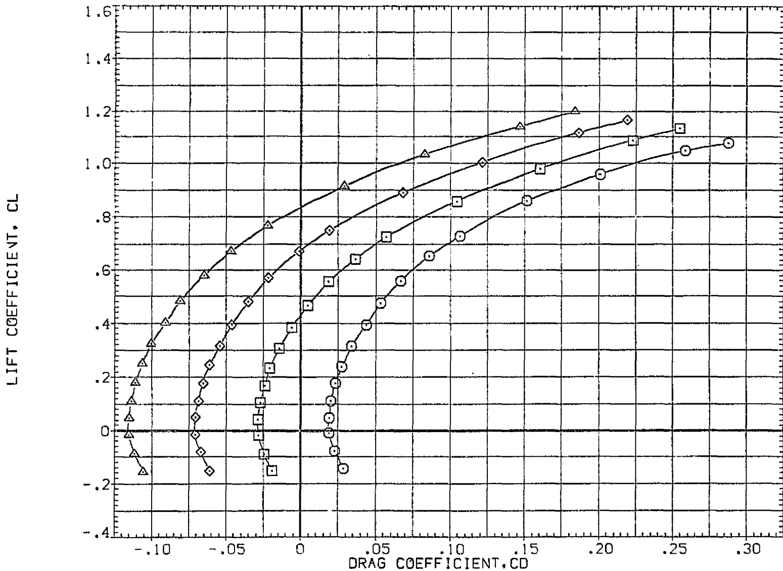
FIG. 13 EFFECTS OF BLOWING ON CONFIGURATION 2 (A) MACH = .90
