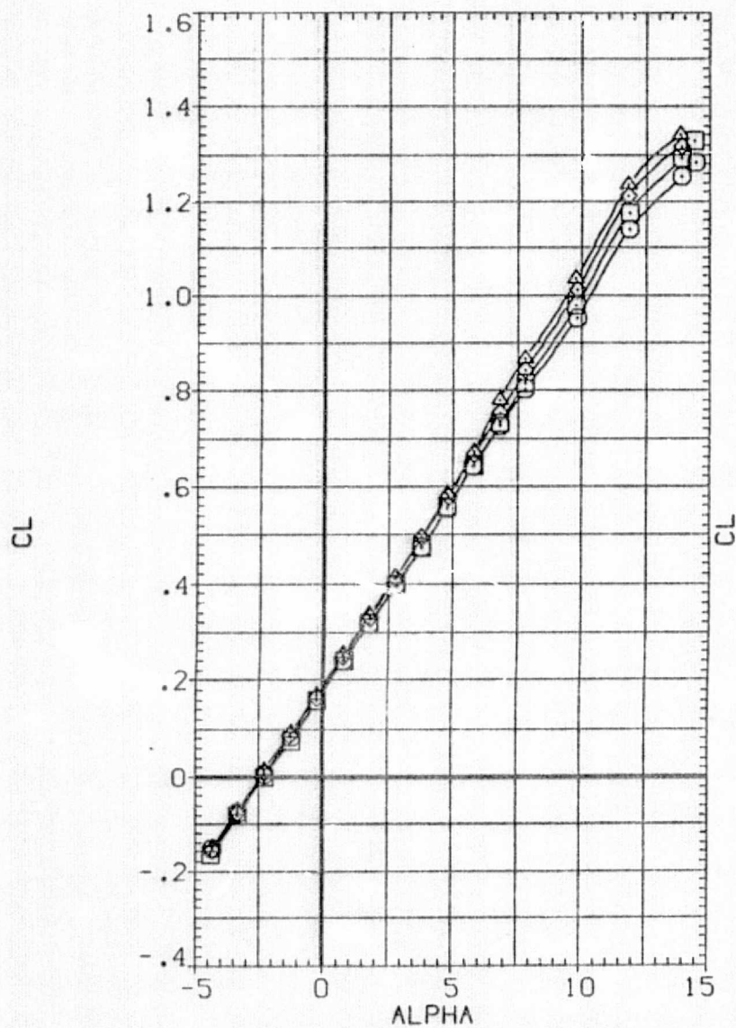
FIG. 13 EFFECTS OF BLOWING ON CONFIGURATION 4
