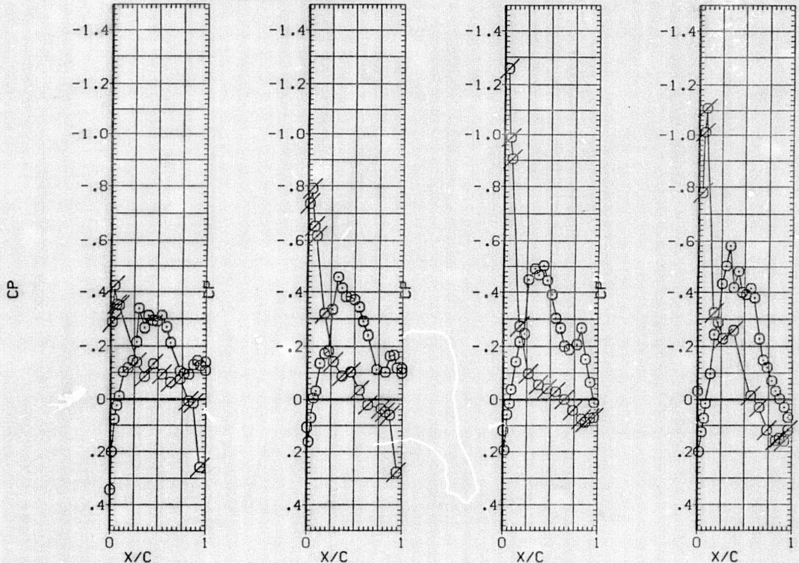
FIG. 15 PRESSURE DISTRIBUTIONS OVER CONFIGURATION 5 AT CTG=0.12
