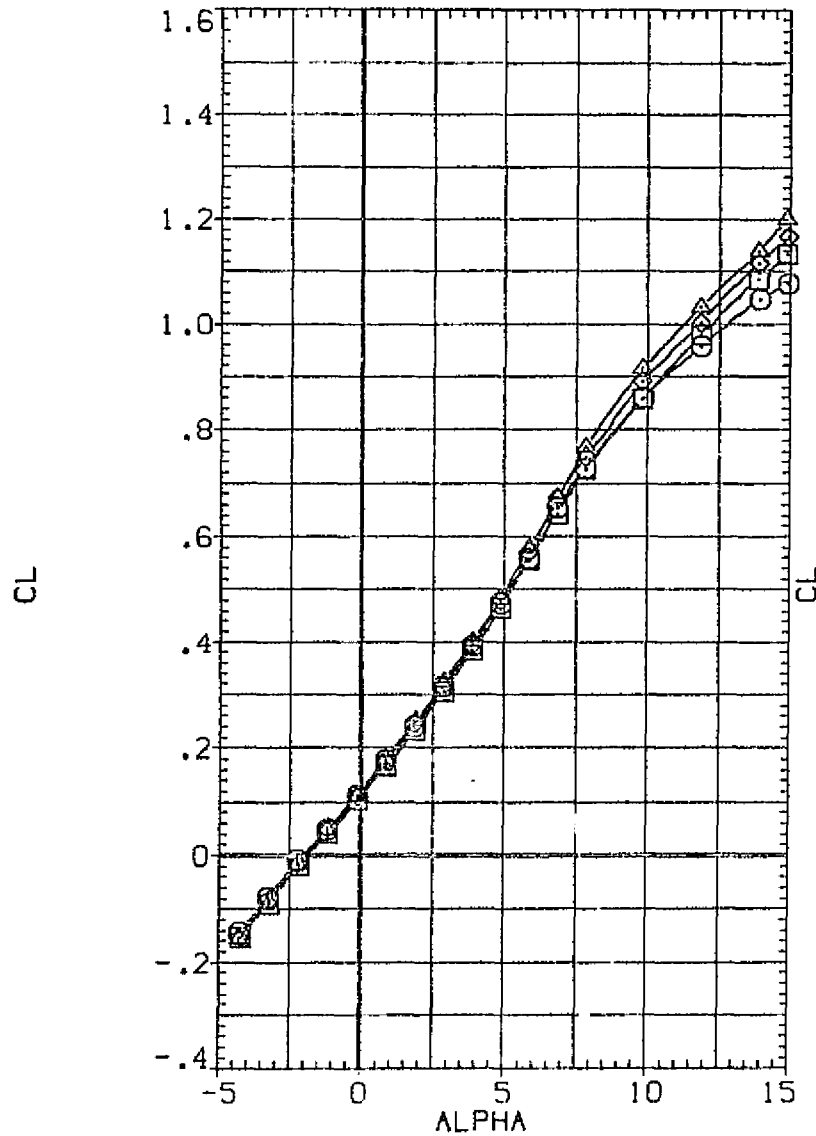
FIG. 13 EFFECTS OF BLOWING ON CONFIGURATION 2 (A) MACH = .90
