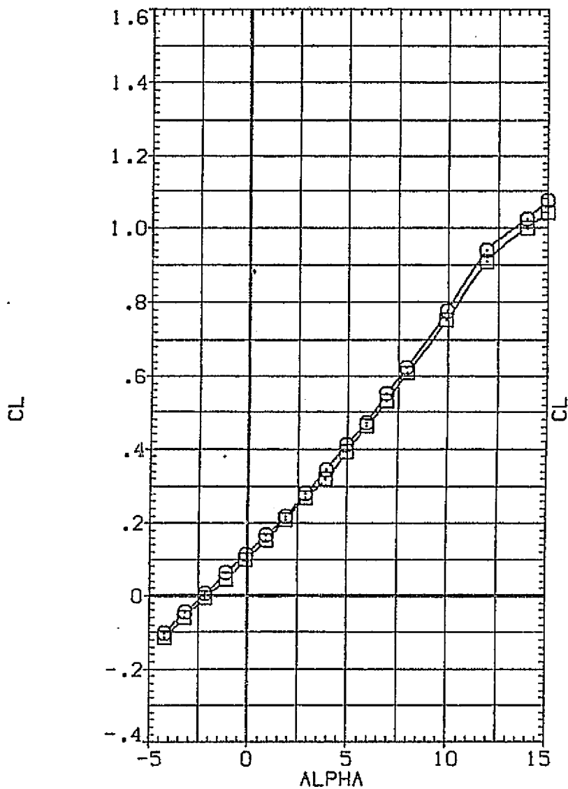
FIG. 9 REPEATABILITY EVALUATION- CONFIGURATION 2 (A)MACH = .70
