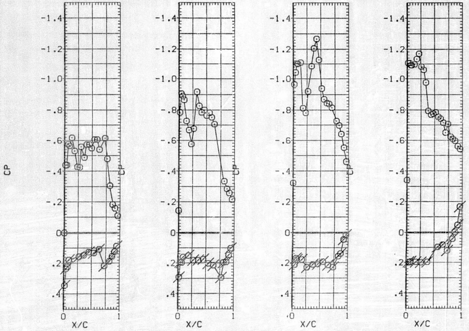
FIG. 15 PRESSURE DISTRIBUTIONS OVER CONFIGURATION 4 AT CTG=0.0
