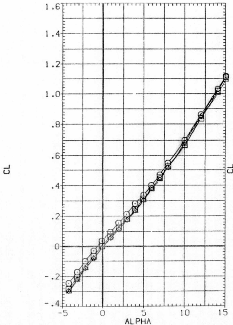
FIG. 13 EFFECTS OF BLOWING ON CONFIGURATION 5
