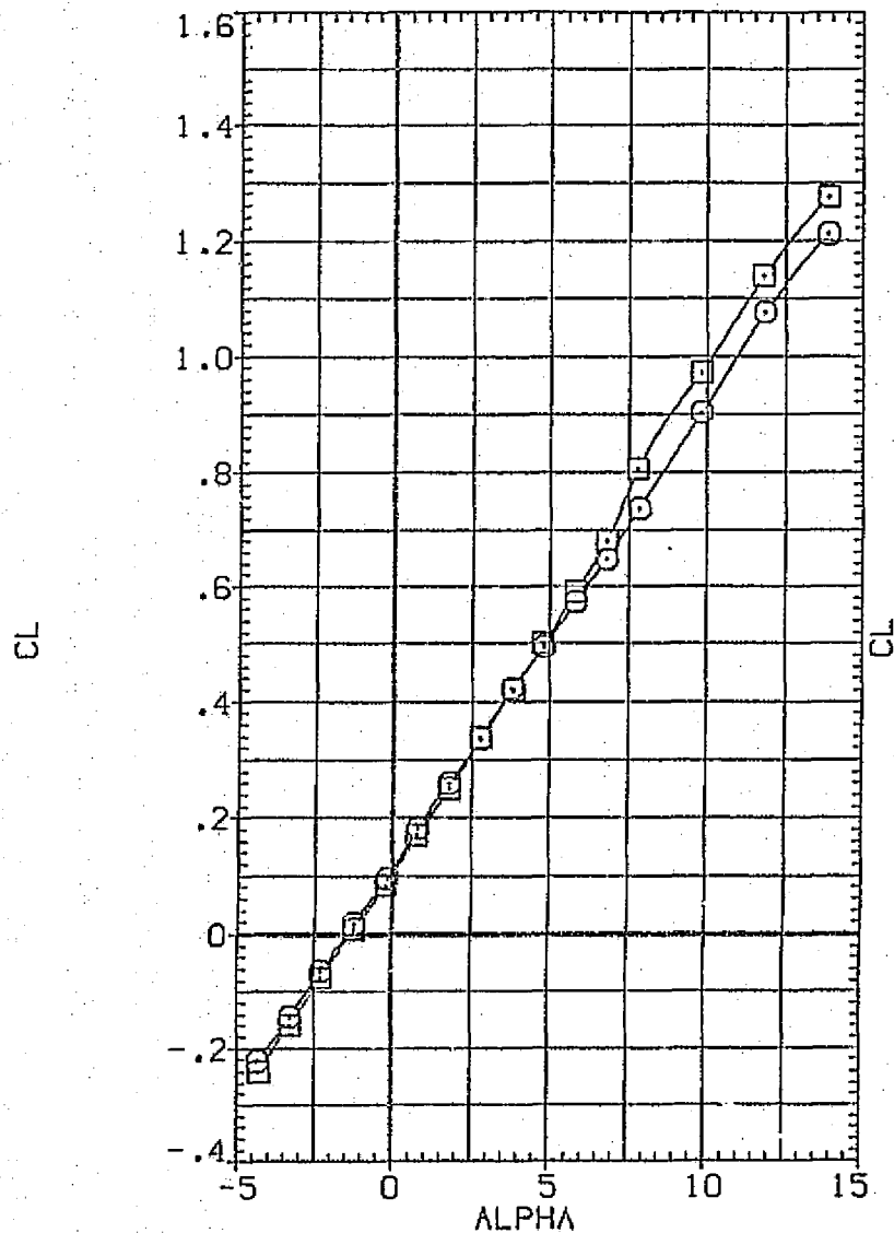
FIG. 13 EFFECTS OF BLOWING ON CONFIGURATION 3 (CO)MACH = .95
