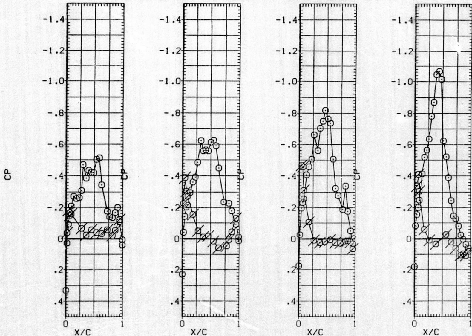
FIG. 15 PRESSURE DISTRIBUTIONS OVER CONFIGURATION 6 AT CTG=0.0
