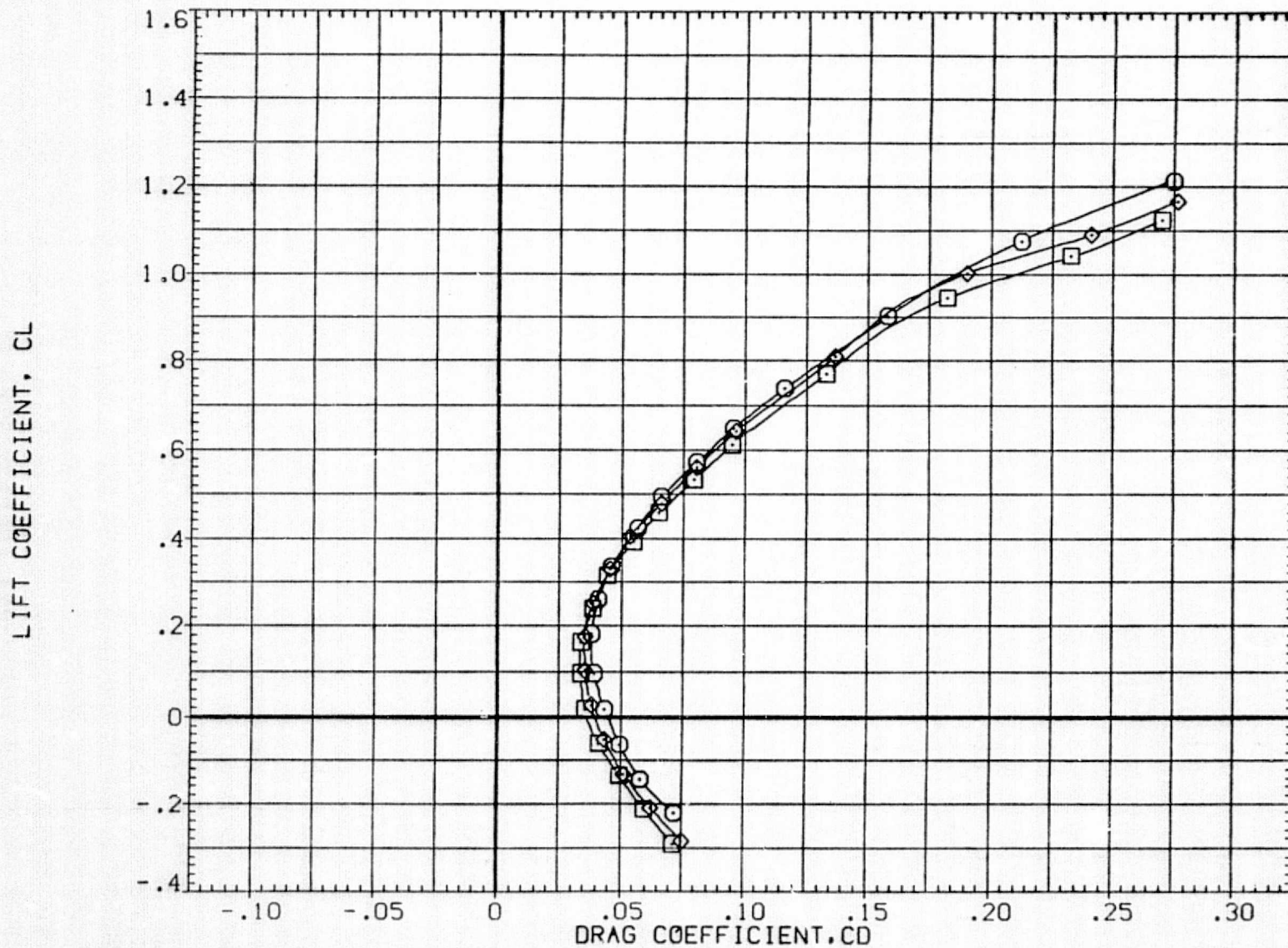
FIG. 14 FLAP EFFECTS WITH NO BLOWING (A) MACH = .95
