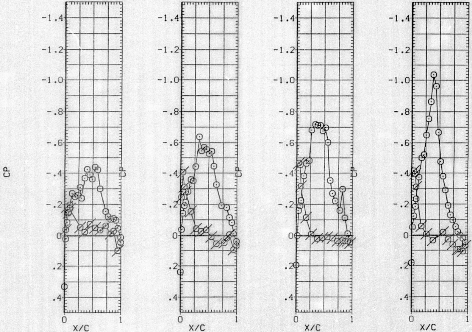
FIG. 15 PRESSURE DISTRIBUTIONS OVER CONFIGURATION 5 AT CTG=0.08
