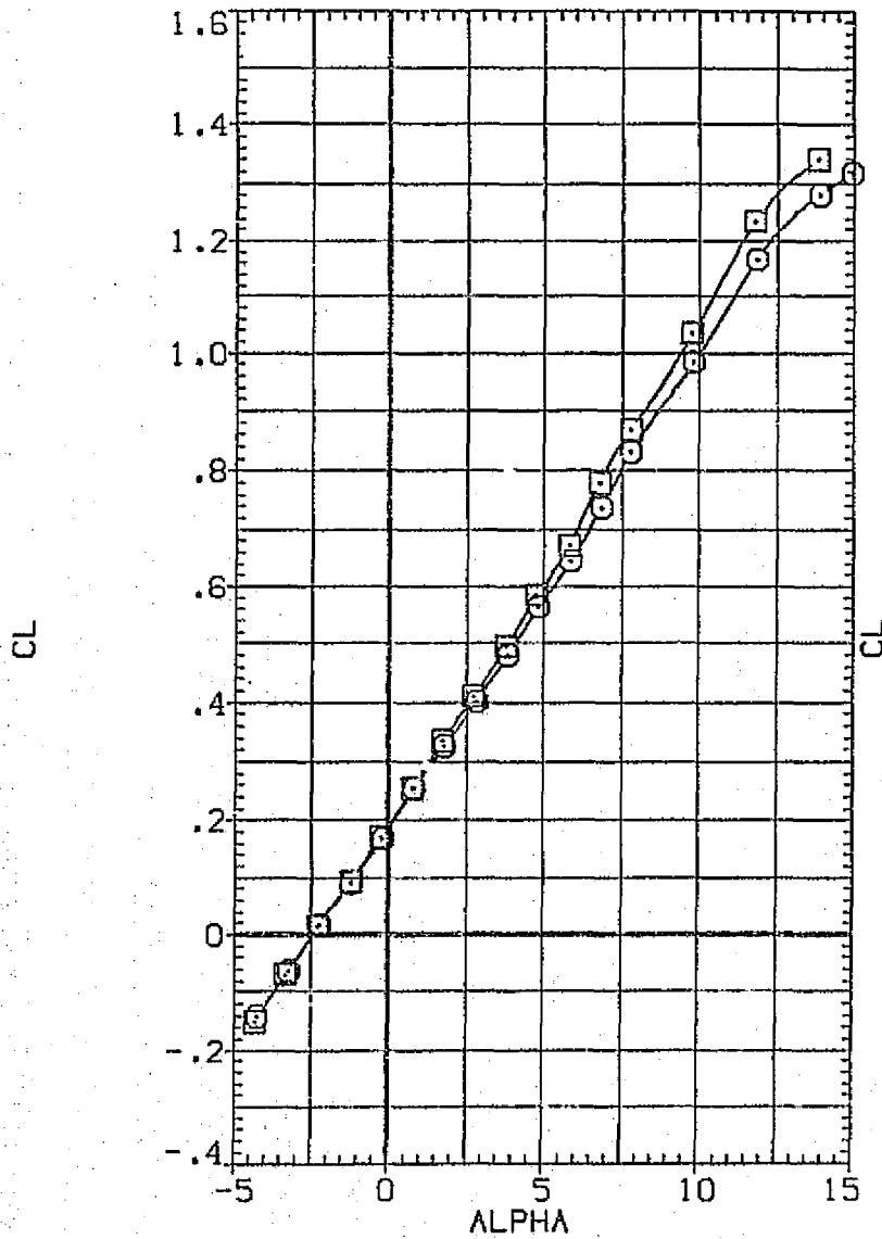
FIG. 12 REYNOLDS NUMBER SENSITIVITY WITH JET ON (B)MACH = .90
