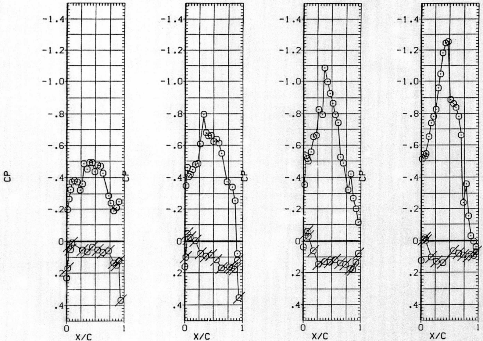
FIG. 15 PRESSURE DISTRIBUTIONS OVER CONFIGURATION 7 AT CTG=0.0
