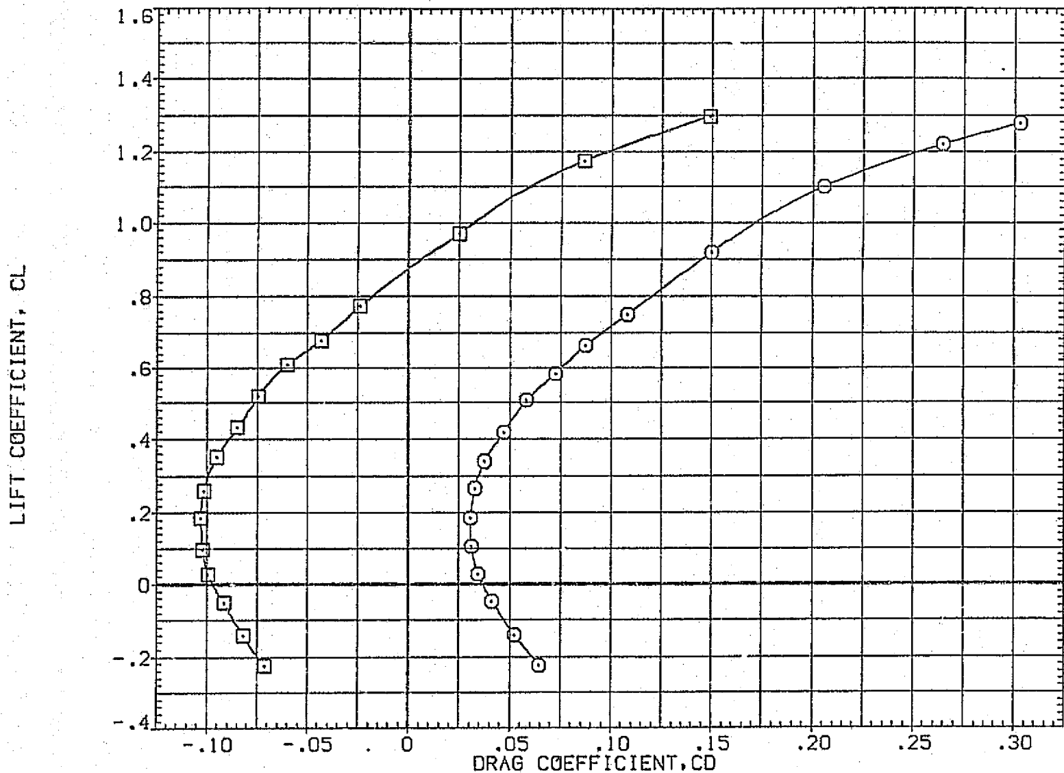
FIG. 13 EFFECTS OF BLOWING ON CONFIGURATION 3 (B)MACH = .90
