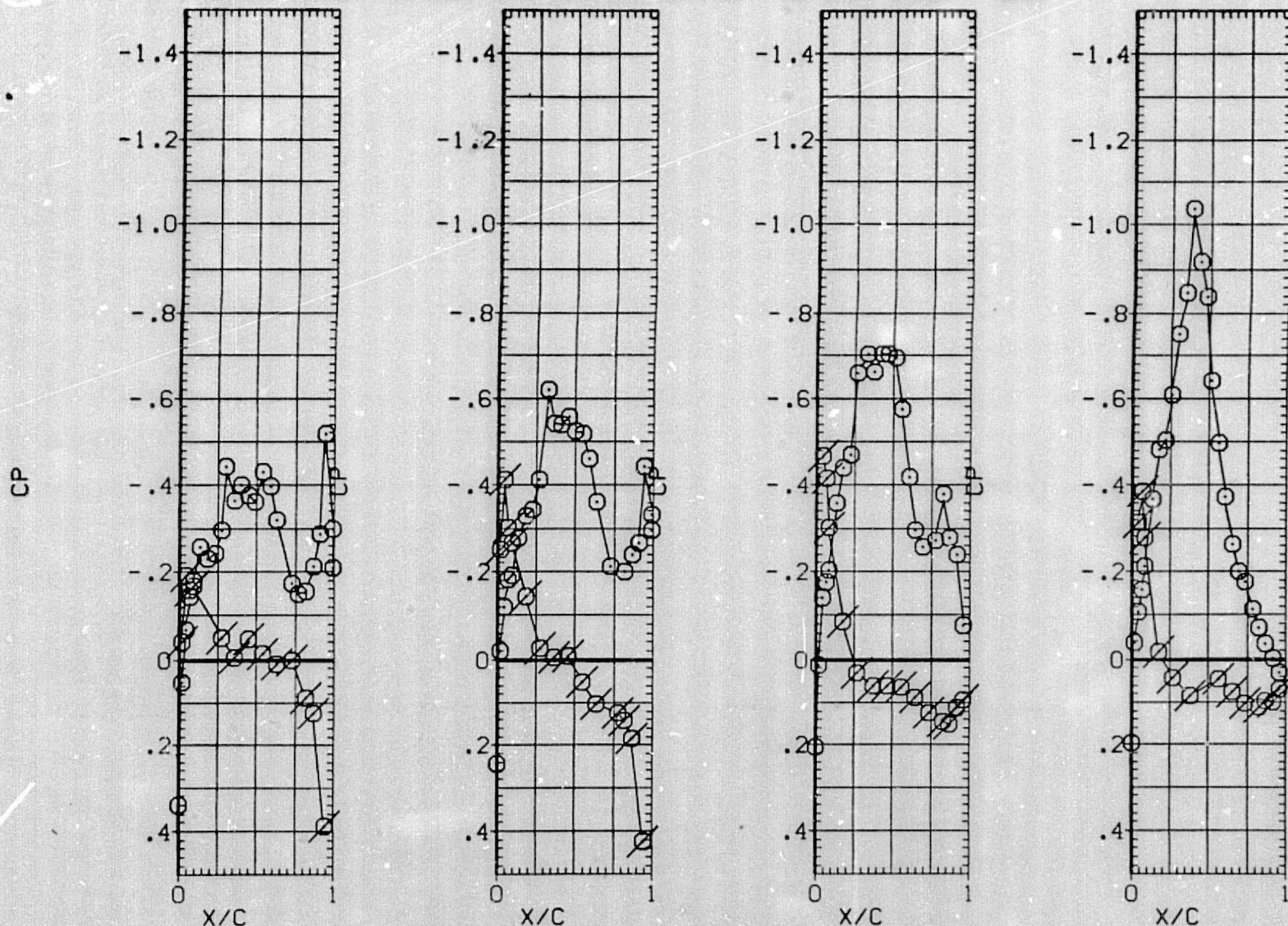
FIG. 15 PRESSURE DISTRIBUTIONS OVER CONFIGURATION 6 AT CTG=0.08
