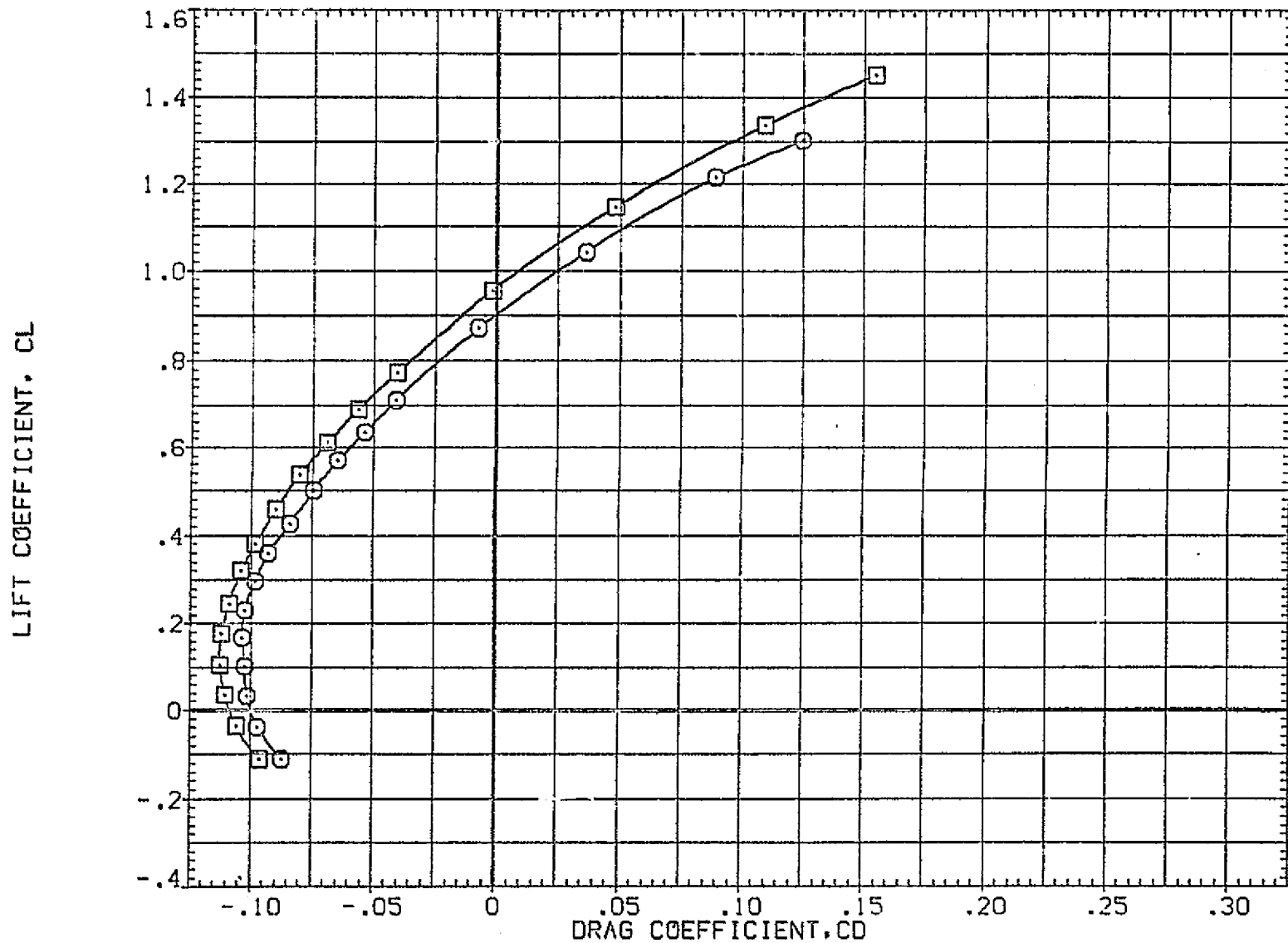
FIG. 12 REYNOLDS NUMBER SENSITIVITY WITH JET ON (A) MACH = .70
