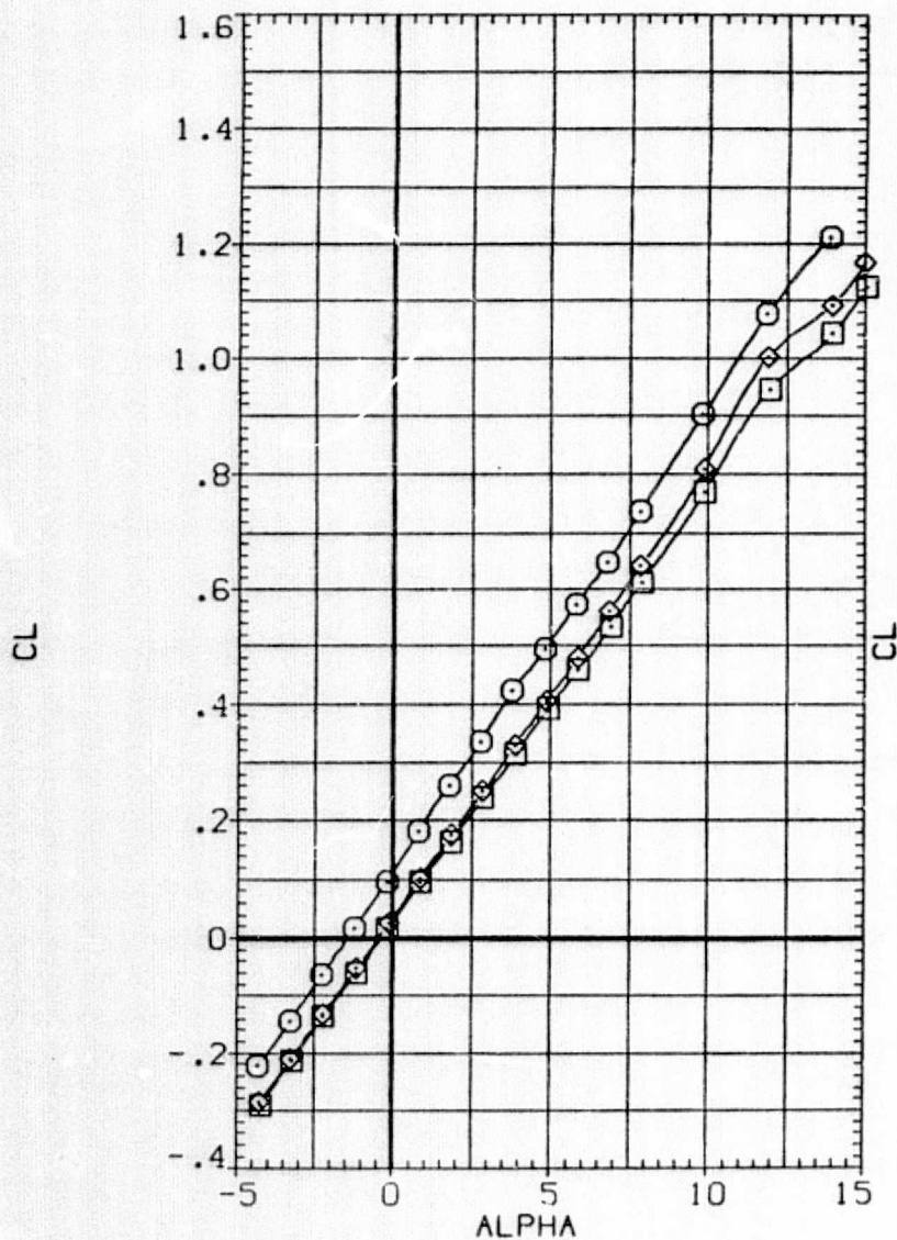
FIG. 14 FLAP EFFECTS WITH NO BLOWING
