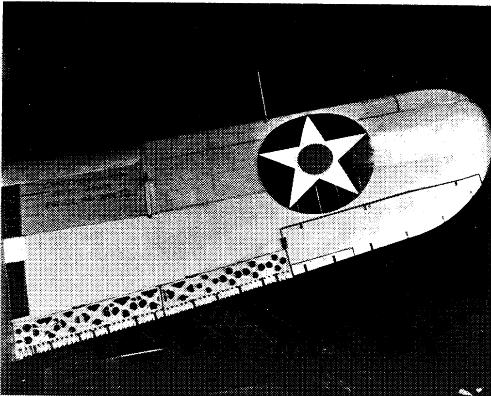
Figure C1.- Perforated flaps on airplane 6 (Brewster XSBA-1).
