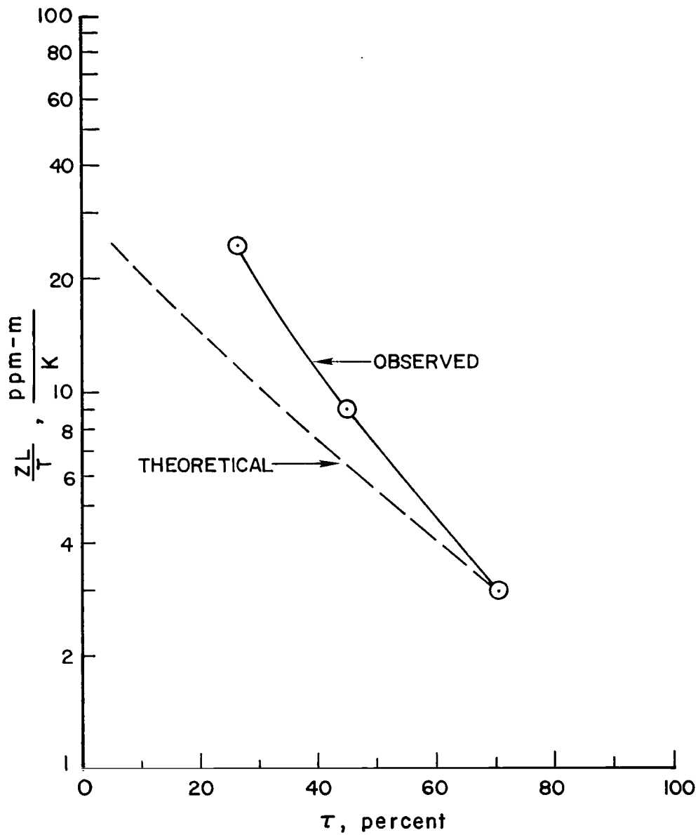
Figure 5.- Radiometer calibration for SO 2 .
