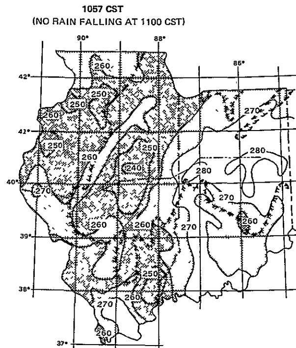
c) T_B ( ^{\circ} K) JUNE 3, 1973
