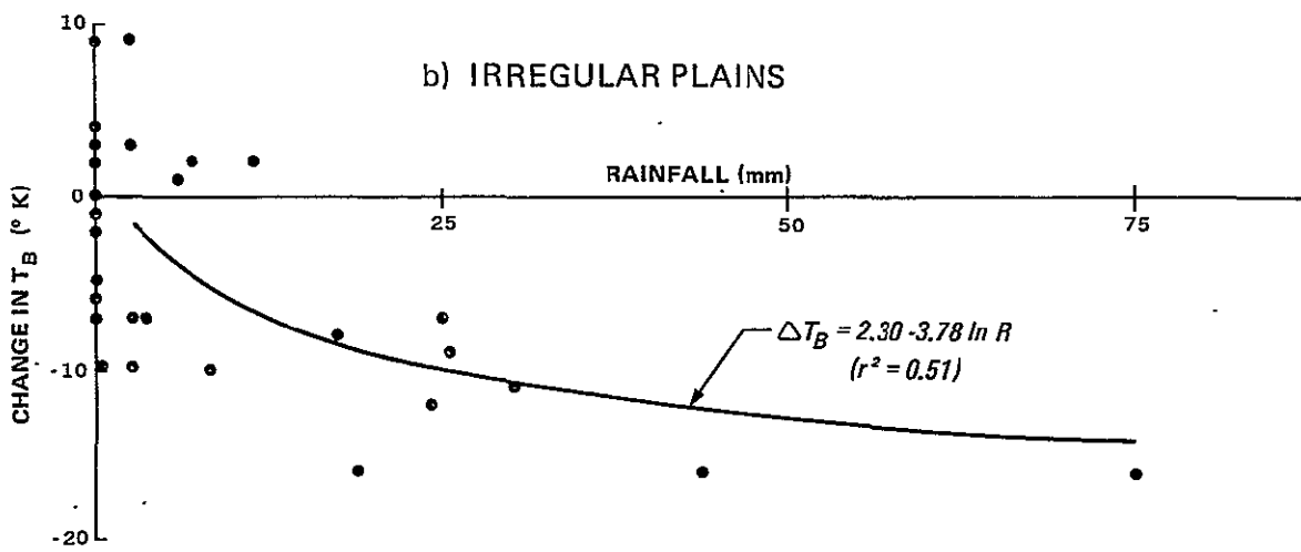
FIGURE 5. Effect of rainfall on brightness temperature for Event 2.
