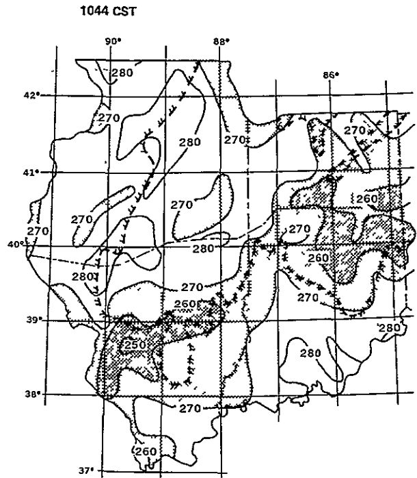
b) T_B ( ^{\circ} K) JUNE 8, 1973
