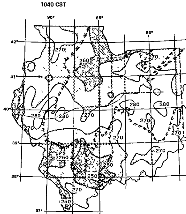
a) T_B ( ^{\circ} K) JUNE 1, 1973
