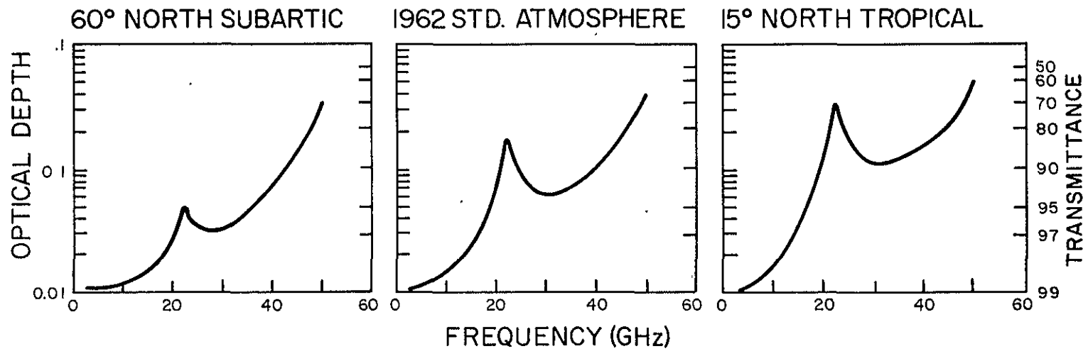
Figure 2. Optical depth of clear atmospheres. (After Westwater, 1972)
