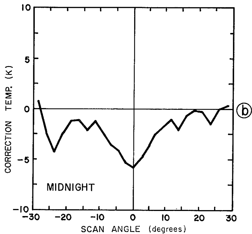
Figure 11. Scan angle correction temperatures, (a) noon correction, (b) midnight correction.
