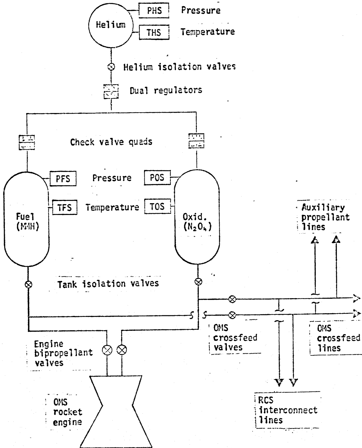
Figure 3. - Shuttle OMS baseline pressurant/propellant system and instrumentation.
