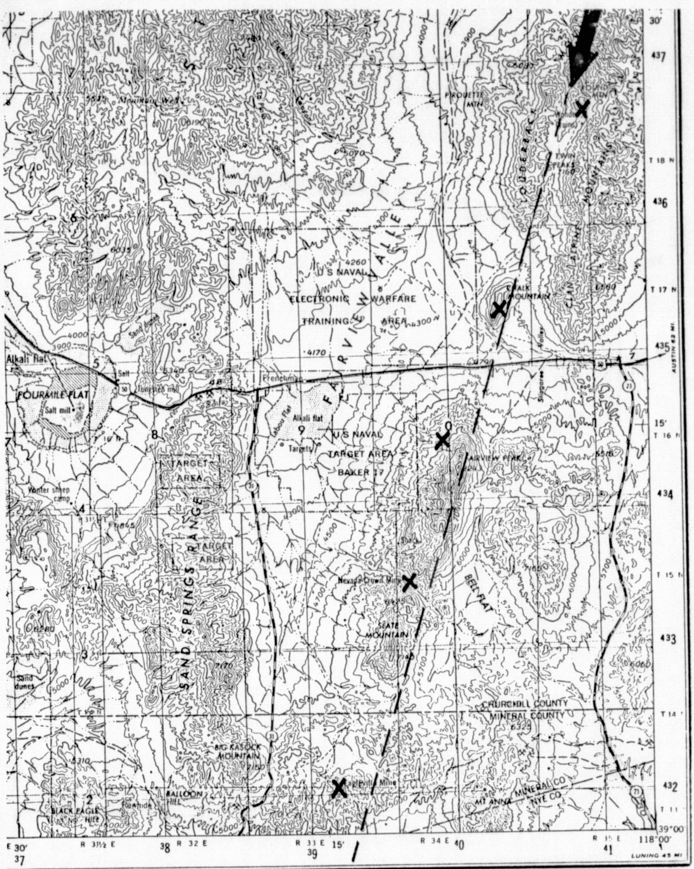
Fig. 2 Southeastern portion of Army Map Service NJ 11-1 Reno AMS topo sheet showing location of 5 mining areas (crosses) and Landsat trend (arrow and dashed line).
