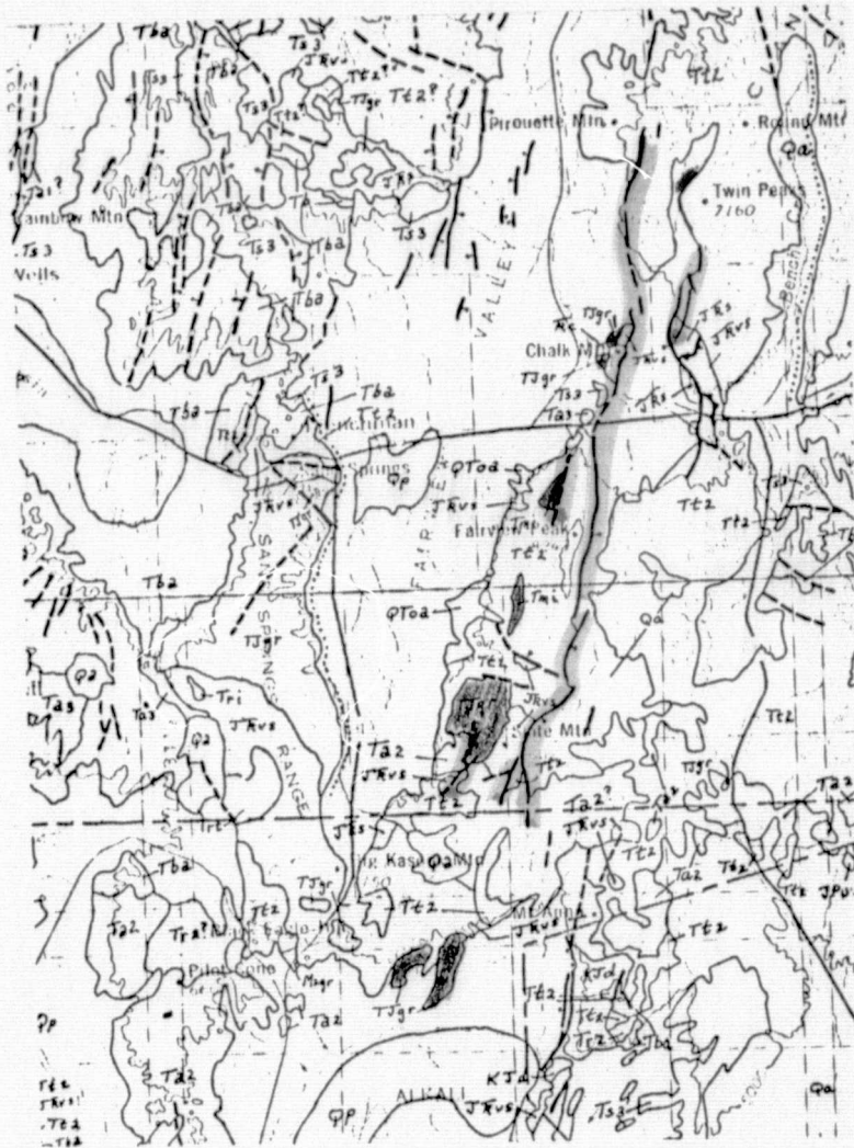
Fig. 3 Portion of Preliminary Geologic Map of Nevada (Stewart and Carlson, 1974) showing NNE alignment of intrusive bodies (red) and faults (blue) along Wonder-Eagleville mining trend, Mineral and Churchill counties, Nevada.
