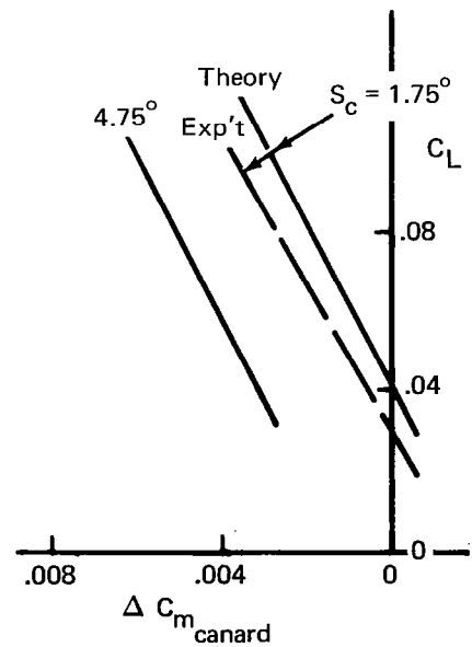
FIGURE 4.4-12.—EFFECT OF CANARD DOWNWASH SHIFT ~ M = 2.7
