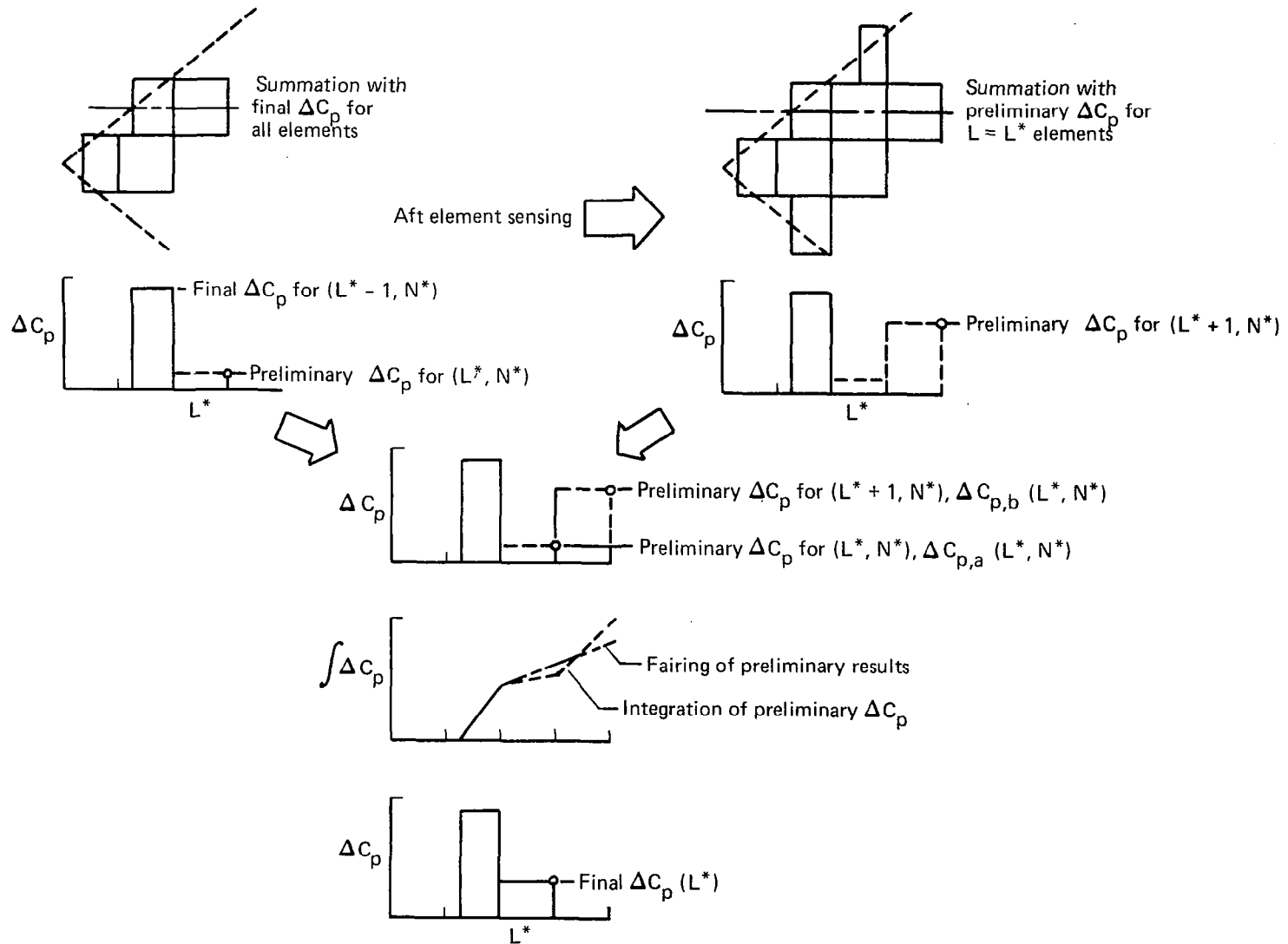
FIGURE 4.4-7.—APPLICATION OF AFT-ELEMENT SMOOTHING TECHNIQUE (FROM REF. 12)
