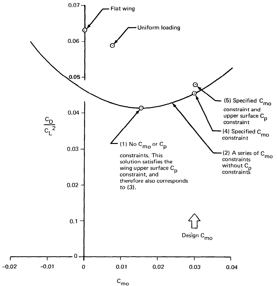
FIGURE 4.4-5.—TYPES OF LOADING SOLUTIONS
