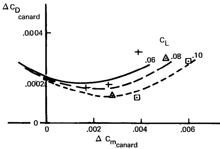
FIGURE 4.4-12.—EFFECT OF CANARD DOWNWASH SHIFT ~ M = 2.7
