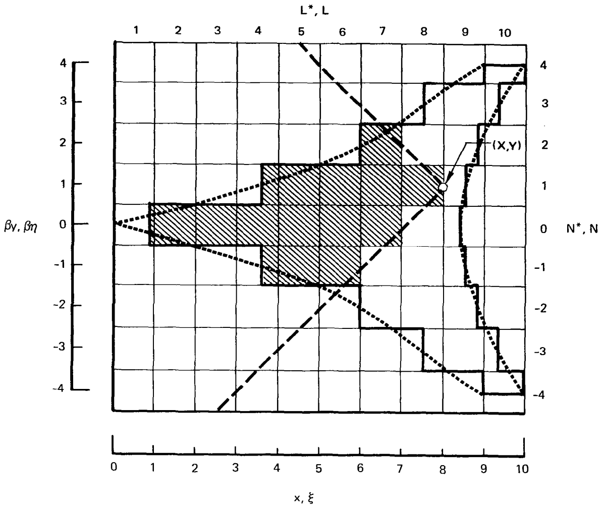
FIGURE 4.4-2.— GRID SYSTEM USED IN NUMERICAL SOLUTION
