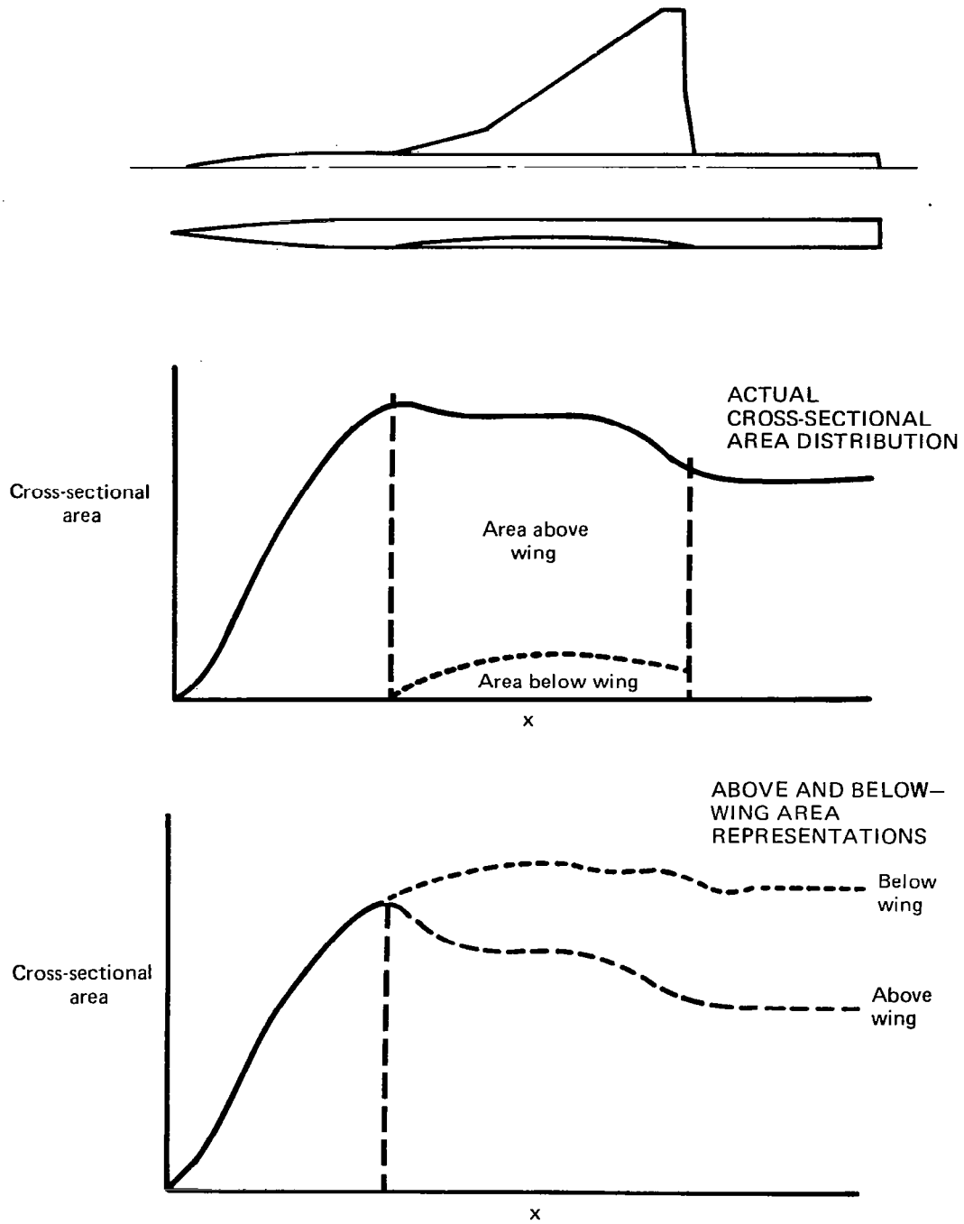
FIGURE 4.4-9.— FUSELAGE AREA REPRESENTATION FOR ASYMMETRIC FUSELAGE BUOYANCY FIELD
