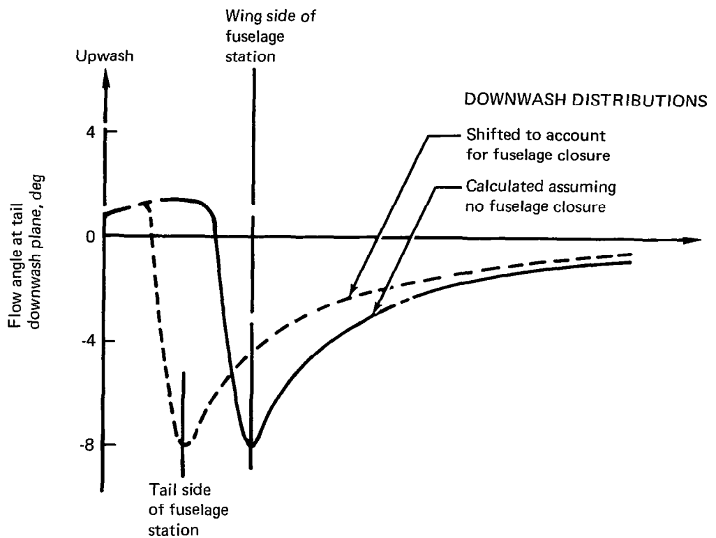
FIGURE 4.4-11.—DOWNWASH PATH CORRECTION
