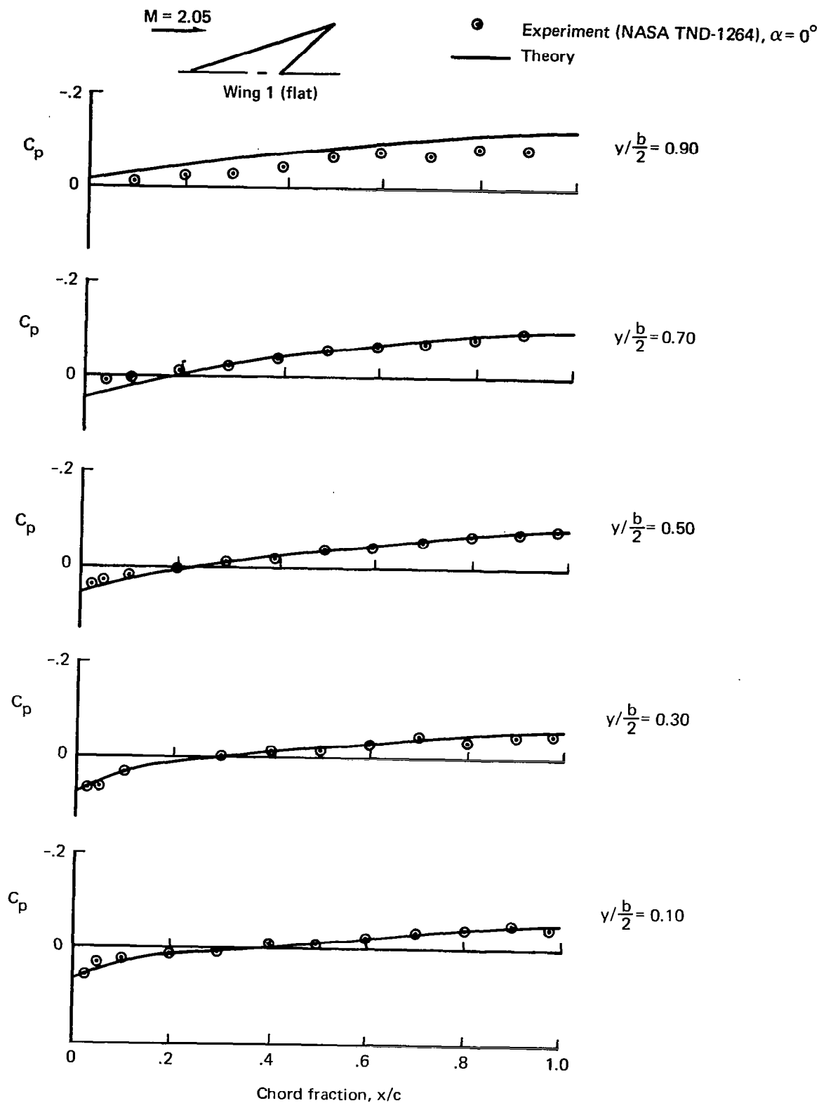
FIGURE 44-14.— THICKNESS PRESSURE COMPARISON ( C_p DUE TO THICKNESS ONLY)
