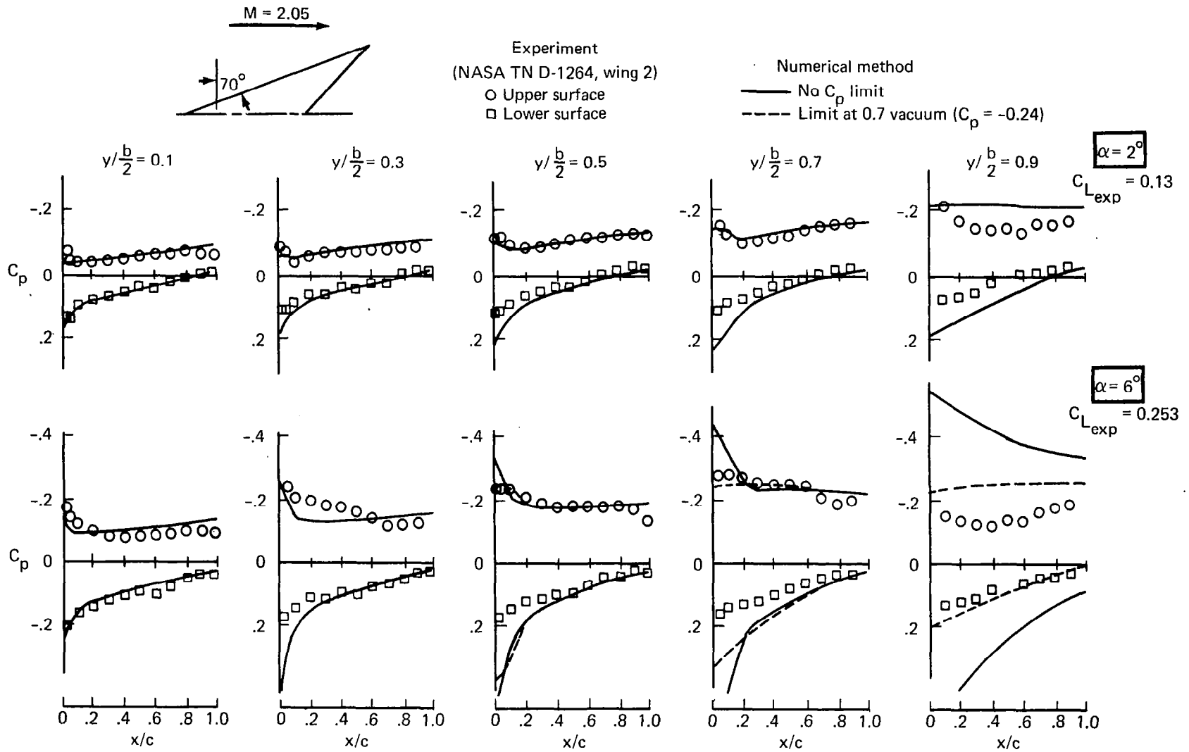
FIGURE 4.4-16. -PRESSURE COEFFICIENT COMPARISON, WING 2 (TWISTED AND CAMBERED WING, DESIGN C_L = .08 )
