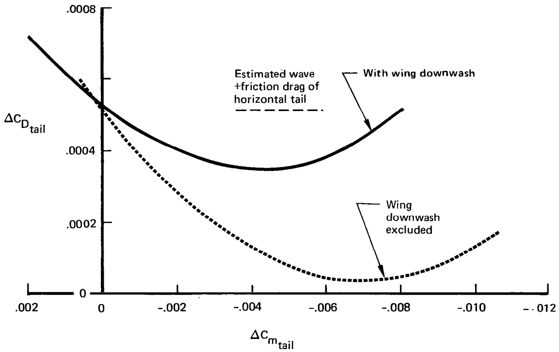
FIGURE 4.4-10.—EFFECT OF WING DOWNWASH ON TAIL (THEORETICAL ESTIMATE)
