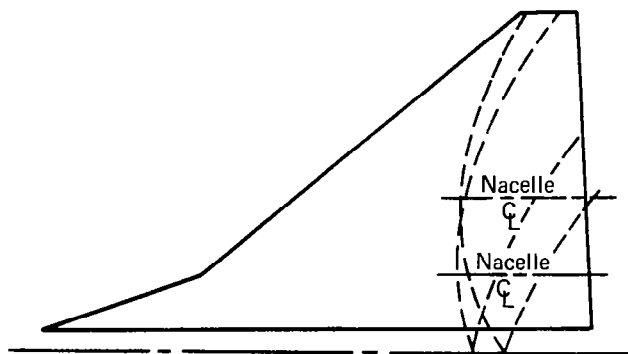
FIGURE 4.3-7.—NACELLE GENERATED WING PRESSURE FIELD CONCEPTS
