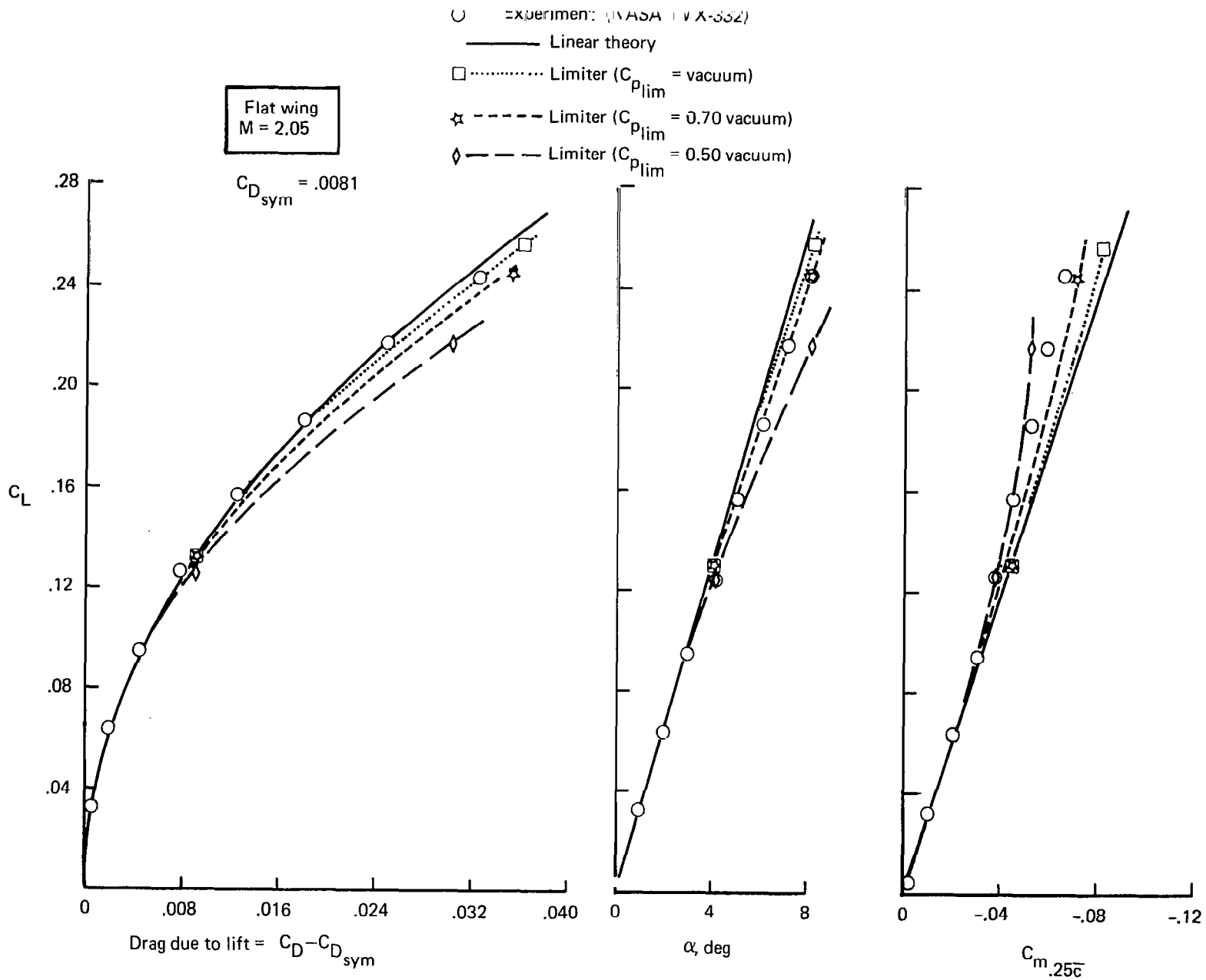
FIGURE 4.4-17. -TEST-THEORY COMPARISON, WING 1 (FLAT WING)
