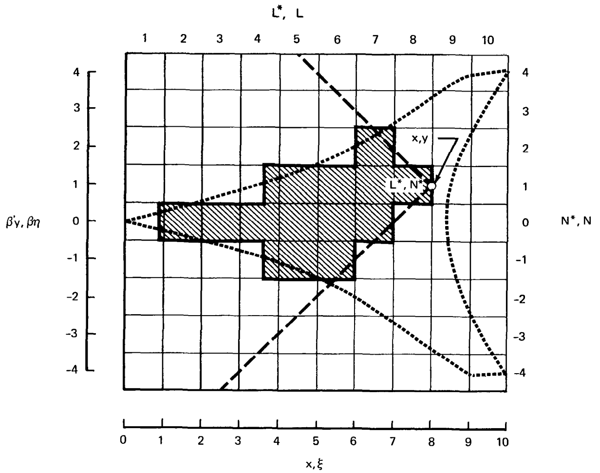
FIGURE 4.3-1.—WING COORDINATE SYSTEM
