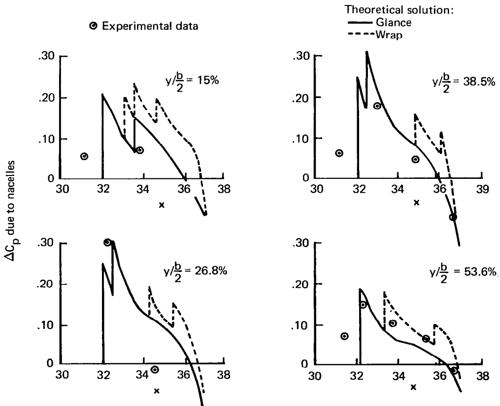
FIGURE 4.3-9.—NACELLE PRESSURE FIELD DATA, M = 1.1
