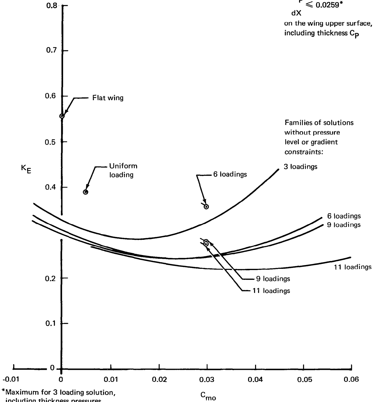
FIGURE 4.4-6.—WING DESIGN STUDY: CONSTRAINTS ON BOTH C_{m0} AND UPPER SURFACE PRESSURE GRADIENT
