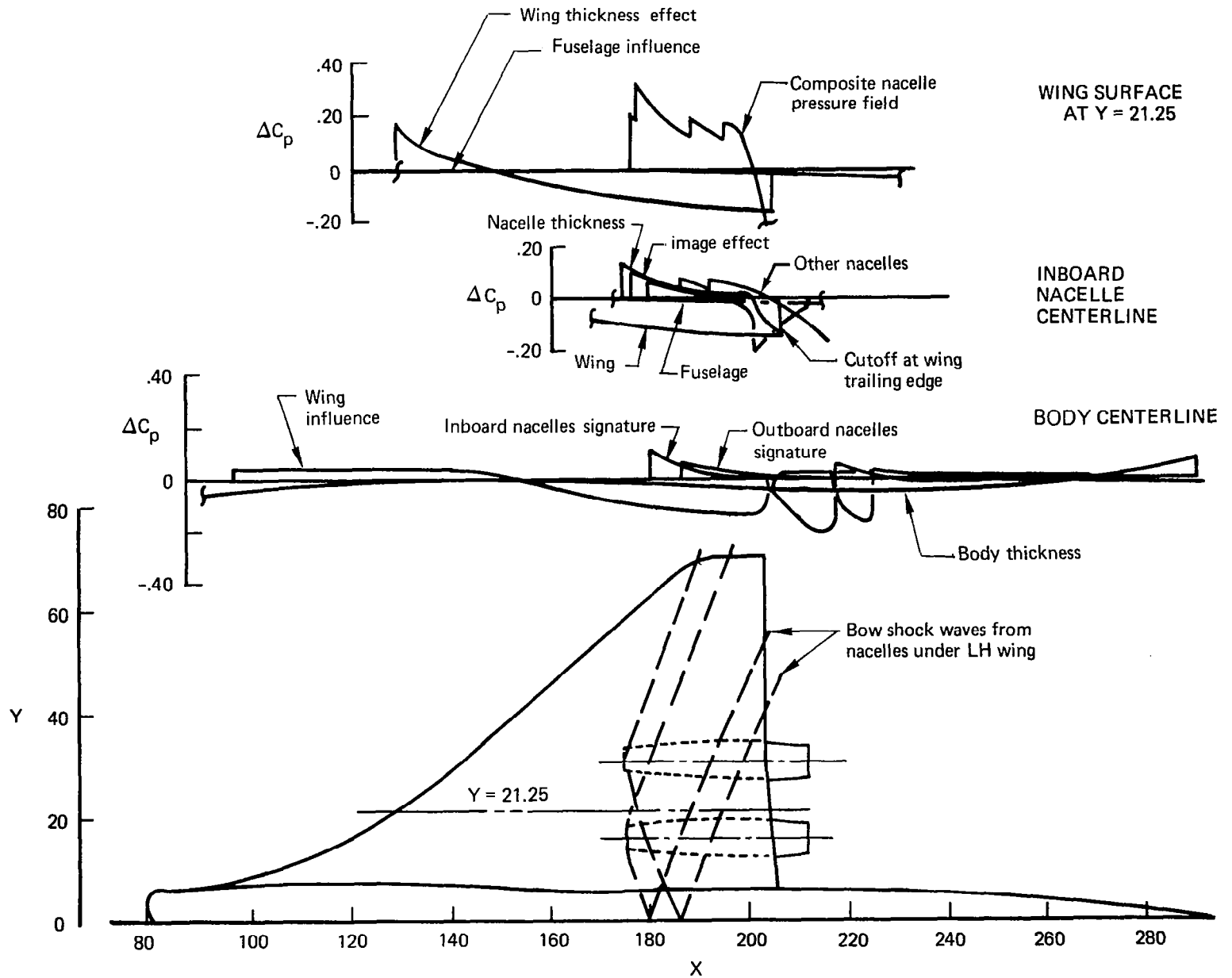
FIGURE 4.3-10.—NEAR-FIELD PRESSURE SIGNATURES, M = 1.1 "WRAP" SOLUTION
