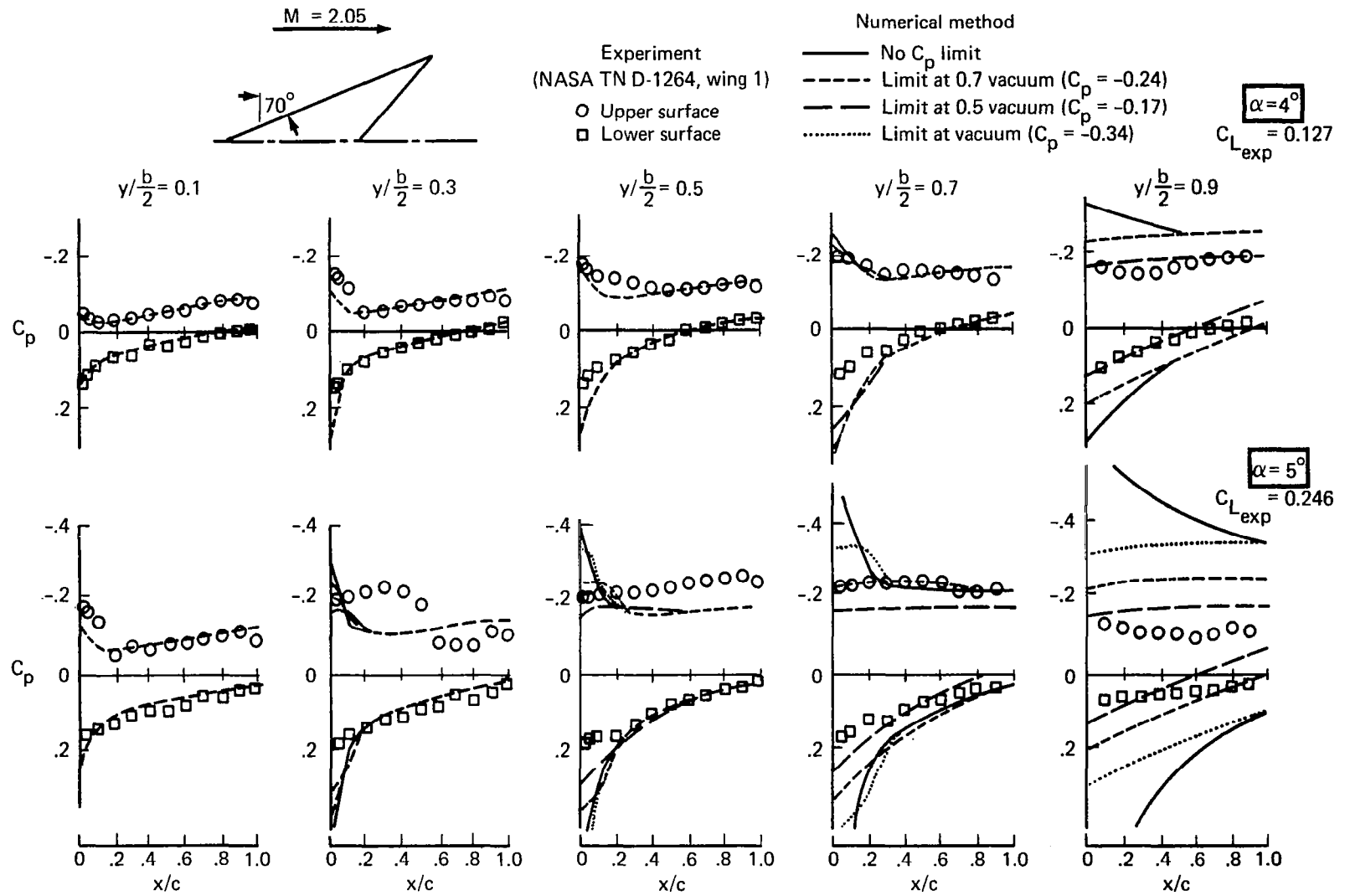
FIGURE 44-15. — PRESSURE COEFFICIENT COMPARISON, WING 1 (FLAT WING)
