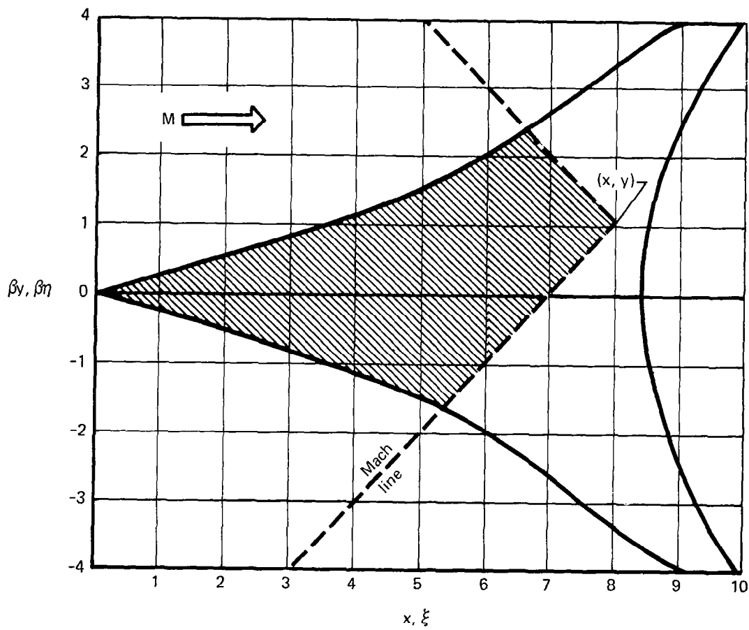
FIGURE 4.4-1.—CARTESIAN COORDINATE SYSTEM
