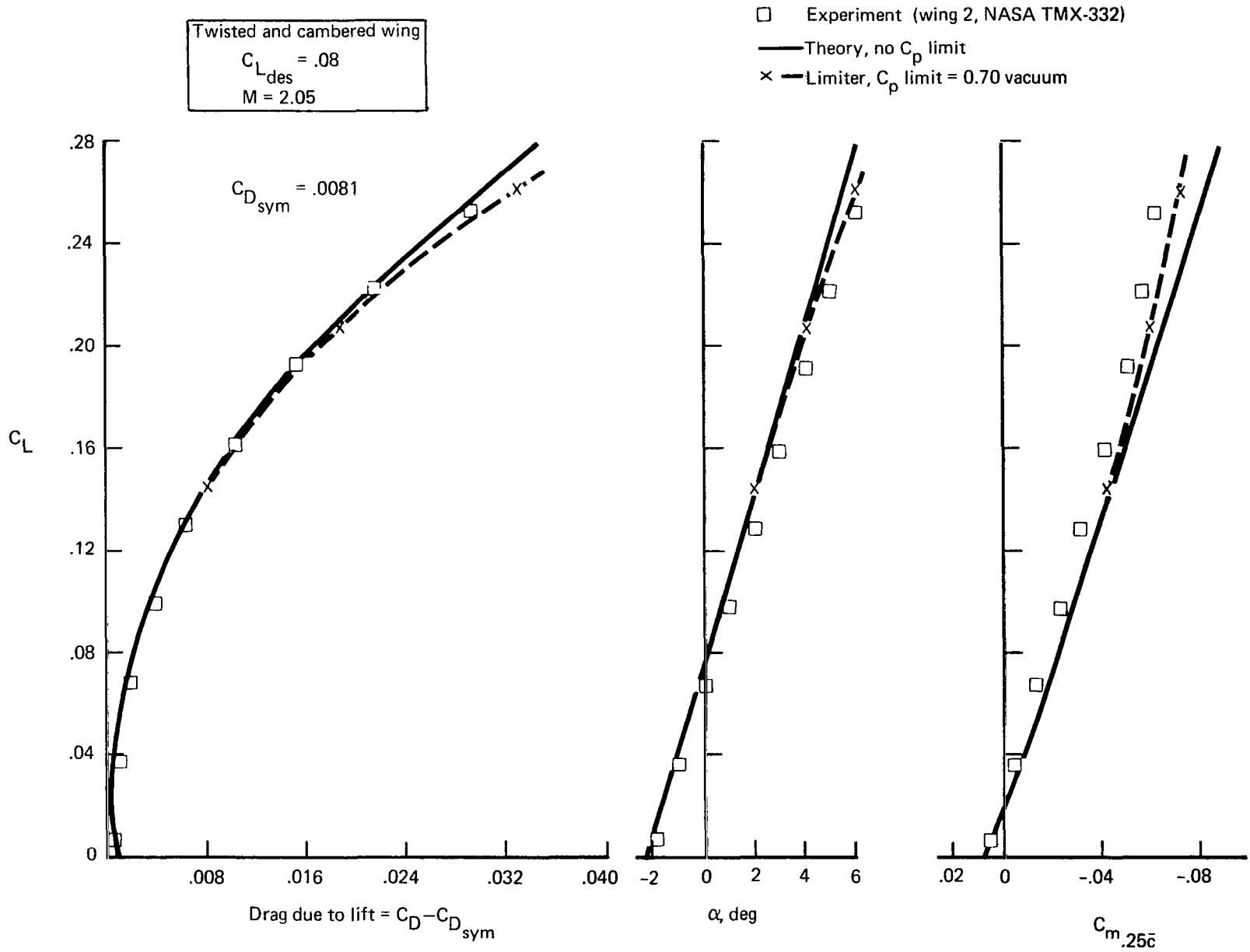
FIGURE 44-18. -TEST-THEORY COMPARISON, WING 2 ( C_{L_{des}} = 0.08 )
