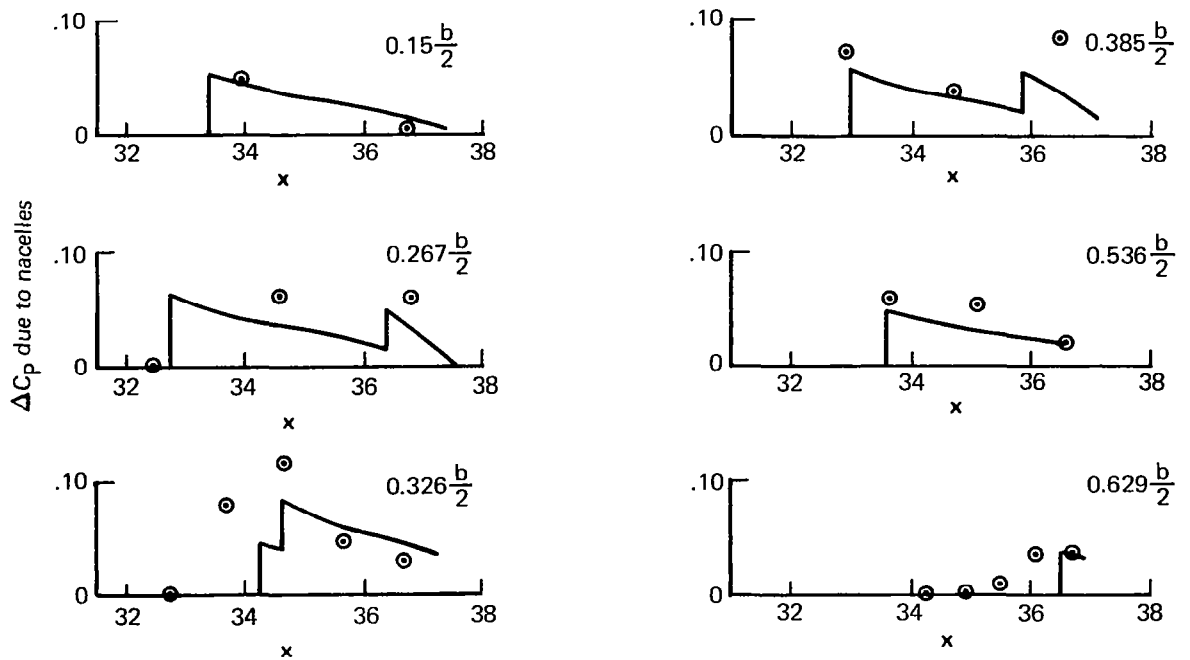
FIGURE 4.3-8.—NACELLE PRESSURE FIELD DATA, M = 2.7
