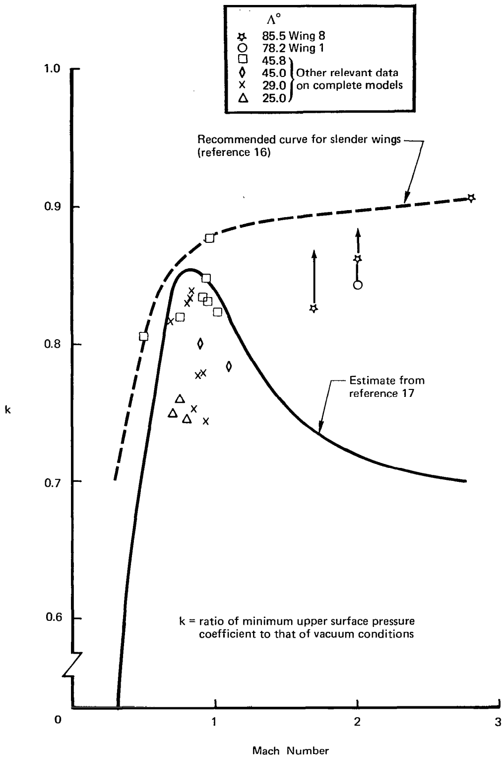
FIGURE 4.4-13.—MINIMUM ATTAINABLE PRESSURE COEFFICIENTS (FROM REF. 16)
