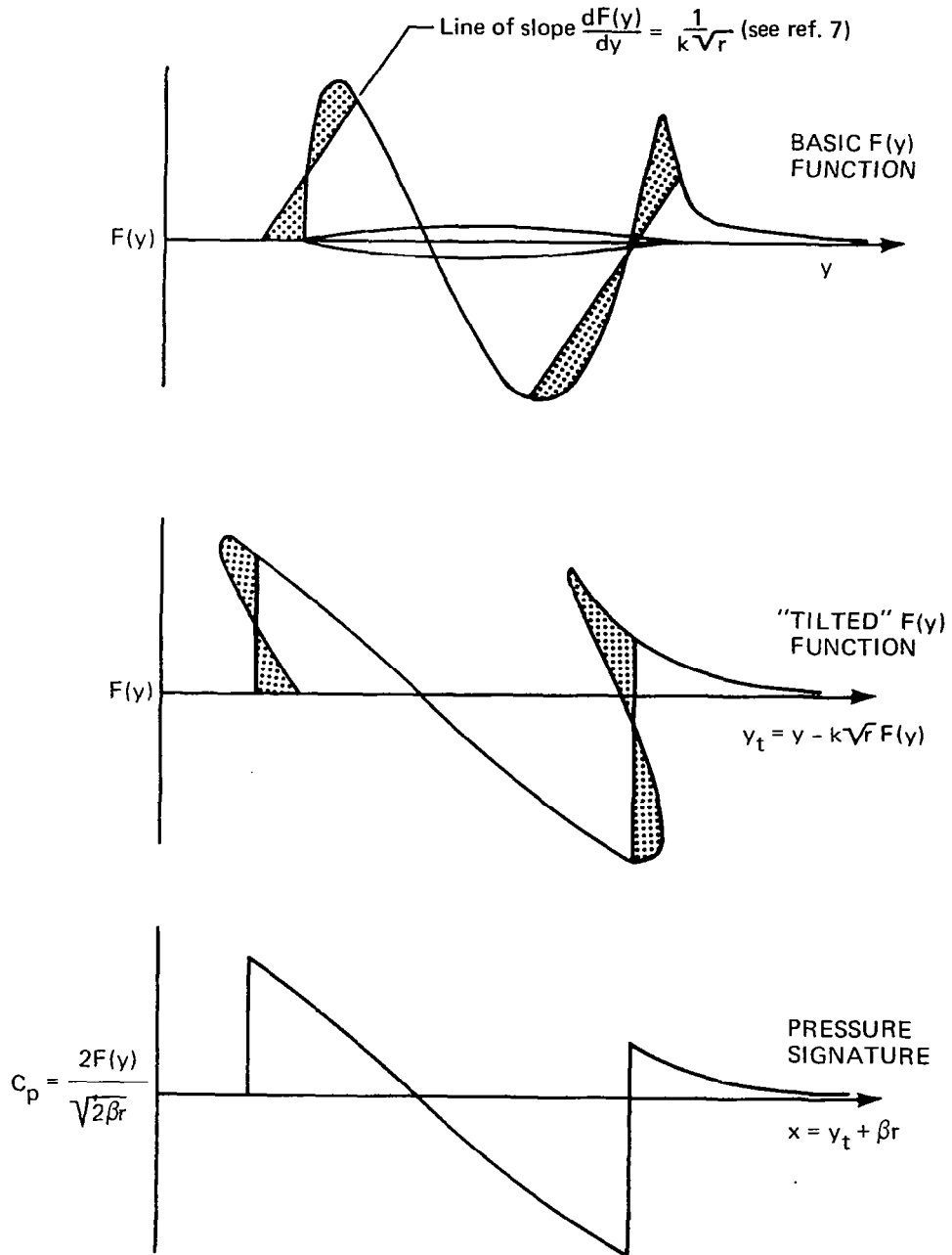
FIGURE 4.3-5.—DEVELOPMENT OF NEAR-FIELD PRESSURE SIGNATURE
