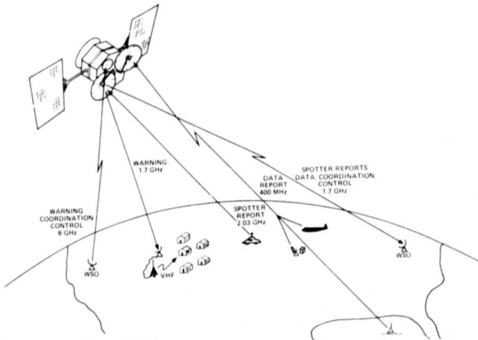
Figure 18. Hybrid System Concept
