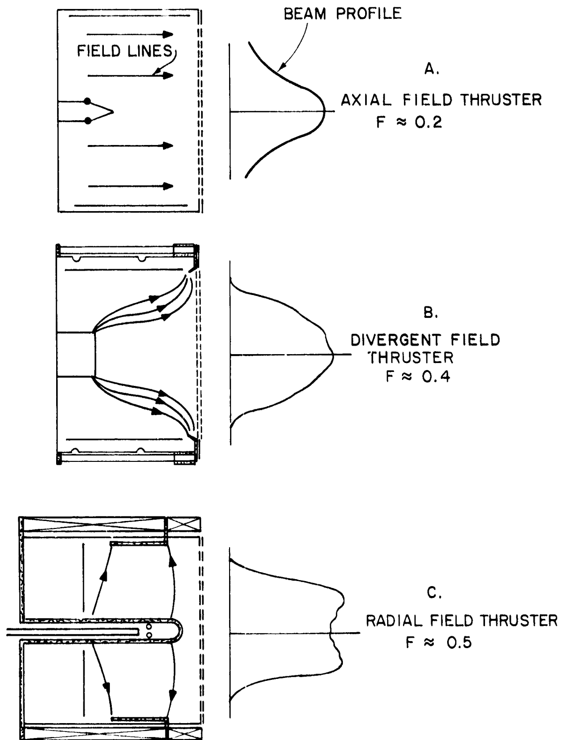
Figure 5. Axial, divergent, and radial field discharge chambers and their associated beam current density profiles.
