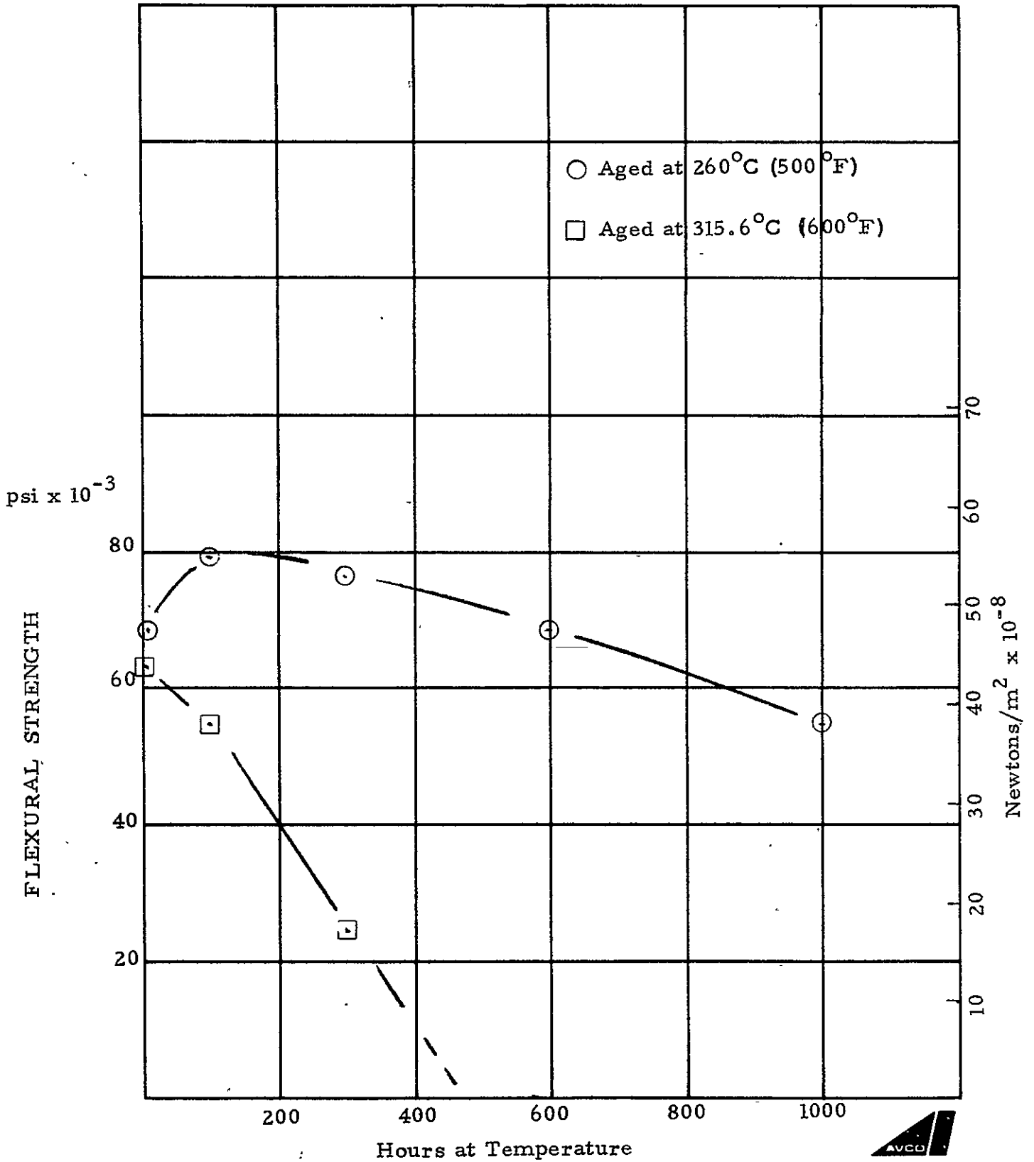
Figure 31. Effect of Aging at Elevated Temperatures on the Flexural Strength of Polymer I/Graphite Composite.
