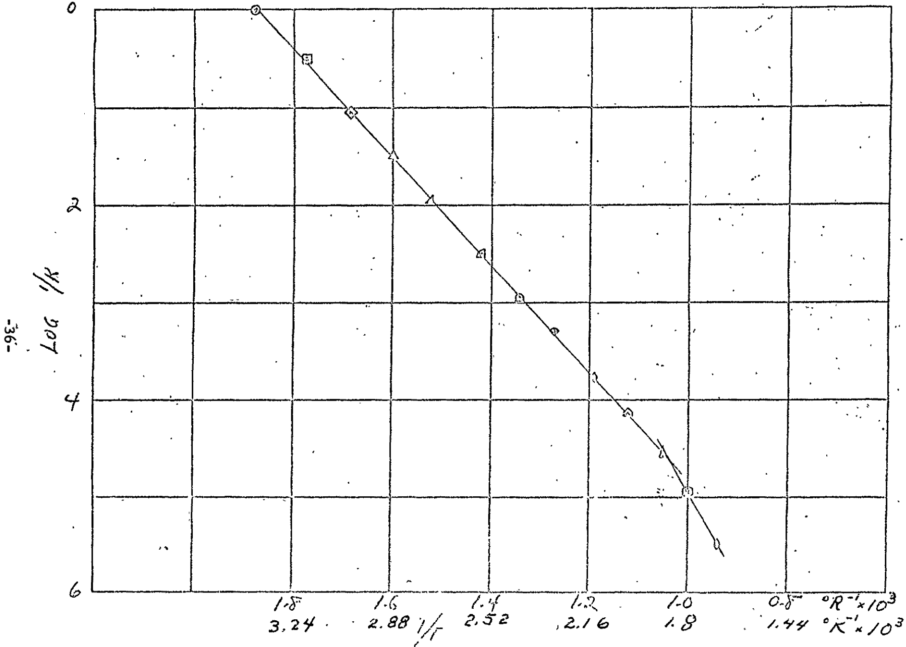
Figure 18. Determination of Second-Order Transition Temperature from Log 1/K vs. 1/T Plot for Polymer I.
