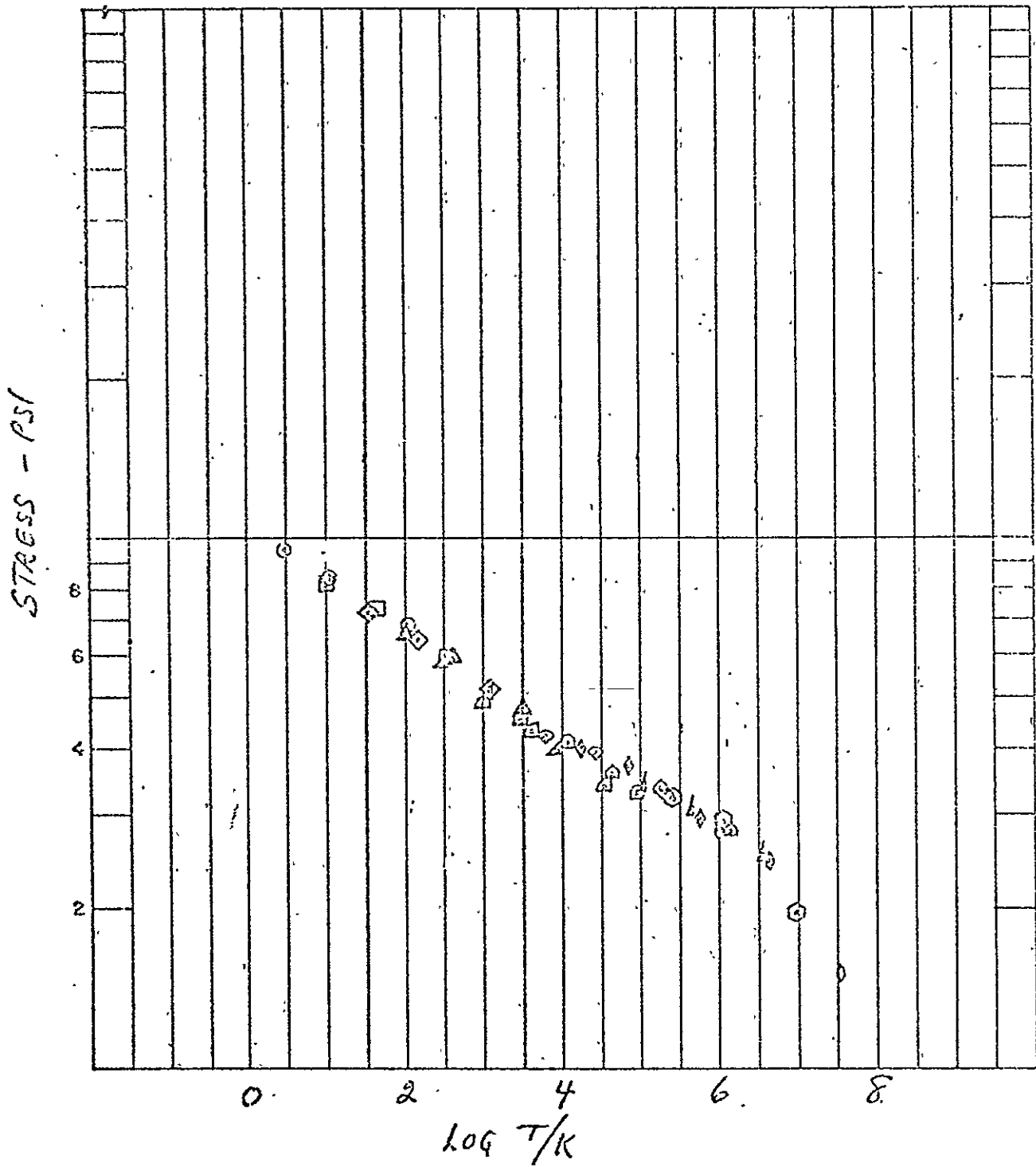
Figure 17. Master Curve for Polymer I.
