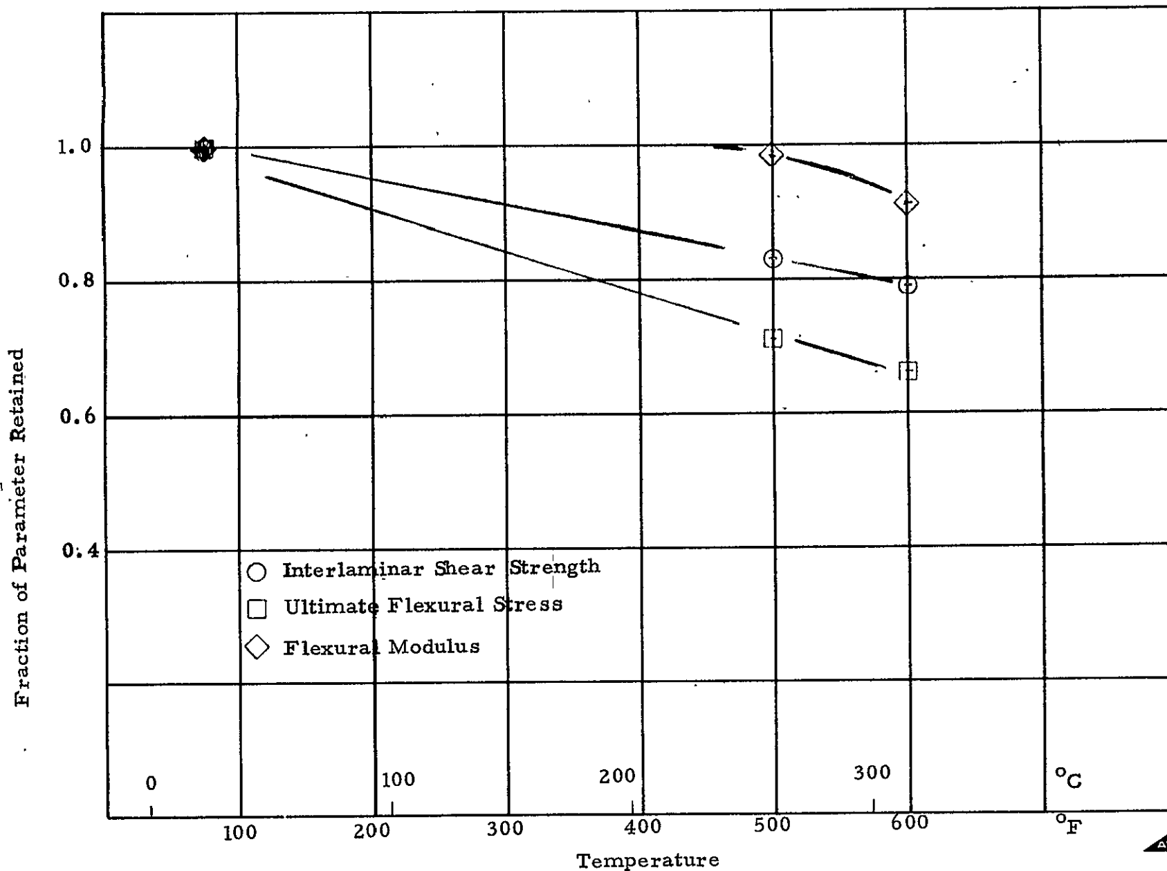
Figure 35. Effect of Temperature on the Fraction of the Value of Mechanical Properties Parameters Retained.
