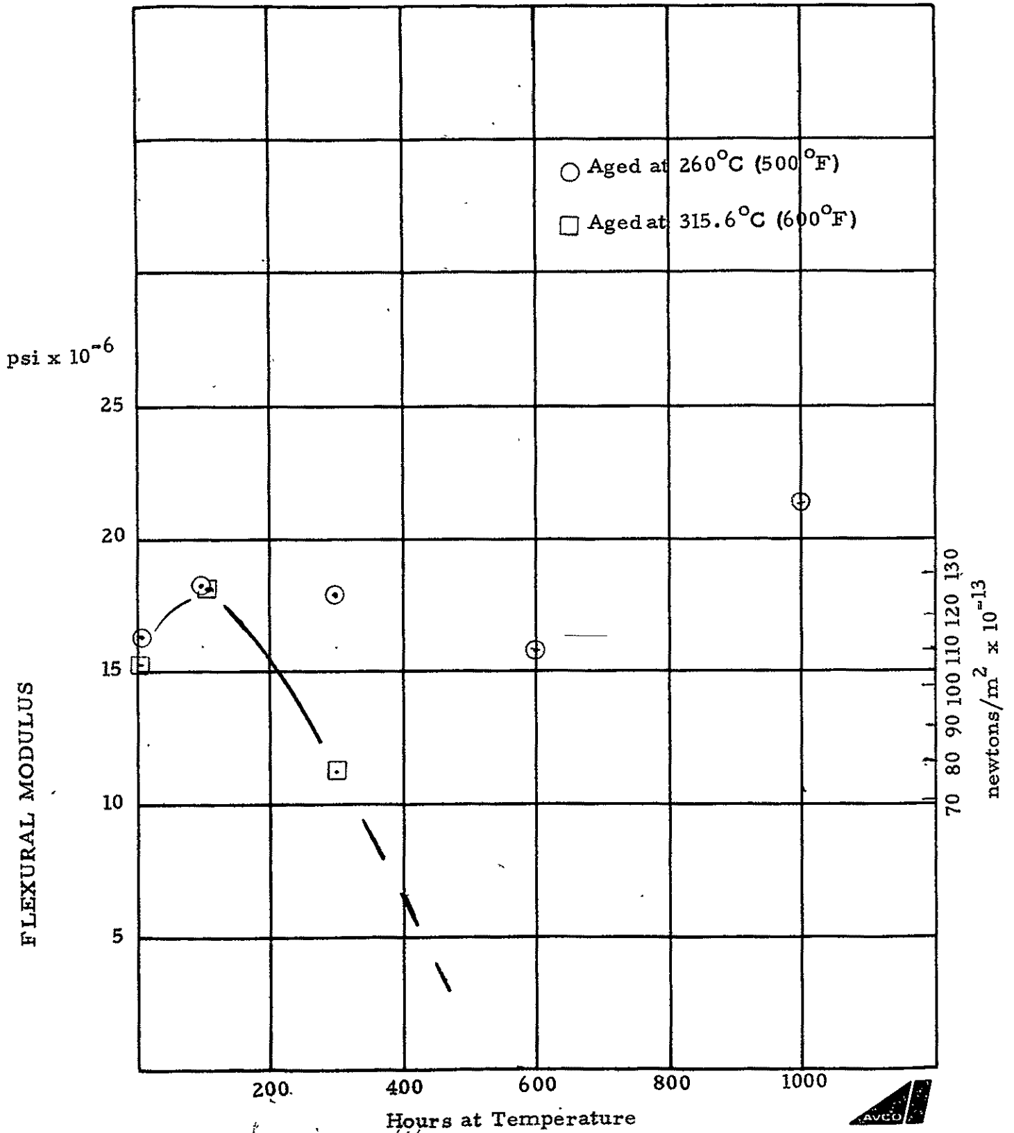
Figure 32. Effect of Aging at Elevated Temperatures on the Flexural Modulus of Polymer I/Graphite Composite.
