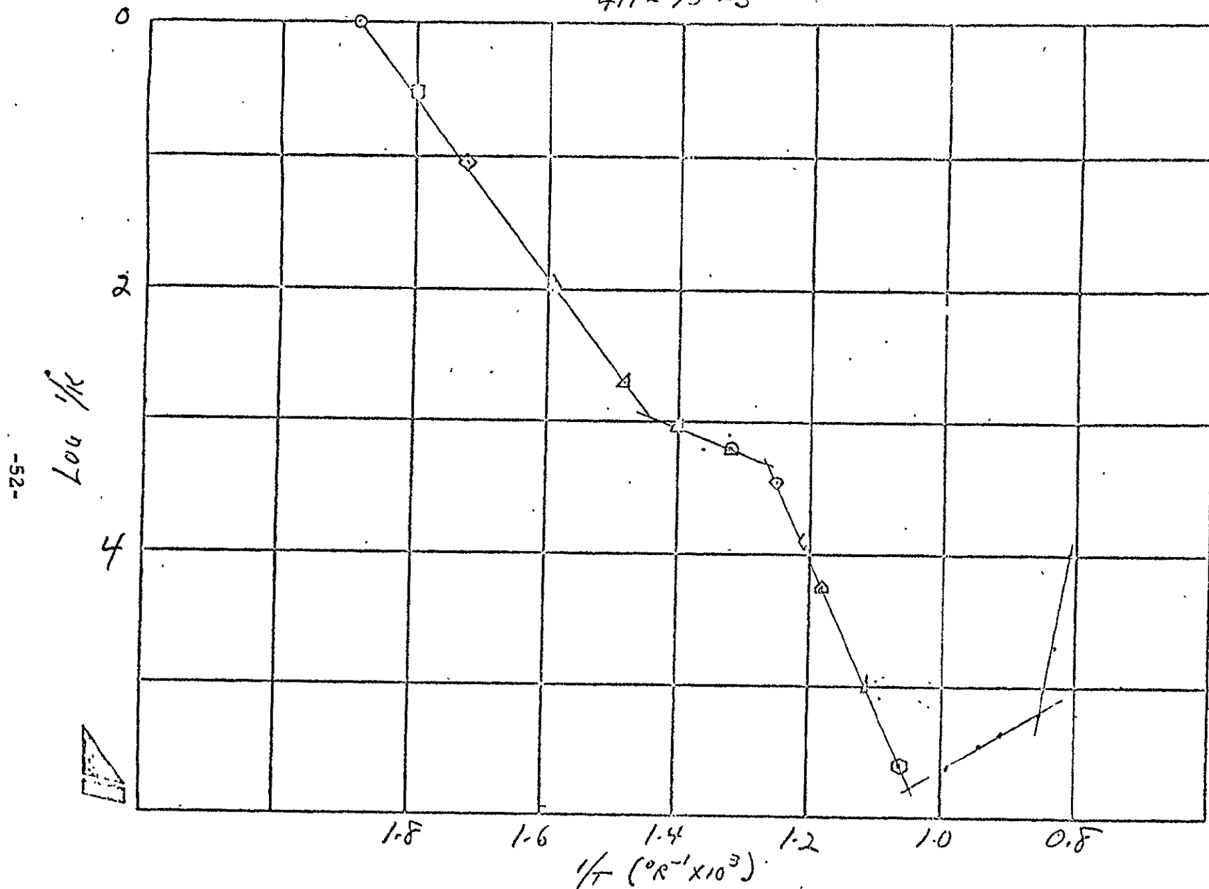
Figure 39. Determination of Second-Order Transition Temperature from \log 1/K vs. 1/T Plot for "Crosslinked" Polymer I.
