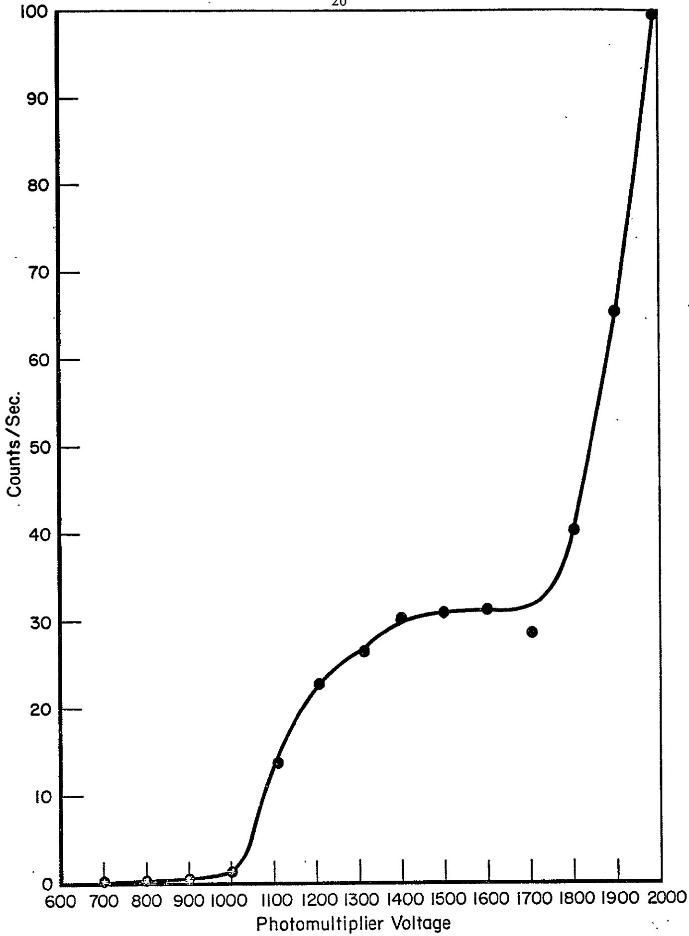
FIGURE 3. PHOTOMULTIPLIER DARK CURRENT VS APPLIED VOLTAGE REPRODUCED FROM THE ORIGINAL PAGE IS POOR
