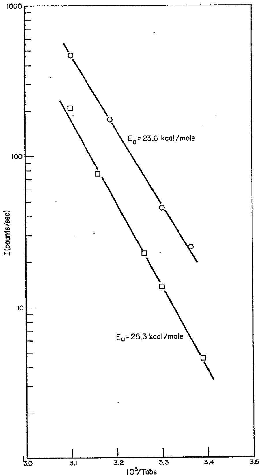
FIGURE 40. CHEMILUMINESCENCE AS A FUNCTION OF TEMPERATURE FOR AUTOXIDIZED ( \square ) AND SINGLET OXYGENATED ( \circ ) CIS-1,4-POLYISOPRENE. EACH RUN CONTAINED 0.5 PERCENT 9,10-DIPHENYLANTHRACENE.
