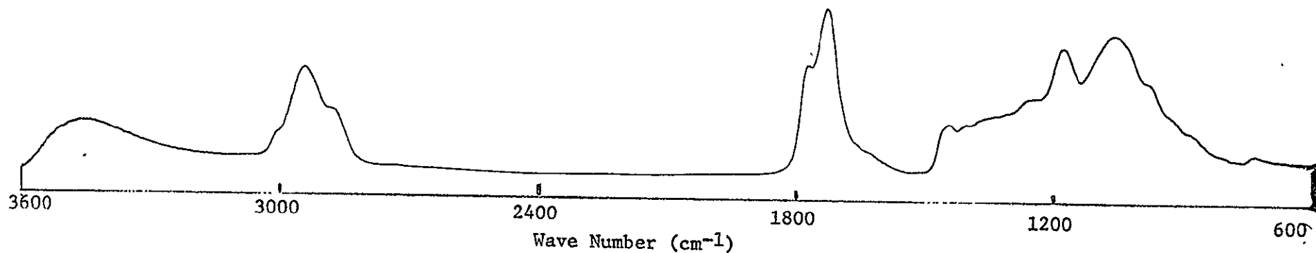
FIGURE 10. SAMPLE NO. 3 AFTER 21 MINUTES : cis-1,4-POLYBUTADIENE IN OXYGEN AT 115°C
