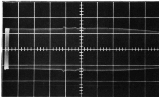
Figure 4: Oscilloscope traces showing peak-to-peak output (mV) from reference transducer E as a function of frequency (kHz) for three quantities of balls, as described in the text. The top trace shows the source-transducer combination as being overdamped; the center trace, underdamped; and the bottom trace, near optimum damping. The vertical scale is 20 mV peak-to-peak per division, and the horizontal scale is 0.3 kHz per division. The left-hand edge of each trace begins at 35 Hz; the sweep range is 3 kHz.
