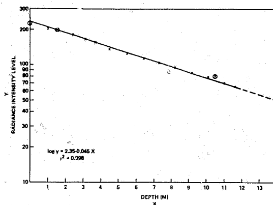
Figure 4. OCS-4 depth determination, 0 to 12 m, on September 19, 1975, off the west coast of Florida. The circled x's indicate three points which can be determined selectively from the radiance-distribution patterns and used to approximate this line.
