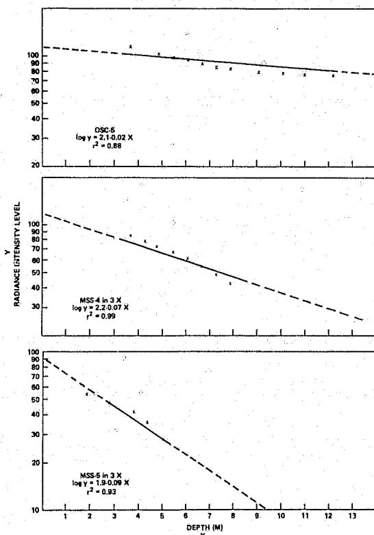
Figure 3. Comparison of OCS-5, MSS-4 in high-gain mode, and MSS-5 in high-gain mode for depth determination on September 19, 1975, off the west coast of Florida.
