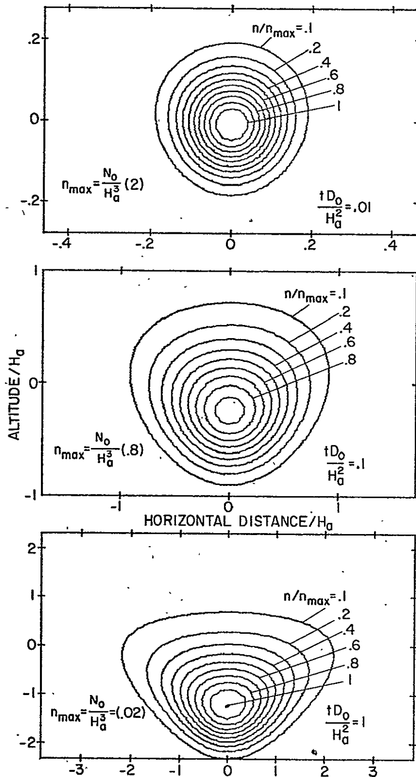
Fig. 2. Expansion of a gas cloud in a nonuniform atmosphere. The cloud becomes highly nonspherical after expanding over many scale heights. An expanding H_2 cloud containing N_0 molecules is released into an atmosphere with scale height H_a . The diffusion coefficient at the release point is D_0 .
