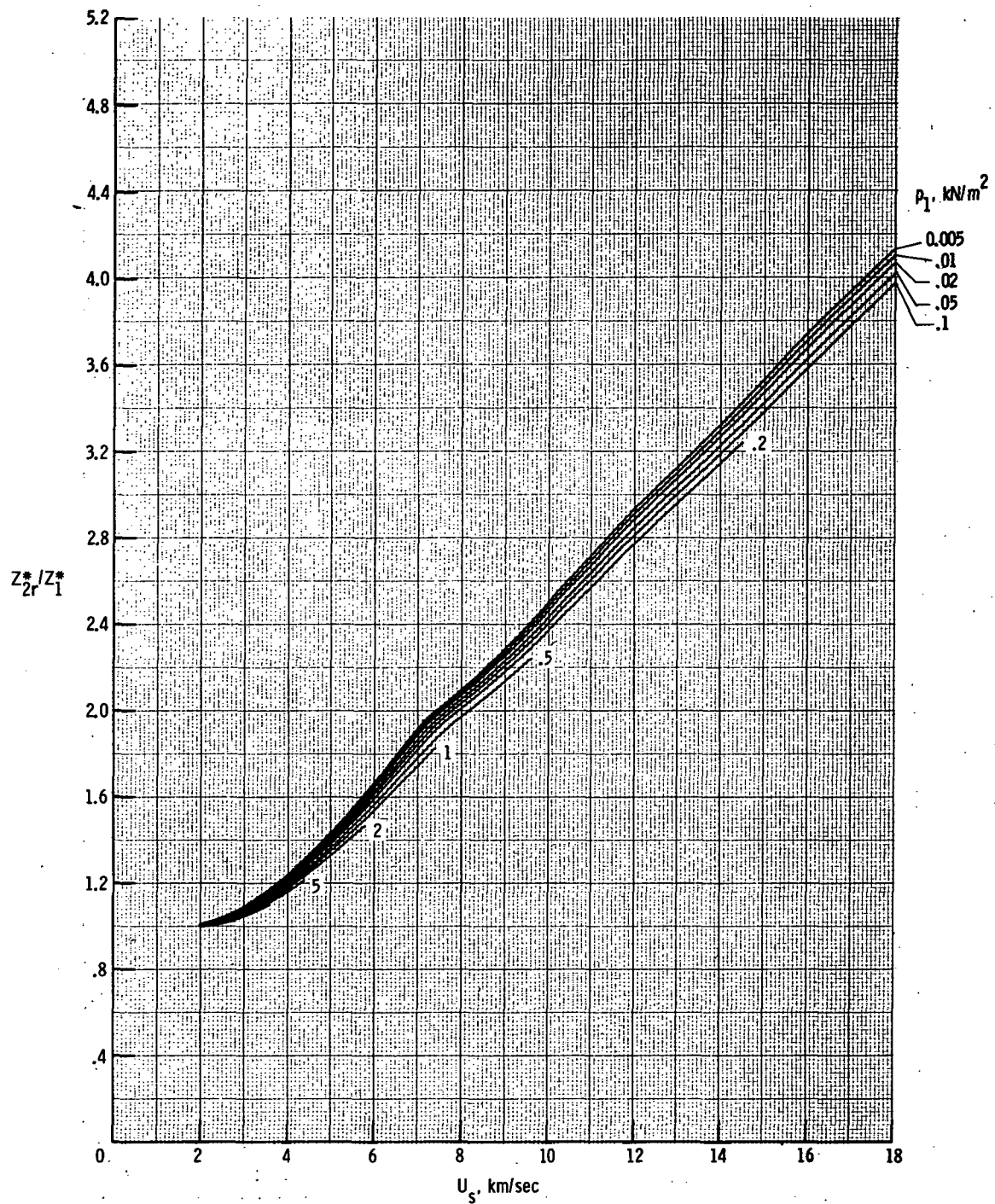
(g) Molecular-weight ratio Z_{2r}^*/Z_1^* .
