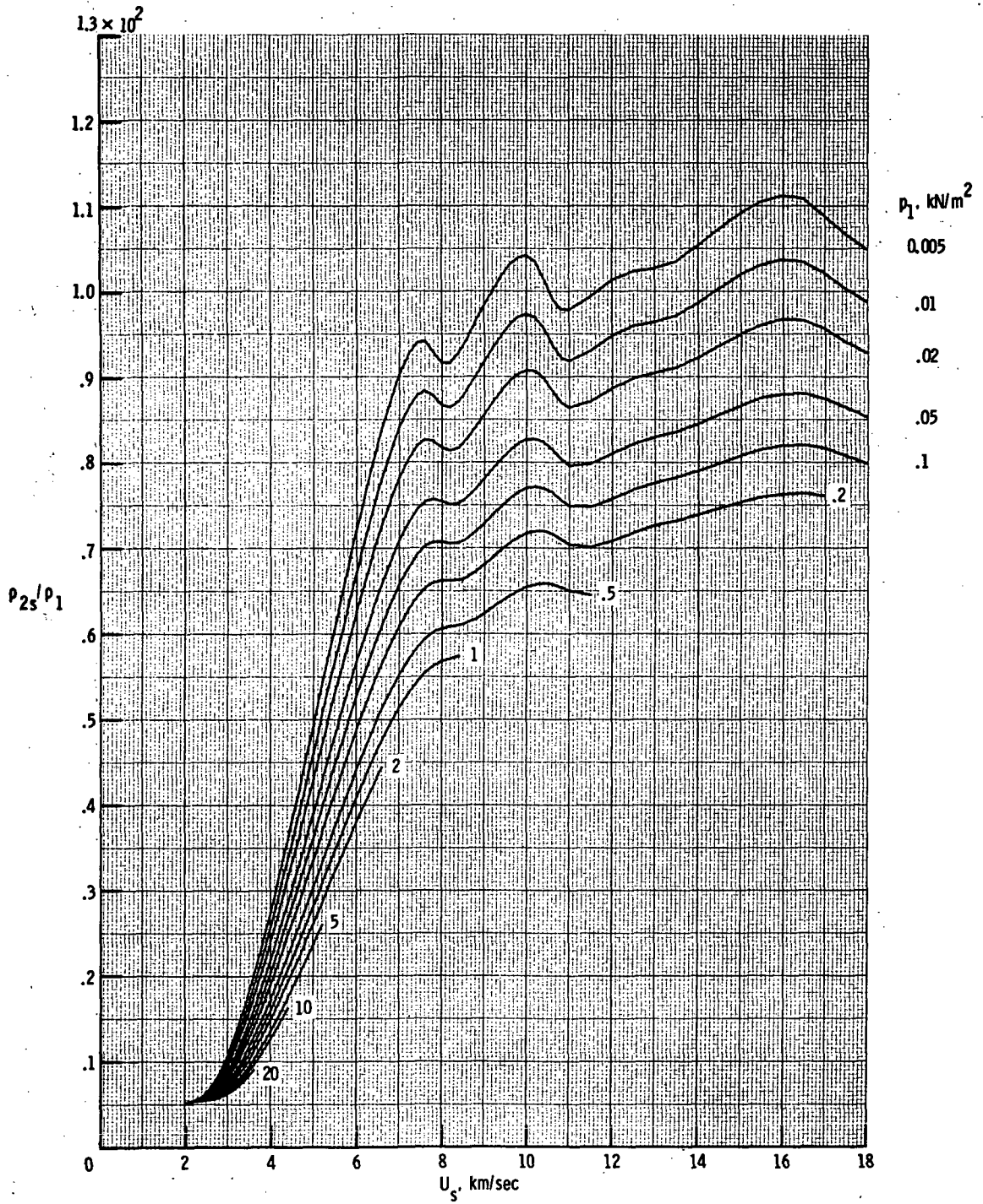
(c) Density \rho_{2s}/\rho_1 .
