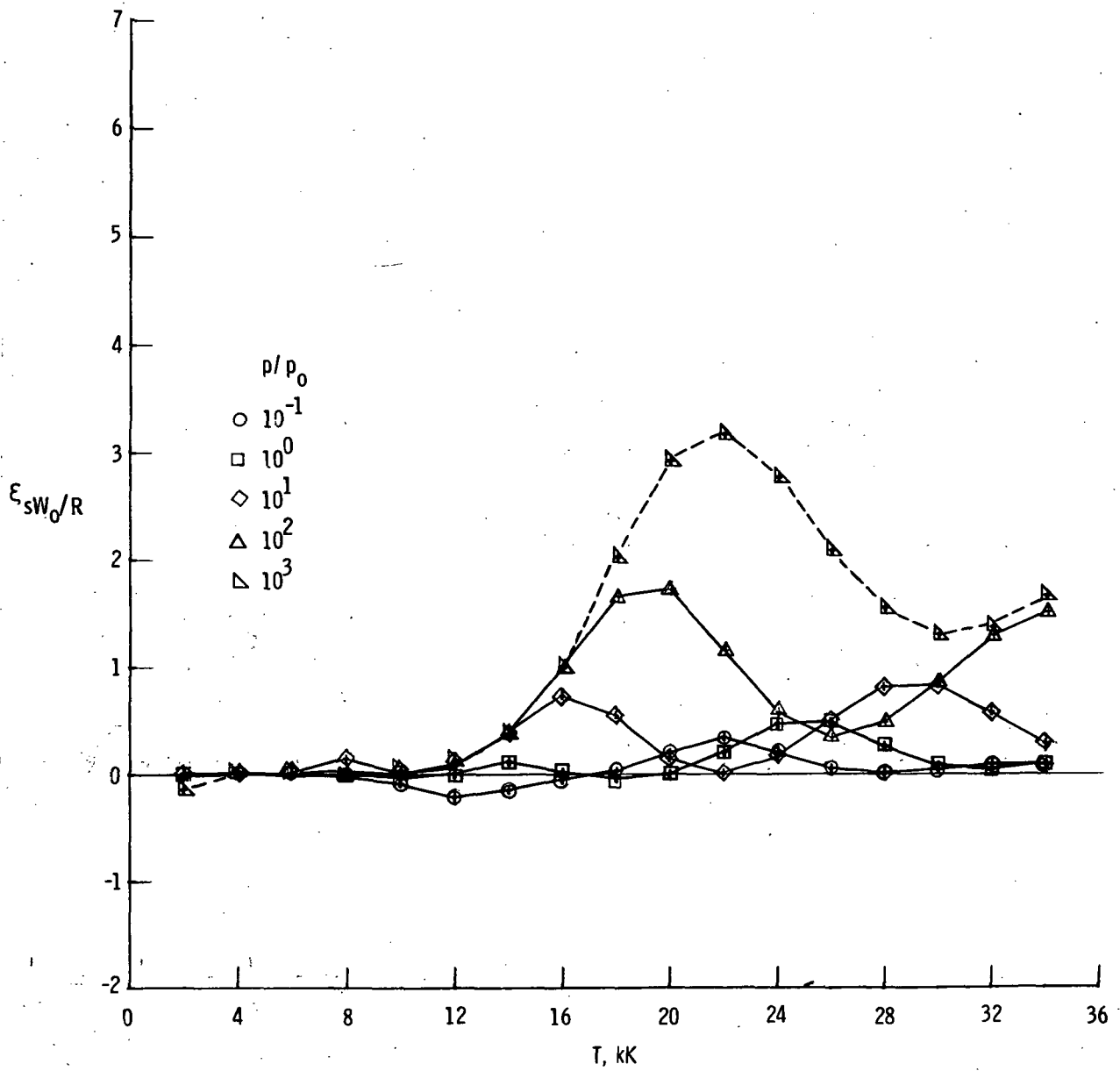
(b) Entropy s_{w_0}/R .
