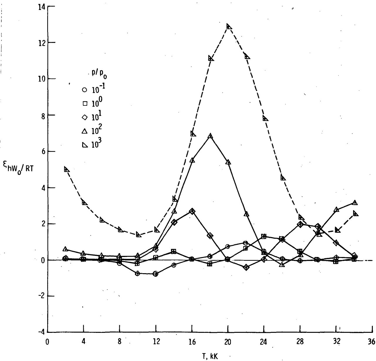
(c) Enthalpy hW_0/RT .
