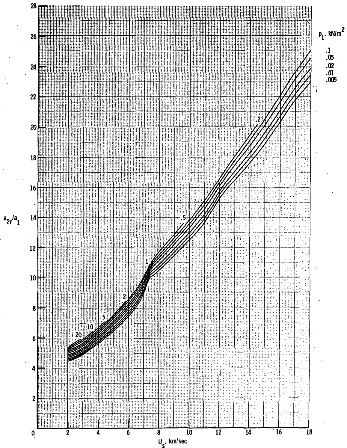
(e) Speed of sound a_{2r}/a_1 .
