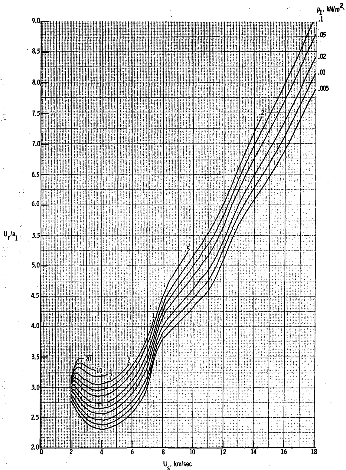
(i) Reflected shock velocity U_r/a_1 .
