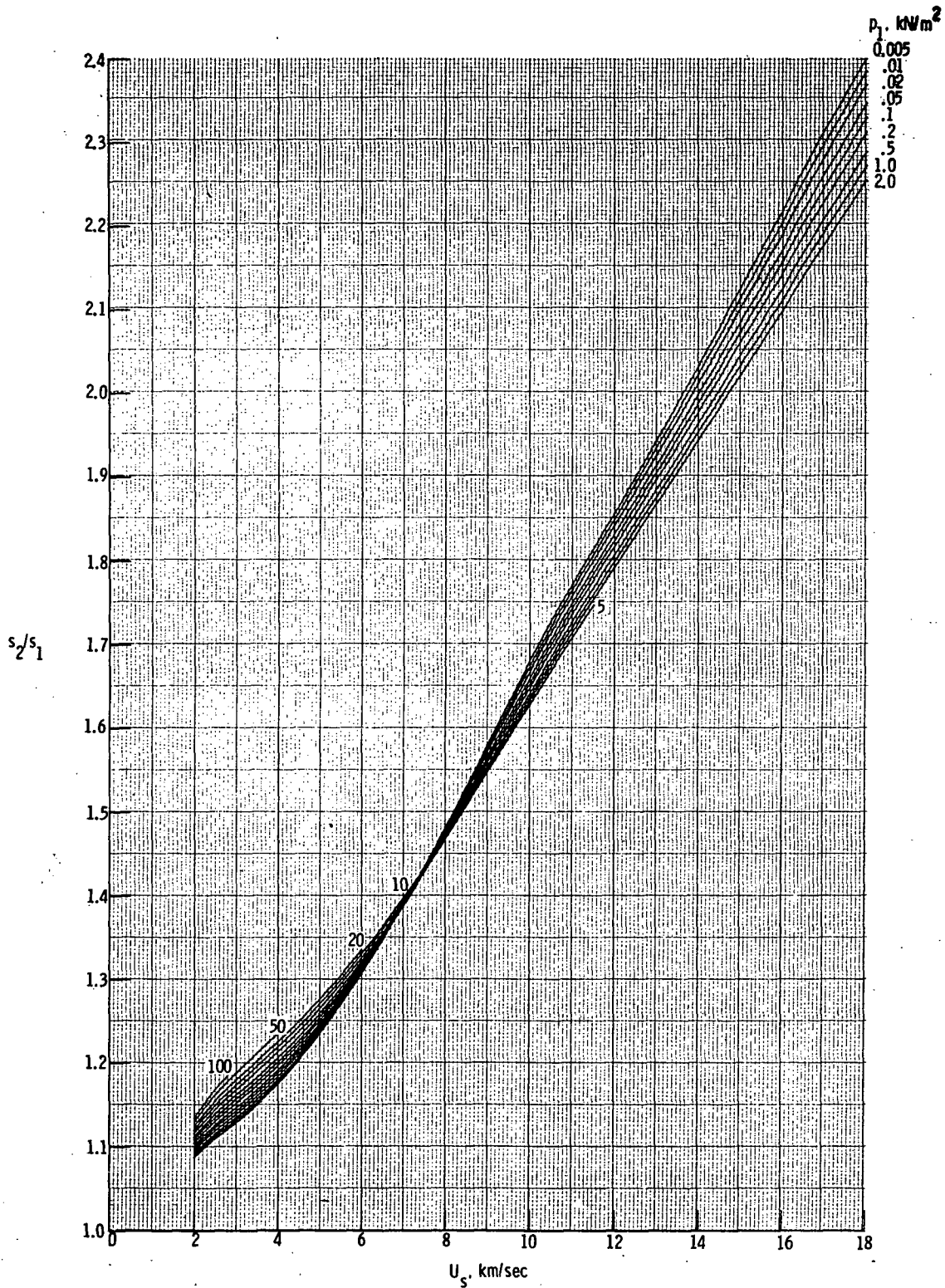
(f) Entropy s_2/s_1 .
