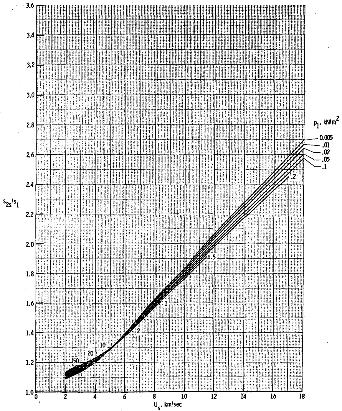
(f) Entropy s_{2s}/s_1 .
