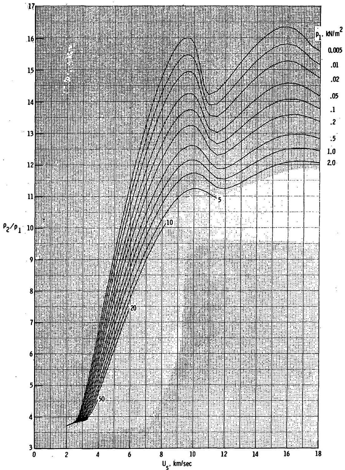
(c) Density \rho_2/\rho_1 .
