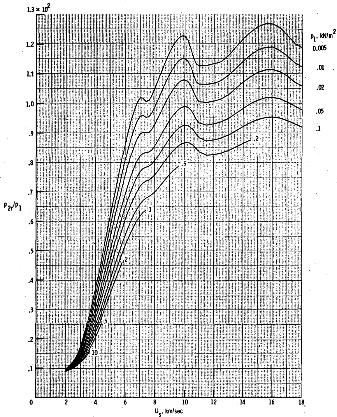
(c) Density \rho_{2r}/\rho_1 . Figure 4.- Continued.
