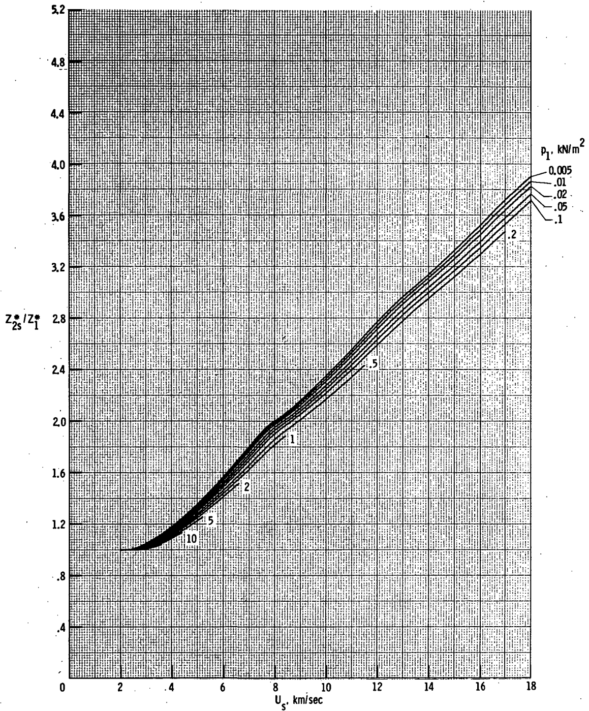
(g) Molecular-weight ratio Z_{2s}^*/Z_1^* .
