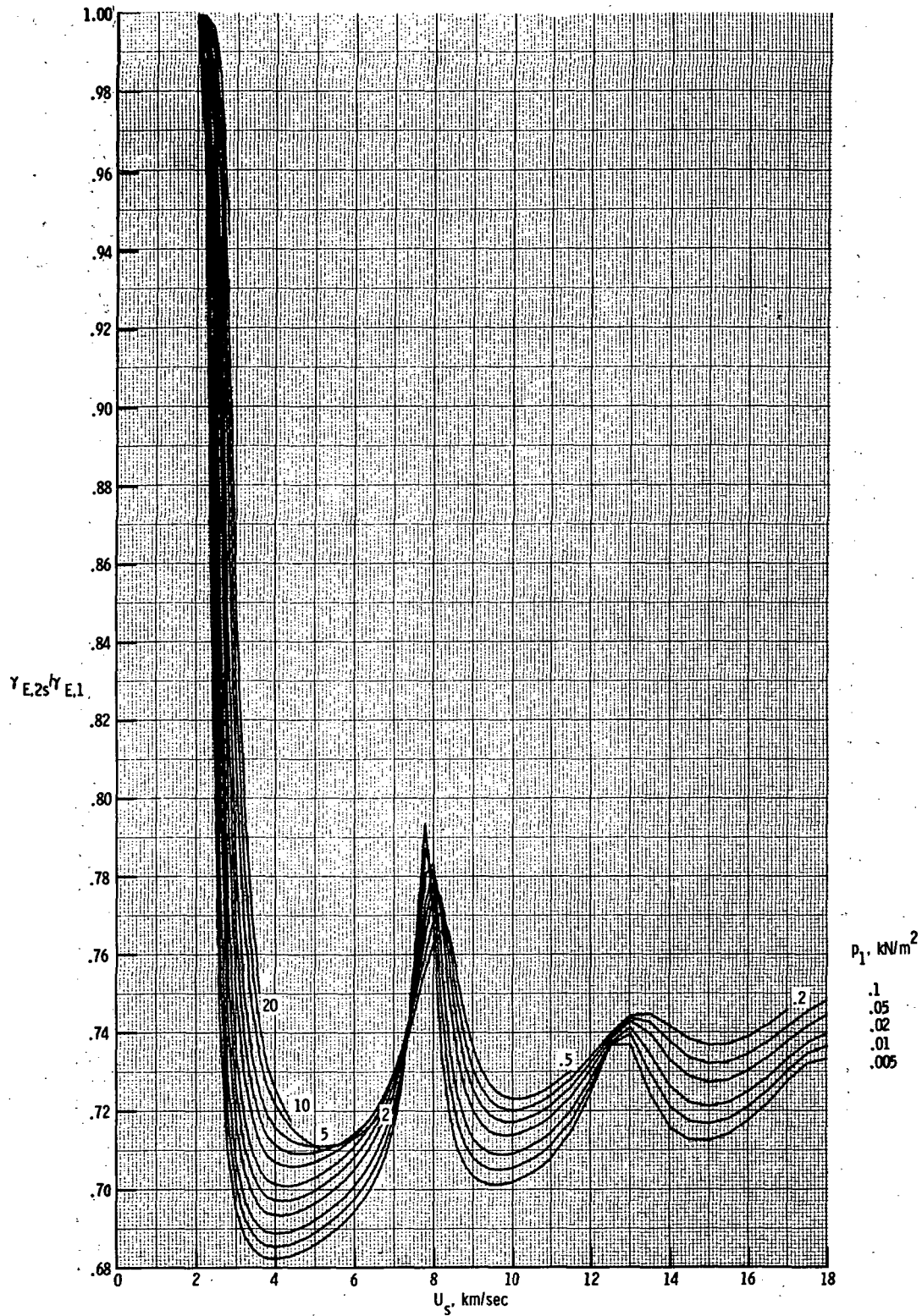
(h) Isentropic exponent \gamma_{E,2s}/\gamma_{E,1}
