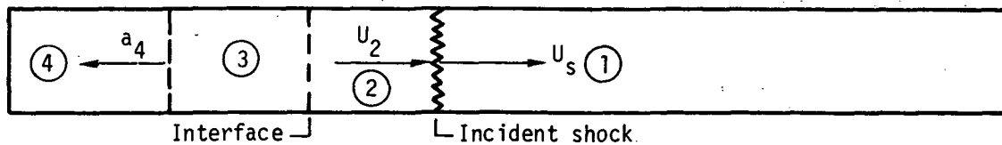
(b) Incident (moving) normal shock in test gas.
