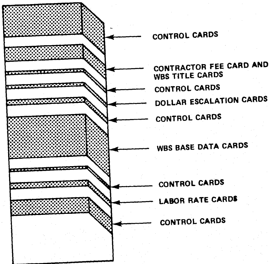
Figure 3. Run deck setup.
