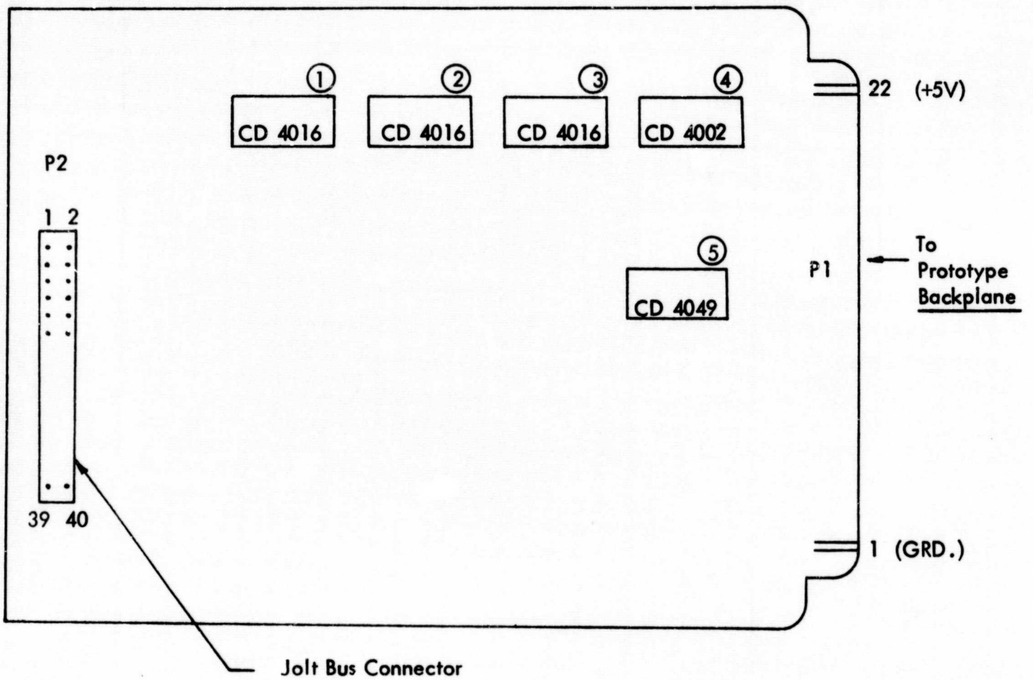
Figure 2. Jolt-to-Prototype Interface Board Component Side.
