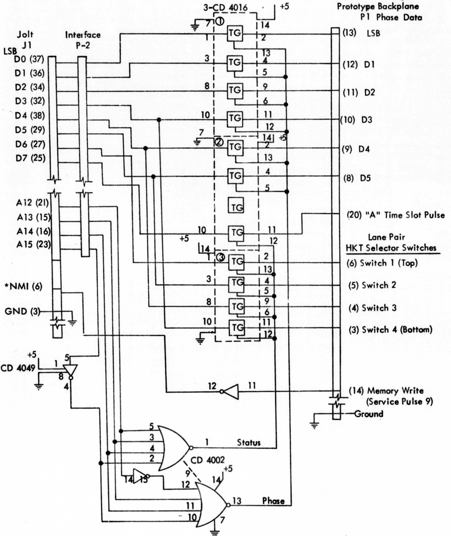
Figure 1. JOLT(TM) Interface to NASA Prototype Receivers.
